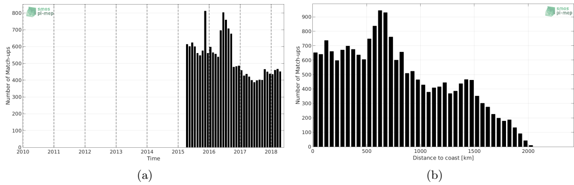
Figure 1: Number of match-ups between Argo and SMAP-L3-JPL-V4-MONTHLY-60KM SSS as a function of time (a) and as function of the distance to coast (b) over the Amazon and Orinoco river plumes Pi-MEP region and for the full satellite product period.
