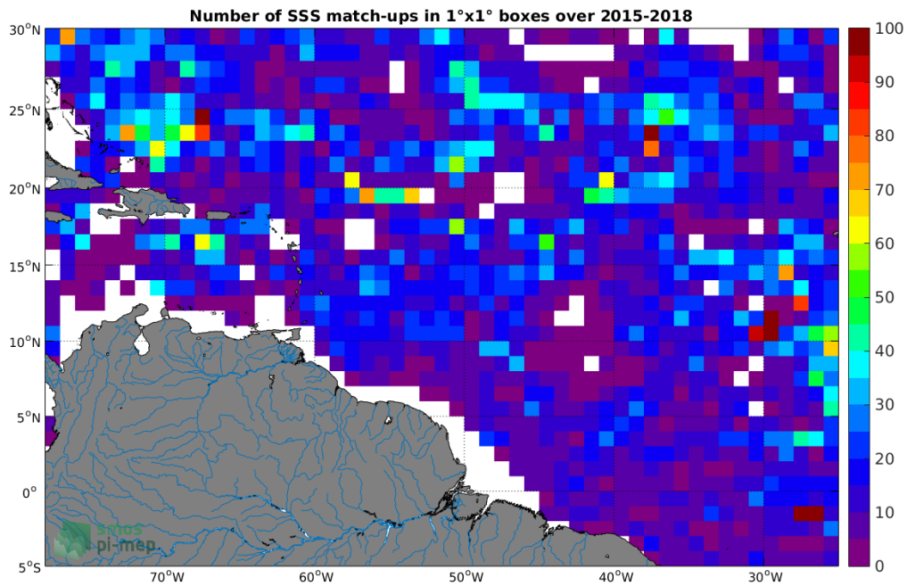
Figure 4: Number of SSS match-ups between Argo SSS and the SMAP-L3-JPL-V4-MONTHLY-60KM SSS product for the Amazon and Orinoco river plumes Pi-MEP region over 1^\circ \times 1^\circ boxes and for the full satellite product period.
