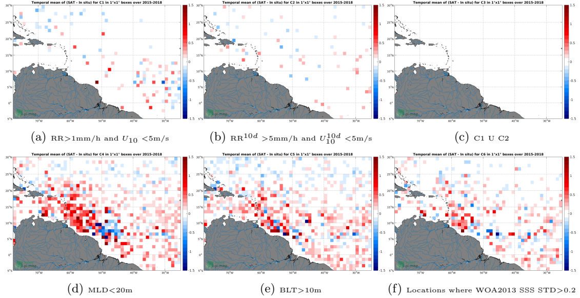
Figure 12: Temporal mean gridded over spatial boxes of size 1^\circ \times 1^\circ of \Delta\text{SSS} (SMAP-L3-JPL-V4-MONTHLY-60KM - Argo) for 6 different subdatasets corresponding to: \text{RR} > 1\text{mm/h} and U_{10} < 5\text{m/s} (a), \text{RR}^{10d} > 5\text{mm/h} and U_{10}^{10d} < 5\text{m/s} (b), C1 U C2 (c), \text{MLD} < 20\text{m} (d), \text{BLT} > 10\text{m} (e), Locations where WOA2013 SSS STD > 0.2 (f).
