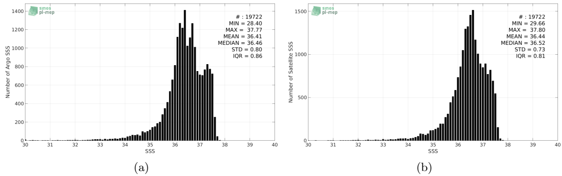
Figure 2: Histograms of SSS from Argo (a) and SMAP-L3-JPL-V4-MONTHLY-60KM (b) considering all match-up pairs per bins of 0.1 over the Amazon and Orinoco river plumes Pi-MEP region and for the full satellite product period.
