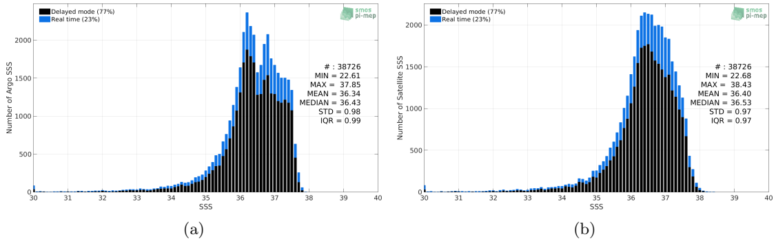
Figure 2: Histograms of SSS from Argo (a) and SMAP SSS L2-AVERAGED v5.0 (JPL) (b) considering all match-up pairs per bins of 0.1 over the Amazon and Orinoco river plumes Pi-MEP region and for the full satellite product period.
