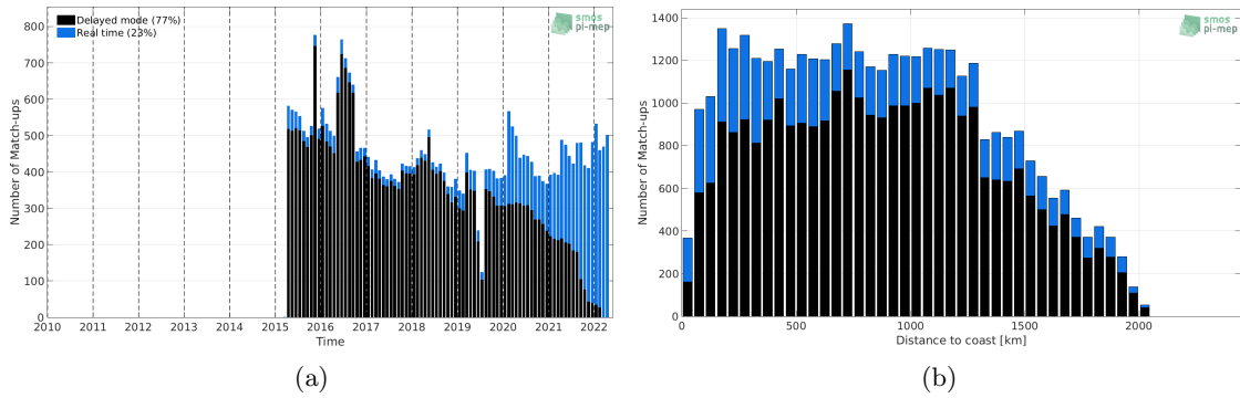
Figure 1: Number of match-ups between Argo and SMAP SSS L2-AVERAGED v5.0 (JPL) SSS as a function of time (a) and as function of the distance to coast (b) over the Amazon and Orinoco river plumes Pi-MEP region and for the full satellite product period.
