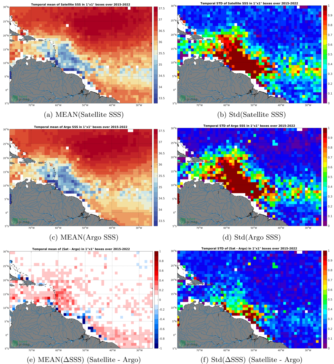
Figure 6: Temporal mean (left) and Std (right) of SSS from SMAP SSS L2-AVERAGED v5.0 (JPL) (top), Argo (middle), and of \Delta SSS (Satellite - Argo). Only match-up pairs are used to generate these maps.
