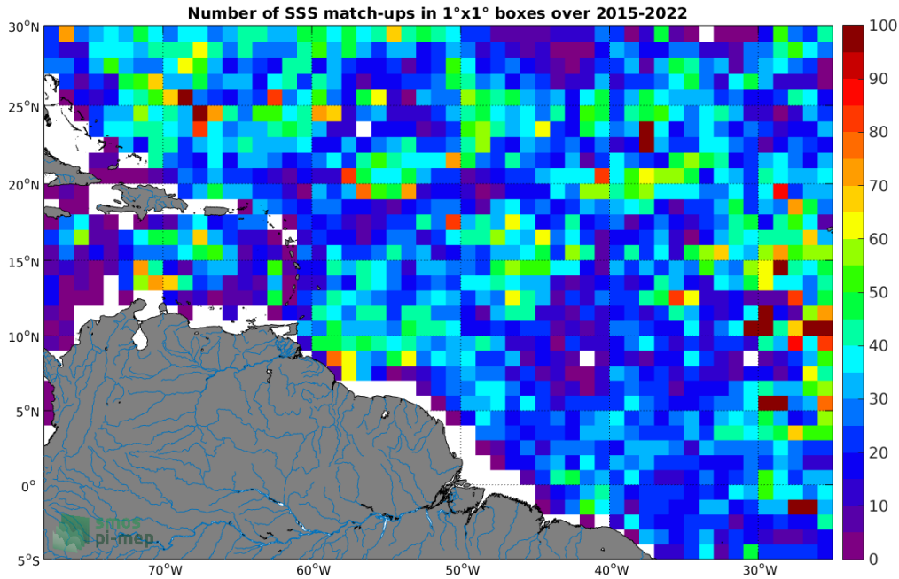
Figure 4: Number of SSS match-ups between Argo SSS and the SMAP SSS L2-AVERAGED v5.0 (JPL) SSS product for the Amazon and Orinoco river plumes Pi-MEP region over 1^\circ \times 1^\circ boxes and for the full satellite product period.
