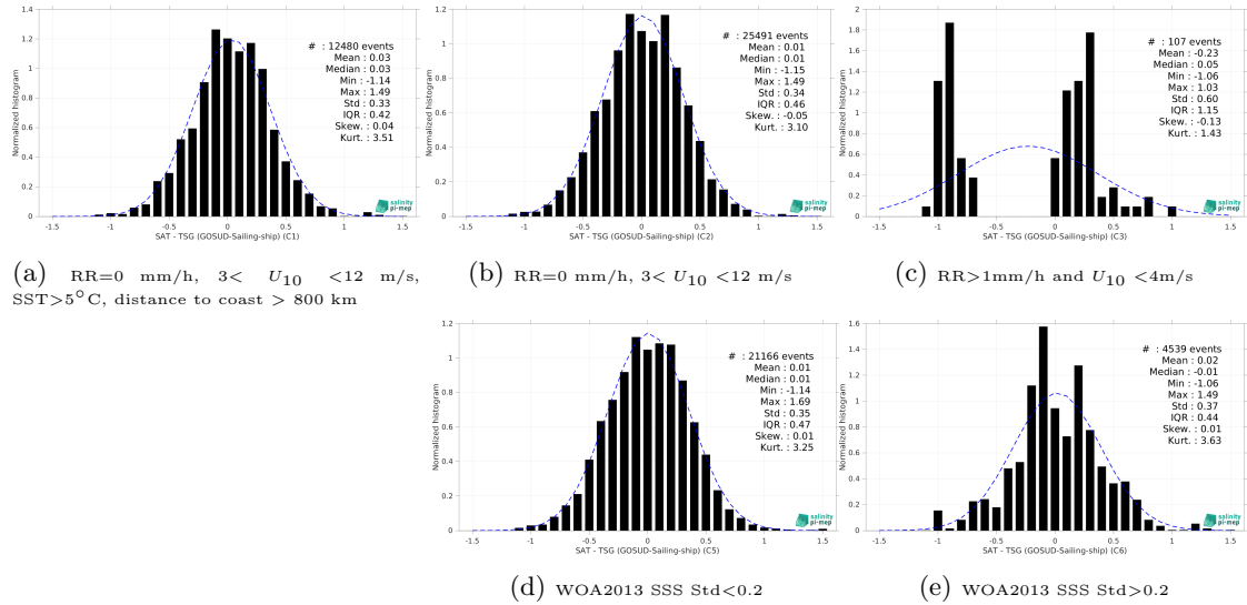
Figure 15: Normalized histogram of \Delta SSS (SMAP SSS L2 v6 (RSS) - TSG (GOSUD-Sailing-ship)) for 5 different subdatasets corresponding to: RR=0 mm/h, 3 < U_{10} < 12 m/s, SST>5°C, distance to coast > 800 km (a), RR=0 mm/h, 3 < U_{10} < 12 m/s (b), RR>1mm/h and U_{10} < 4 m/s (c), WOA2013 SSS Std<0.2 (d), WOA2013 SSS Std>0.2 (e).
