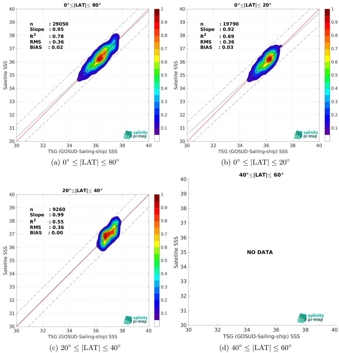
Figure 10: Contour maps of the concentration of SMAP SSS L2 v6 (RSS) SSS (y-axis) versus TSG (GOSUD-Sailing-ship) SSS (x-axis) at match-up pairs for different latitude bands. For each plot, the red line shows x=y . The black thin and dashed lines indicate a linear fit through the data cloud and the \pm 95\% confidence levels, respectively. The number match-up pairs n , the slope and R^2 coefficient of the linear fit, the root mean square (RMS) and the mean bias between satellite and in situ data are indicated for each latitude band in each plots.
