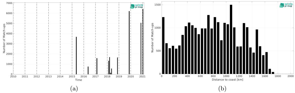
Figure 2: Number of match-ups between TSG (GOSUD-Sailing-ship) and SMAP SSS L2 v6 (RSS) SSS as a function of time (a) and as function of the distance to coast (b) over the Amazon and Orinoco river plumes Pi-MEP region and for the full satellite product period.
