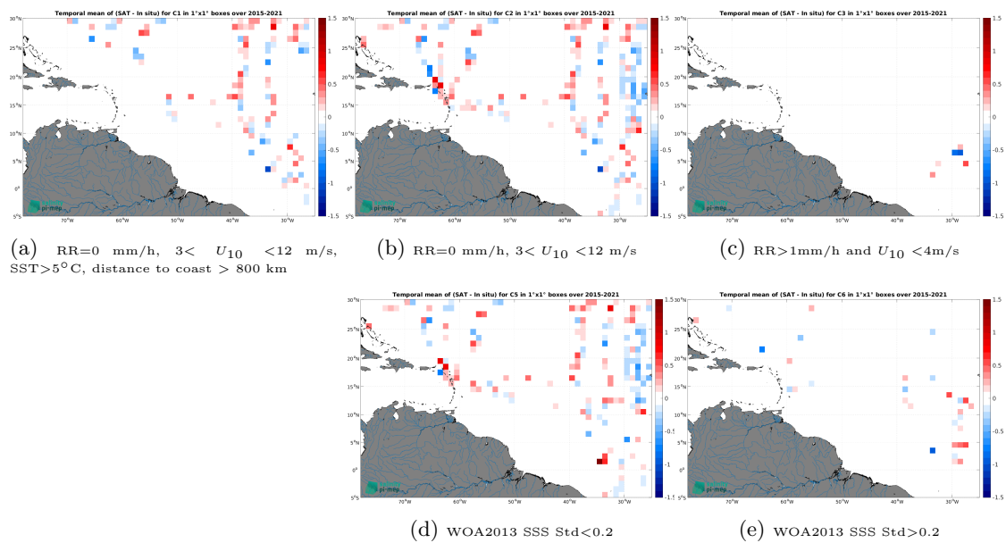
Figure 14: Temporal mean gridded over spatial boxes of size 1^\circ \times 1^\circ of \Delta SSS (SMAP SSS L2 v6 (RSS) - TSG (GOSUD-Sailing-ship)) for 5 different subdatasets corresponding to:RR=0 mm/h, 3 < U_{10} < 12 m/s, SST >5^\circ C, distance to coast > 800 km (a), RR=0 mm/h, 3 < U_{10} < 12 m/s (b), RR >1 mm/h and U_{10} < 4 m/s (c), WOA2013 SSS Std <0.2 (d), WOA2013 SSS Std >0.2 (e).
