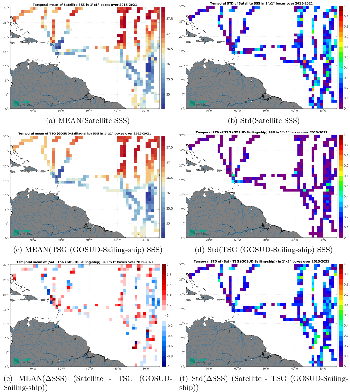
Figure 7: Temporal mean (left) and Std (right) of SSS from SMAP SSS L2 v6 (RSS) (top), TSG (GOSUD-Sailing-ship) (middle), and of \Delta SSS (Satellite - TSG (GOSUD-Sailing-ship)). Only match-up pairs are used to generate these maps.
