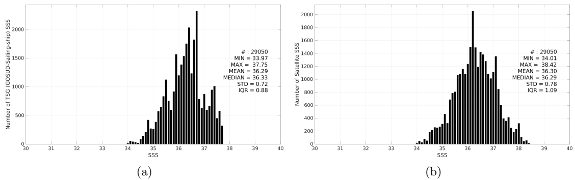
Figure 3: Histograms of SSS from TSG (GOSUD-Sailing-ship) (a) and SMAP SSS L2 v6 (RSS) (b) considering all match-up pairs per bins of 0.1 over the Amazon and Orinoco river plumes Pi-MEP region and for the full satellite product period.
