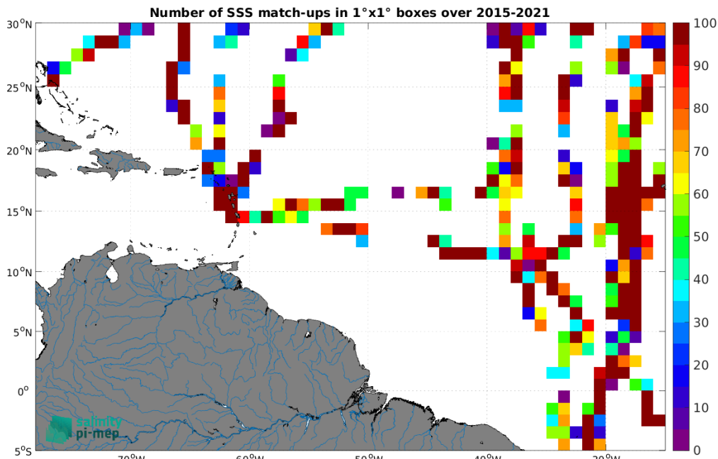
Figure 5: Number of SSS match-ups between TSG (GOSUD-Sailing-ship) SSS and the SMAP SSS L2 v6 (RSS) SSS product for the Amazon and Orinoco river plumes Pi-MEP region over 1^\circ \times 1^\circ boxes and for the full satellite product period.
