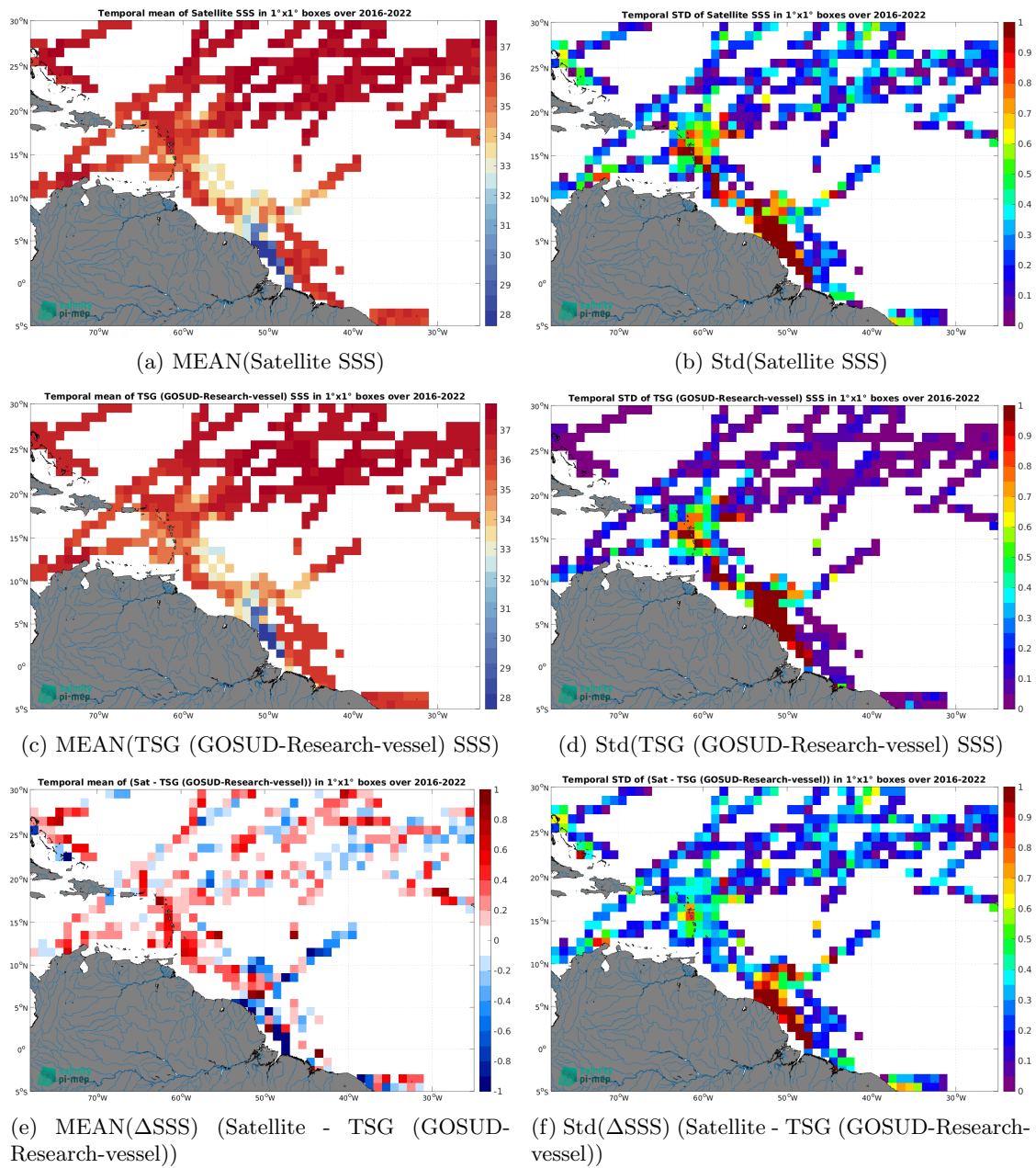
Figure 7: Temporal mean (left) and Std (right) of SSS from SMAP SSS L2 v6 (RSS) (top), TSG (GOSUD-Research-vessel) (middle), and of \Delta SSS (Satellite - TSG (GOSUD-Research-vessel)). Only match-up pairs are used to generate these maps.
