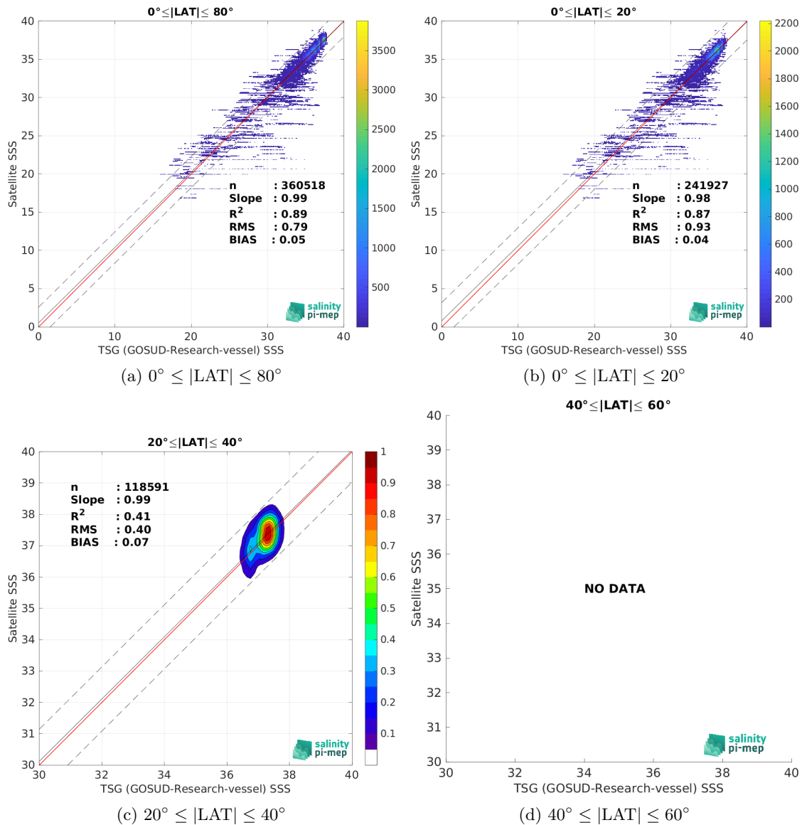
Figure 10: Contour maps of the concentration of SMAP SSS L2 v6 (RSS) SSS (y-axis) versus TSG (GOSUD-Research-vessel) SSS (x-axis) at match-up pairs for different latitude bands. For each plot, the red line shows x=y . The black thin and dashed lines indicate a linear fit through the data cloud and the \pm 95\% confidence levels, respectively. The number match-up pairs n , the slope and R^2 coefficient of the linear fit, the root mean square (RMS) and the mean bias between satellite and in situ data are indicated for each latitude band in each plot.
