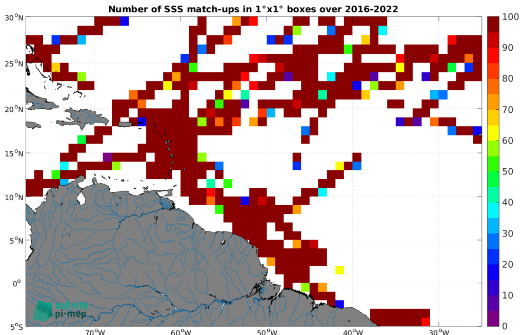
Figure 5: Number of SSS match-ups between TSG (GOSUD-Research-vessel) SSS and the SMAP SSS L2 v6 (RSS) SSS product for the Amazon and Orinoco river plumes Pi-MEP region over 1^\circ \times 1^\circ boxes and for the full satellite product period.
