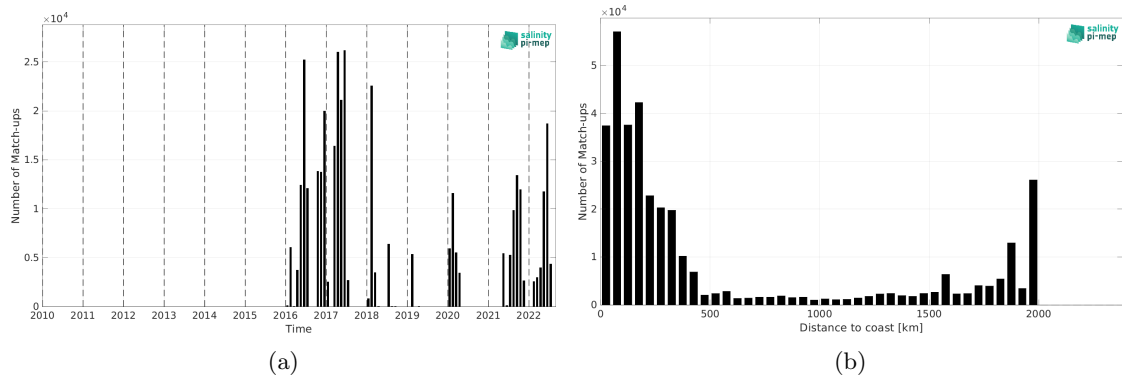
Figure 2: Number of match-ups between TSG (GOSUD-Research-vessel) and SMAP SSS L2 v6 (RSS) SSS as a function of time (a) and as function of the distance to coast (b) over the Amazon and Orinoco river plumes Pi-MEP region and for the full satellite product period.
