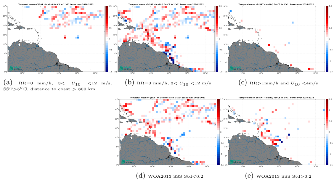
Figure 14: Temporal mean gridded over spatial boxes of size 1^\circ \times 1^\circ of \Delta SSS (SMAP SSS L2 v6 (RSS) - TSG (GOSUD-Research-vessel)) for 5 different subdatasets corresponding to: RR=0 mm/h, 3 < U_{10} < 12 m/s, SST > 5°C, distance to coast > 800 km (a), RR=0 mm/h, 3 < U_{10} < 12 m/s (b), RR > 1mm/h and U_{10} < 4 m/s (c), WOA2013 SSS Std < 0.2 (d), WOA2013 SSS Std > 0.2 (e).
