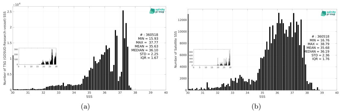
Figure 3: Histograms of SSS from TSG (GOSUD-Research-vessel) (a) and SMAP SSS L2 v6 (RSS) (b) considering all match-up pairs per bins of 0.1 over the Amazon and Orinoco river plumes Pi-MEP region and for the full satellite product period.
