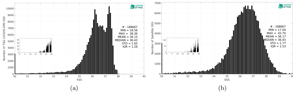
Figure 3: Histograms of SSS from TSG (LEGOS-DM) (a) and SMAP SSS L2 v6 - 40 km (RSS) (b) considering all match-up pairs per bins of 0.1 over the Amazon and Orinoco river plumes Pi-MEP region and for the full satellite product period.
