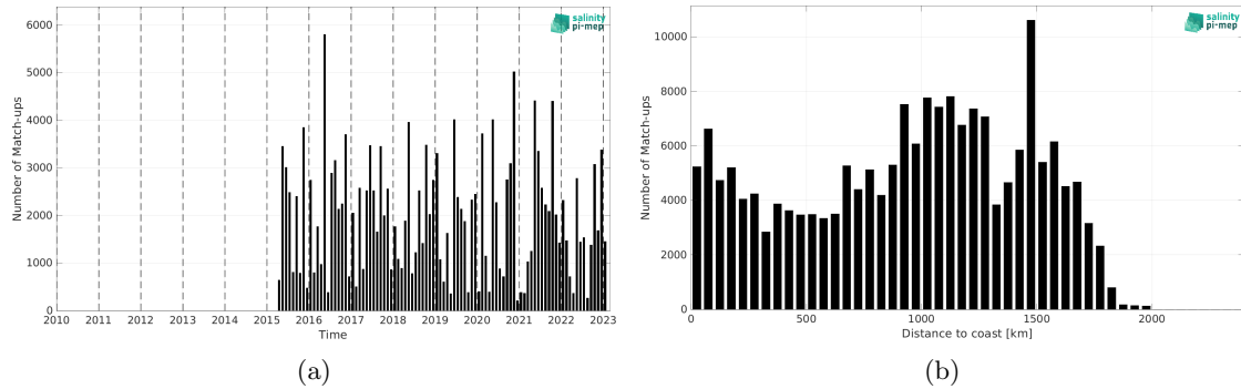
Figure 2: Number of match-ups between TSG (LEGOS-DM) and SMAP SSS L2 v6 - 40 km (RSS) SSS as a function of time (a) and as function of the distance to coast (b) over the Amazon and Orinoco river plumes Pi-MEP region and for the full satellite product period.
