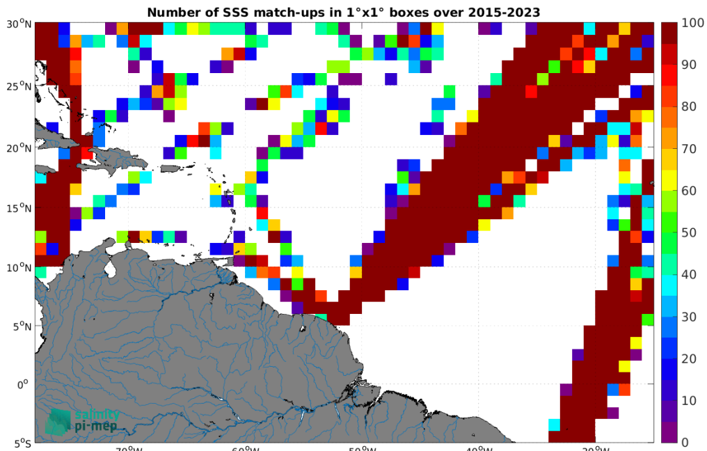
Figure 5: Number of SSS match-ups between TSG (LEGOS-DM) SSS and the SMAP SSS L2 v6 - 40 km (RSS) SSS product for the Amazon and Orinoco river plumes Pi-MEP region over 1^\circ \times 1^\circ boxes and for the full satellite product period.
