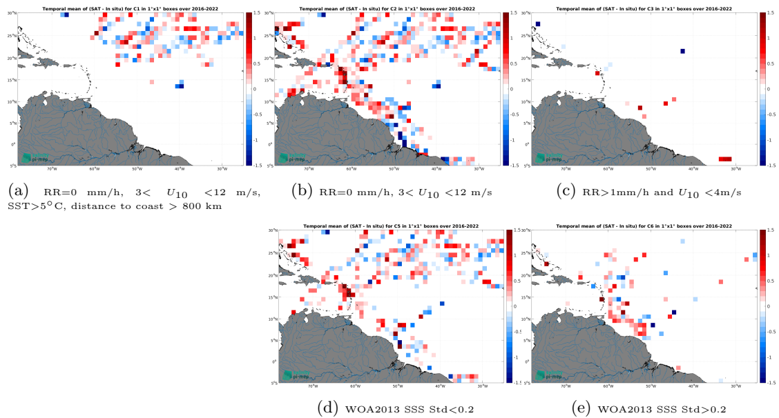
Figure 14: Temporal mean gridded over spatial boxes of size 1^\circ \times 1^\circ of \Delta SSS (SMAP SSS L2 v6 - 40 km (RSS) - TSG (GOSUD-Research-vessel)) for 5 different subdatasets corresponding to:RR=0 mm/h, 3 < U_{10} < 12 m/s, SST>5°C, distance to coast > 800 km (a), RR=0 mm/h, 3 < U_{10} < 12 m/s (b), RR>1mm/h and U_{10} < 4 m/s (c), WOA2013 SSS Std<0.2 (d), WOA2013 SSS Std>0.2 (e).
