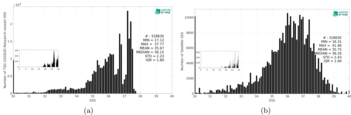
Figure 3: Histograms of SSS from TSG (GOSUD-Research-vessel) (a) and SMAP SSS L2 v6 - 40 km (RSS) (b) considering all match-up pairs per bins of 0.1 over the Amazon and Orinoco river plumes Pi-MEP region and for the full satellite product period.
