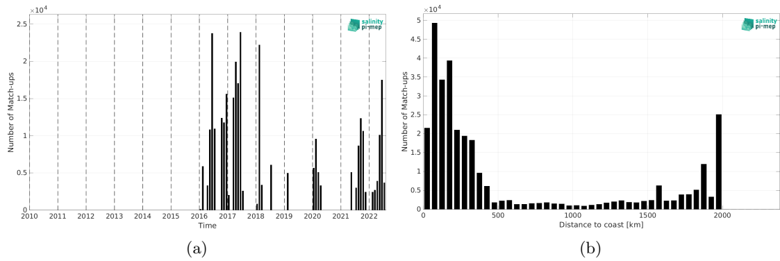
Figure 2: Number of match-ups between TSG (GOSUD-Research-vessel) and SMAP SSS L2 v6 - 40 km (RSS) SSS as a function of time (a) and as function of the distance to coast (b) over the Amazon and Orinoco river plumes Pi-MEP region and for the full satellite product period.
