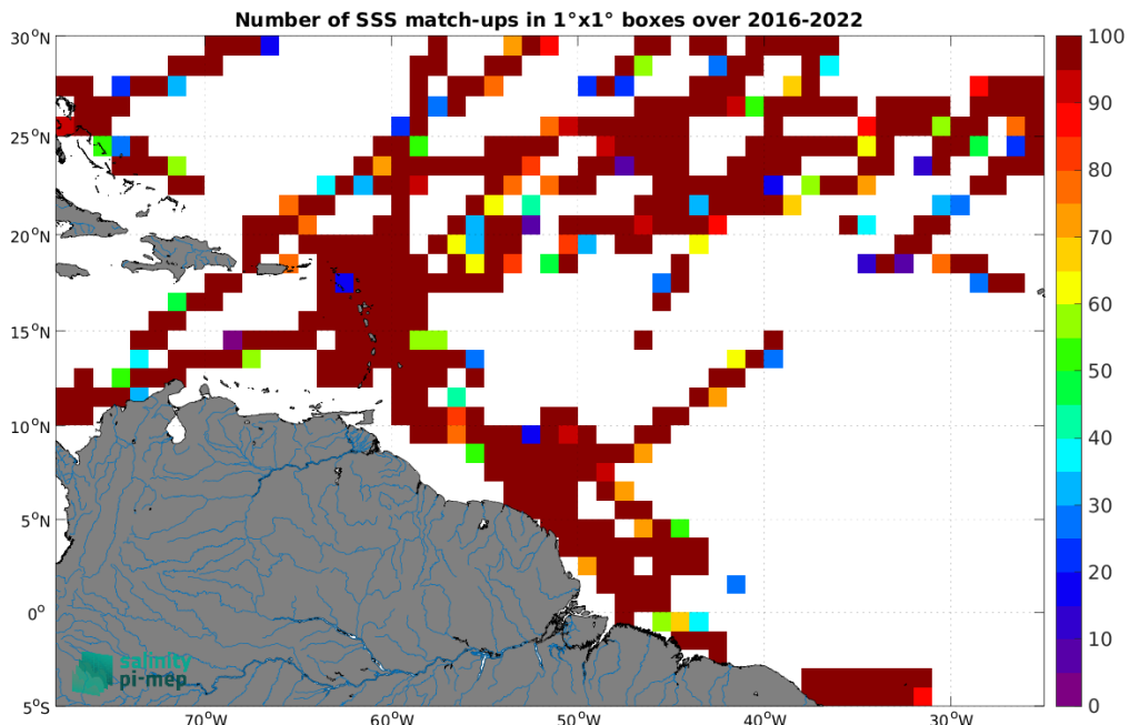
Figure 5: Number of SSS match-ups between TSG (GOSUD-Research-vessel) SSS and the SMAP SSS L2 v6 - 40 km (RSS) SSS product for the Amazon and Orinoco river plumes Pi-MEP region over 1°x1° boxes and for the full satellite product period.
