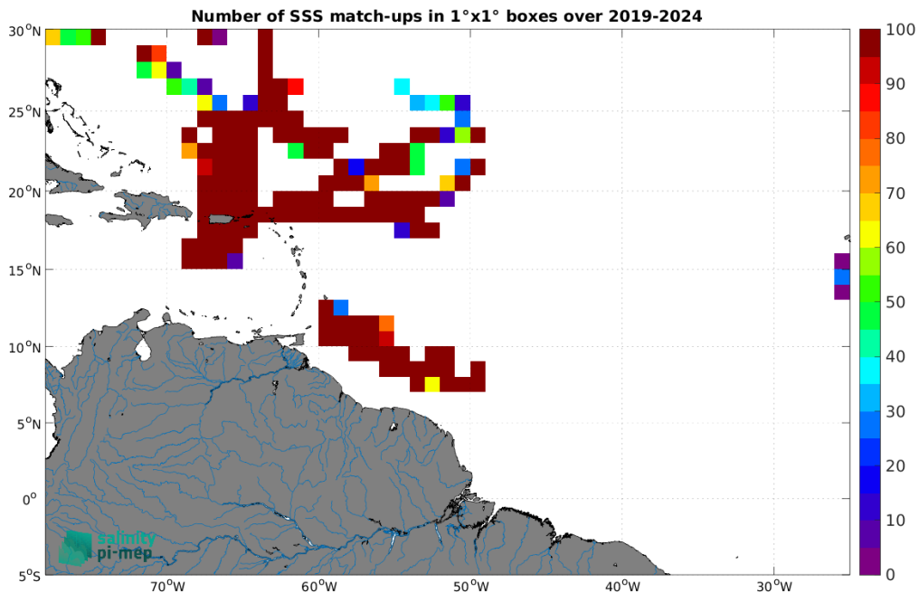
Figure 5: Number of SSS match-ups between Saildrone SSS and the SMAP SSS L2 v6 - 40 km (RSS) SSS product for the Amazon and Orinoco river plumes Pi-MEP region over 1^\circ \times 1^\circ boxes and for the full satellite product period.
