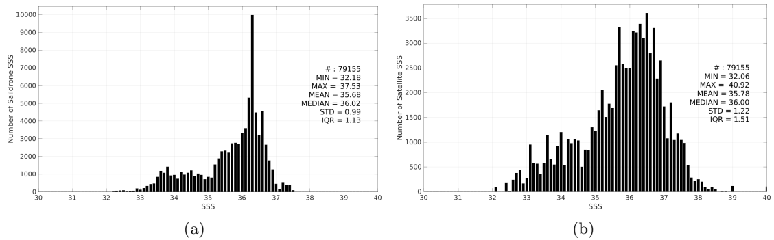
Figure 3: Histograms of SSS from Saildrone (a) and SMAP SSS L2 v6 - 40 km (RSS) (b) considering all match-up pairs per bins of 0.1 over the Amazon and Orinoco river plumes Pi-MEP region and for the full satellite product period.
