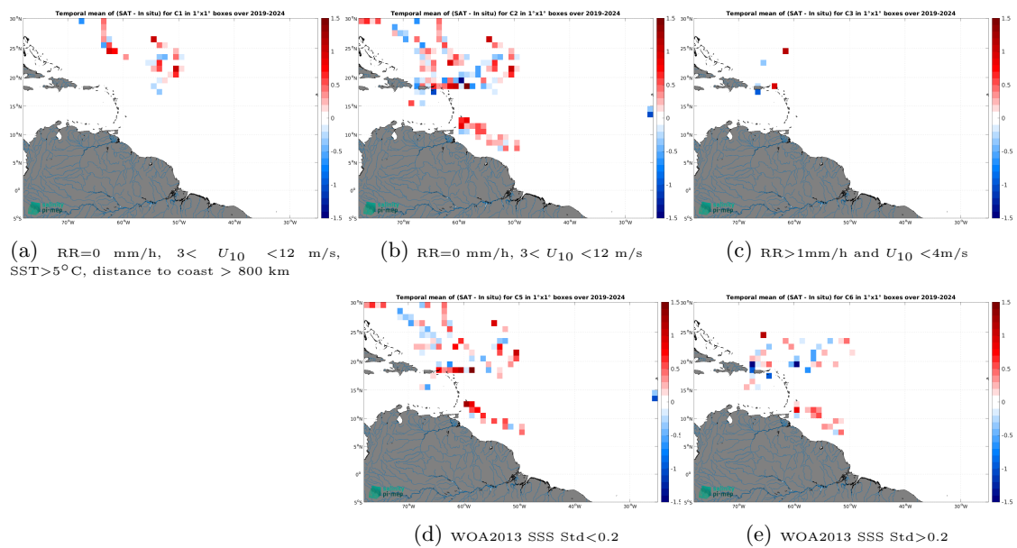
Figure 14: Temporal mean gridded over spatial boxes of size 1^\circ \times 1^\circ of \Delta SSS (SMAP SSS L2 v6 - 40 km (RSS) - Salldrone) for 5 different subdatasets corresponding to:RR=0 mm/h, 3 < U_{10} < 12 m/s, SST >5^\circ\text{C} , distance to coast > 800 km (a), RR=0 mm/h, 3 < U_{10} < 12 m/s (b), RR >1 mm/h and U_{10} < 4 m/s (c), WOA2013 SSS Std <0.2 (d), WOA2013 SSS Std >0.2 (e).
