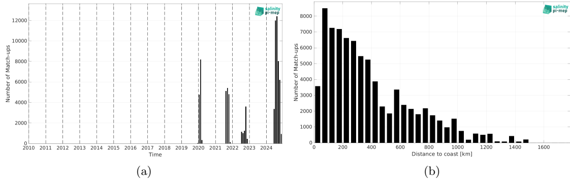
Figure 2: Number of match-ups between Saildrone and SMAP SSS L2 v6 - 40 km (RSS) SSS as a function of time (a) and as function of the distance to coast (b) over the Amazon and Orinoco river plumes Pi-MEP region and for the full satellite product period.
