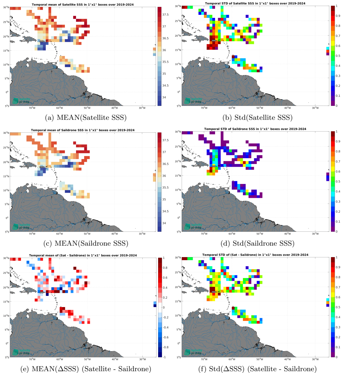
Figure 7: Temporal mean (left) and Std (right) of SSS from SMAP SSS L2 v6 - 40 km (RSS) (top), Saildrone (middle), and of \Delta SSS (Satellite - Saildrone). Only match-up pairs are used to generate these maps.
