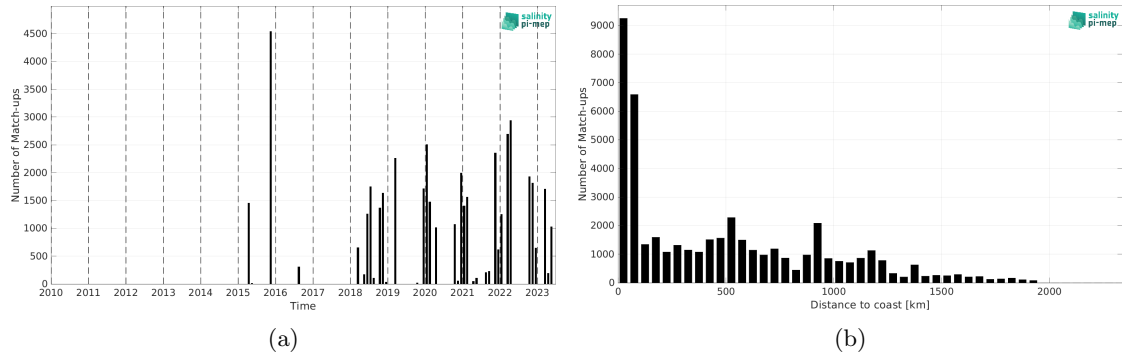
Figure 2: Number of match-ups between TSG (SAMOS) and SMAP SSS L2 v5.3 (RSS) SSS as a function of time (a) and as function of the distance to coast (b) over the Amazon and Orinoco river plumes Pi-MEP region and for the full satellite product period.
