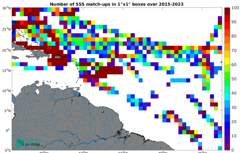
Figure 5: Number of SSS match-ups between TSG (SAMOS) SSS and the SMAP SSS L2 v5.3 (RSS) SSS product for the Amazon and Orinoco river plumes Pi-MEP region over 1^\circ \times 1^\circ boxes and for the full satellite product period.
