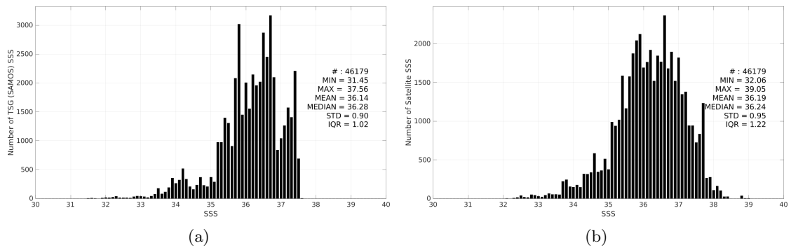
Figure 3: Histograms of SSS from TSG (SAMOS) (a) and SMAP SSS L2 v5.3 (RSS) (b) considering all match-up pairs per bins of 0.1 over the Amazon and Orinoco river plumes Pi-MEP region and for the full satellite product period.
