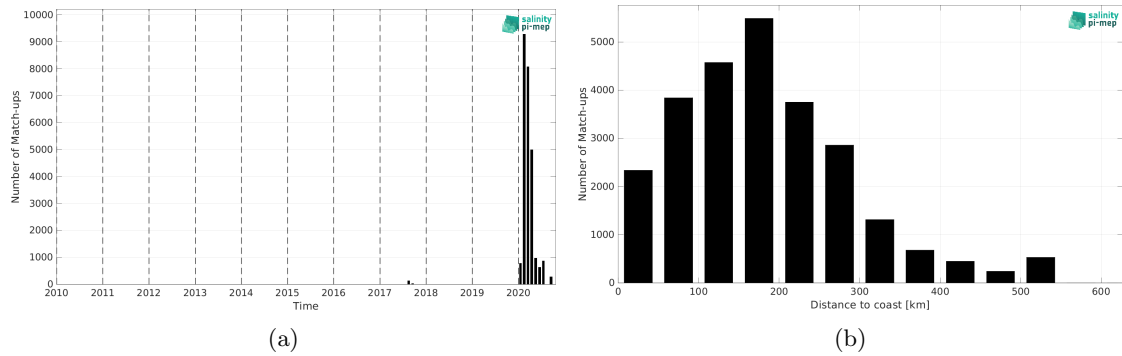
Figure 2: Number of match-ups between Surface drifters and SMAP SSS L2 v5.3 (RSS) SSS as a function of time (a) and as function of the distance to coast (b) over the Amazon and Orinoco river plumes Pi-MEP region and for the full satellite product period.
