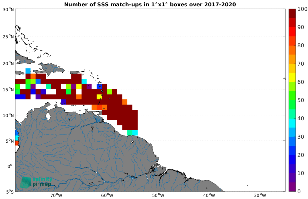
Figure 4: Number of SSS match-ups between Surface drifters SSS and the SMAP SSS L2 v5.3 (RSS) SSS product for the Amazon and Orinoco river plumes Pi-MEP region over 1^\circ \times 1^\circ boxes and for the full satellite product period.
