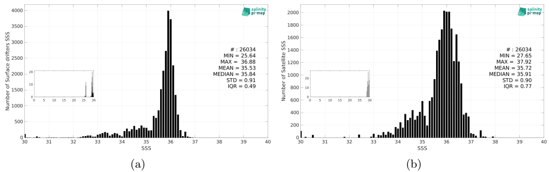
Figure 3: Histograms of SSS from Surface drifters (a) and SMAP SSS L2 v5.3 (RSS) (b) considering all match-up pairs per bins of 0.1 over the Amazon and Orinoco river plumes Pi-MEP region and for the full satellite product period.
