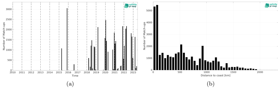
Figure 2: Number of match-ups between TSG (SAMOS) and SMAP SSS L2 v5.3 - 40 km (RSS) SSS as a function of time (a) and as function of the distance to coast (b) over the Amazon and Orinoco river plumes Pi-MEP region and for the full satellite product period.
