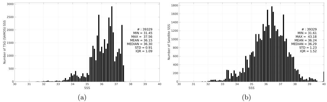
Figure 3: Histograms of SSS from TSG (SAMOS) (a) and SMAP SSS L2 v5.3 - 40 km (RSS) (b) considering all match-up pairs per bins of 0.1 over the Amazon and Orinoco river plumes Pi-MEP region and for the full satellite product period.
