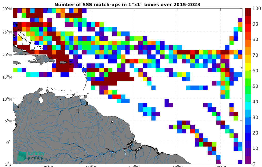
Figure 5: Number of SSS match-ups between TSG (SAMOS) SSS and the SMAP SSS L2 v5.3 - 40 km (RSS) SSS product for the Amazon and Orinoco river plumes Pi-MEP region over 1^\circ \times 1^\circ boxes and for the full satellite product period.
