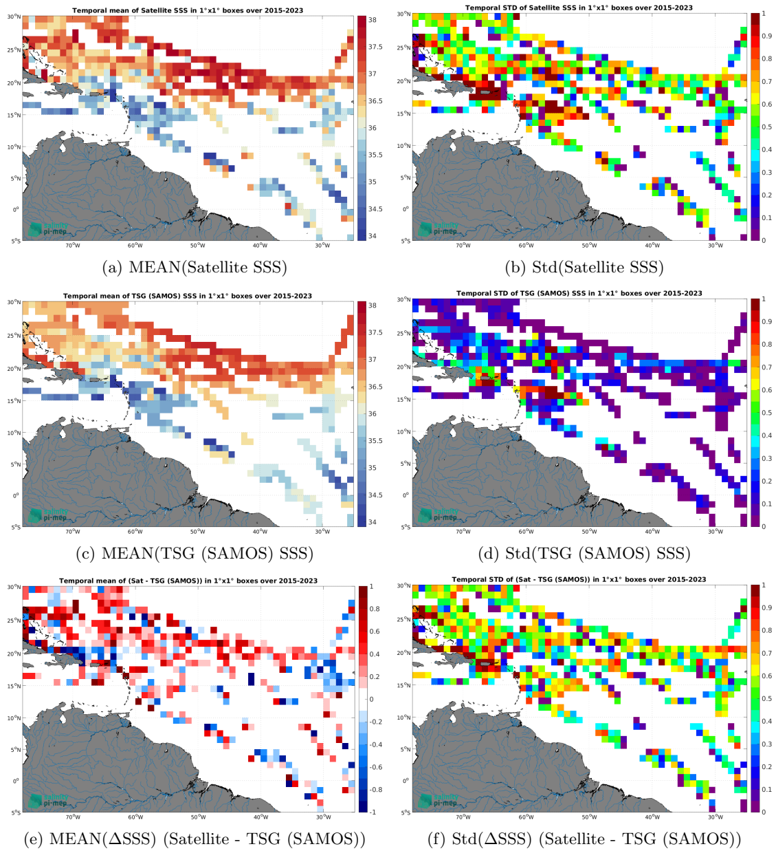
Figure 7: Temporal mean (left) and Std (right) of SSS from SMAP SSS L2 v5.3 - 40 km (RSS) (top), TSG (SAMOS) (middle), and of \Delta SSS (Satellite - TSG (SAMOS)). Only match-up pairs are used to generate these maps.
