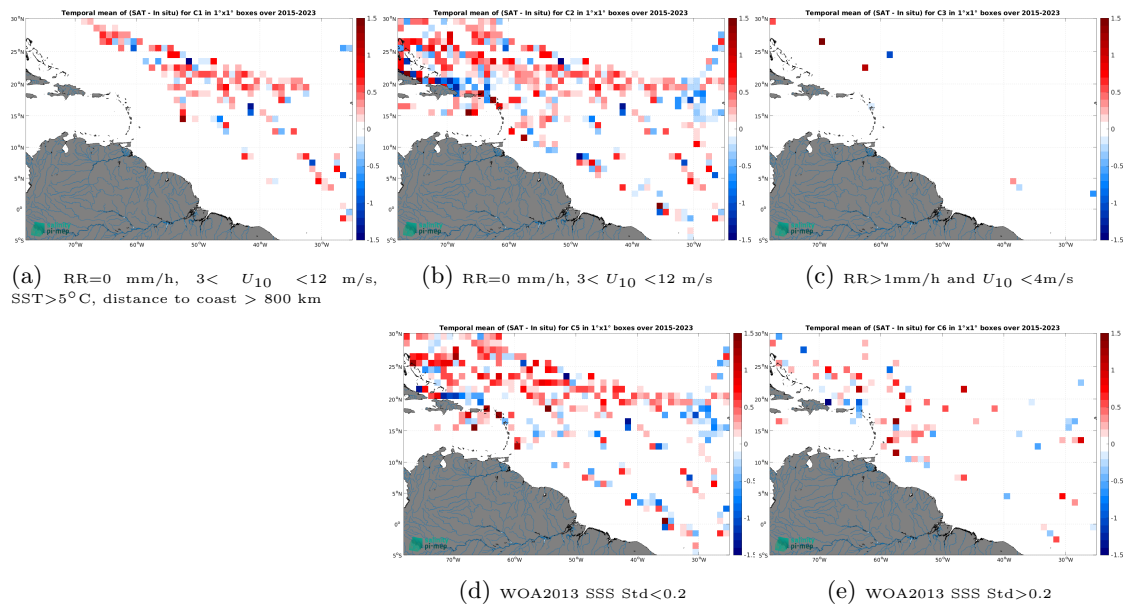
Figure 14: Temporal mean gridded over spatial boxes of size 1^\circ \times 1^\circ of \Delta SSS (SMAP SSS L2 v5.3 - 40 km (RSS) - TSG (SAMOS)) for 5 different subdatasets corresponding to: RR=0 mm/h, 3 < U_{10} < 12 m/s, SST > 5°C, distance to coast > 800 km (a), RR=0 mm/h, 3 < U_{10} < 12 m/s (b), RR > 1mm/h and U_{10} < 4 m/s (c), WOA2013 SSS Std < 0.2 (d), WOA2013 SSS Std > 0.2 (e).
