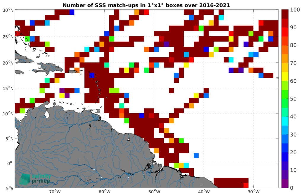
Figure 5: Number of SSS match-ups between TSG (GOSUD-Research-vessel) SSS and the SMAP SSS L2 v5.3 - 40 km (RSS) SSS product for the Amazon and Orinoco river plumes Pi-MEP region over 1^\circ \times 1^\circ boxes and for the full satellite product period.
