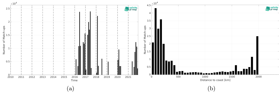
Figure 2: Number of match-ups between TSG (GOSUD-Research-vessel) and SMAP SSS L2 v5.3 - 40 km (RSS) SSS as a function of time (a) and as function of the distance to coast (b) over the Amazon and Orinoco river plumes Pi-MEP region and for the full satellite product period.
