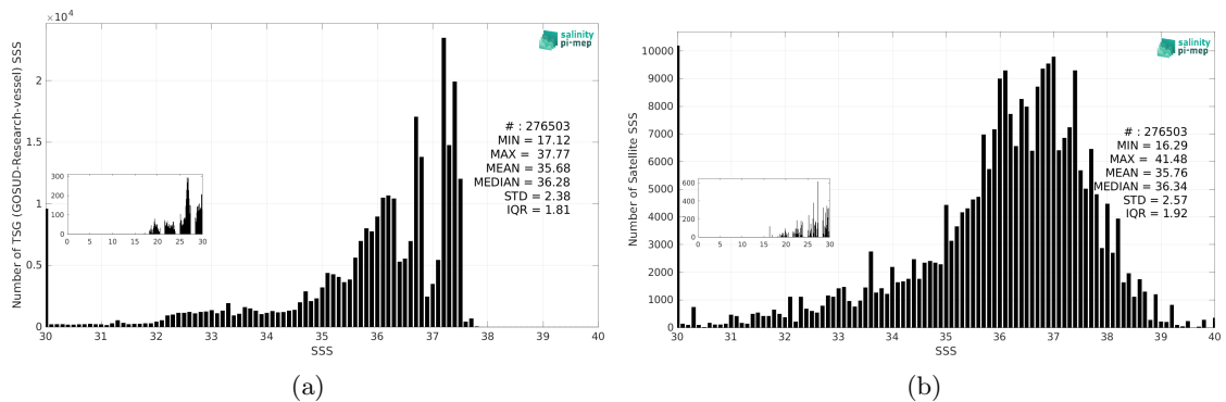
Figure 3: Histograms of SSS from TSG (GOSUD-Research-vessel) (a) and SMAP SSS L2 v5.3 - 40 km (RSS) (b) considering all match-up pairs per bins of 0.1 over the Amazon and Orinoco river plumes Pi-MEP region and for the full satellite product period.
