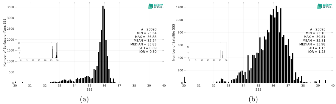
Figure 3: Histograms of SSS from Surface drifters (a) and SMAP SSS L2 v5.3 - 40 km (RSS) (b) considering all match-up pairs per bins of 0.1 over the Amazon and Orinoco river plumes Pi-MEP region and for the full satellite product period.
