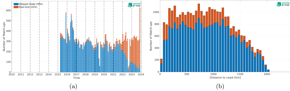
Figure 2: Number of match-ups between Argo and SMAP SSS L2 v5.3 - 40 km (RSS) SSS as a function of time (a) and as function of the distance to coast (b) over the Amazon and Orinoco river plumes Pi-MEP region and for the full satellite product period.
