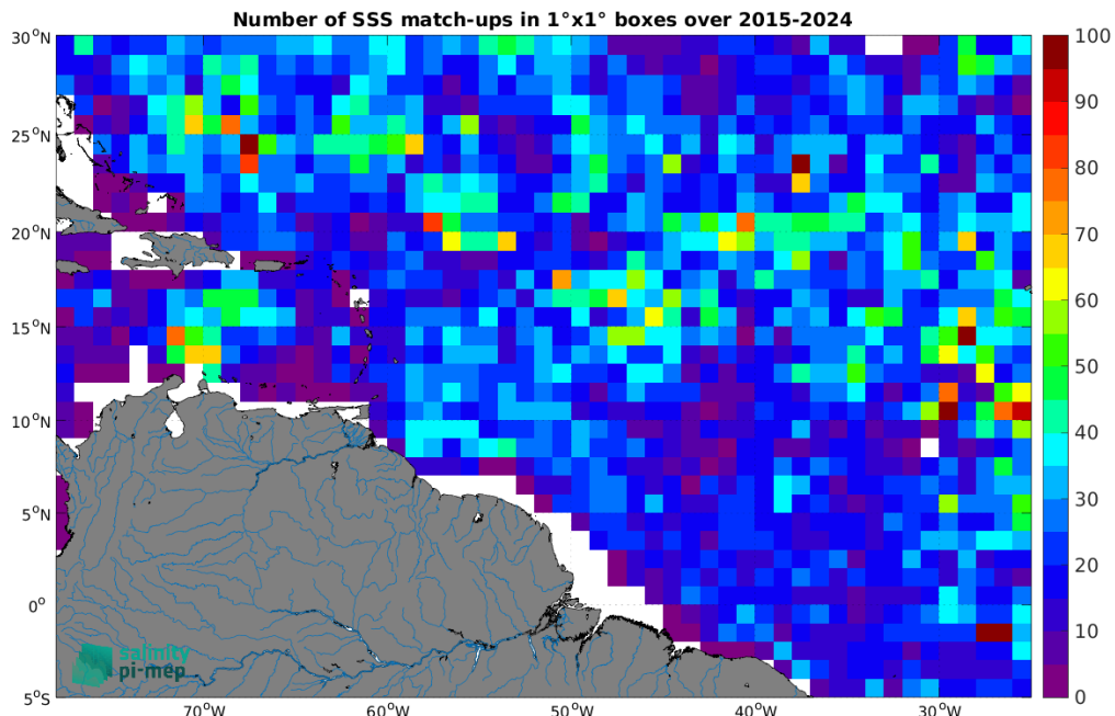
Figure 5: Number of SSS match-ups between Argo SSS and the SMAP SSS L2 v5.3 - 40 km (RSS) SSS product for the Amazon and Orinoco river plumes Pi-MEP region over 1^\circ \times 1^\circ boxes and for the full satellite product period.
