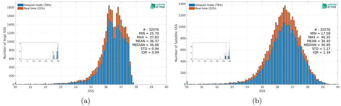
Figure 3: Histograms of SSS from Argo (a) and SMAP SSS L2 v5.3 - 40 km (RSS) (b) considering all match-up pairs per bins of 0.1 over the Amazon and Orinoco river plumes Pi-MEP region and for the full satellite product period.
