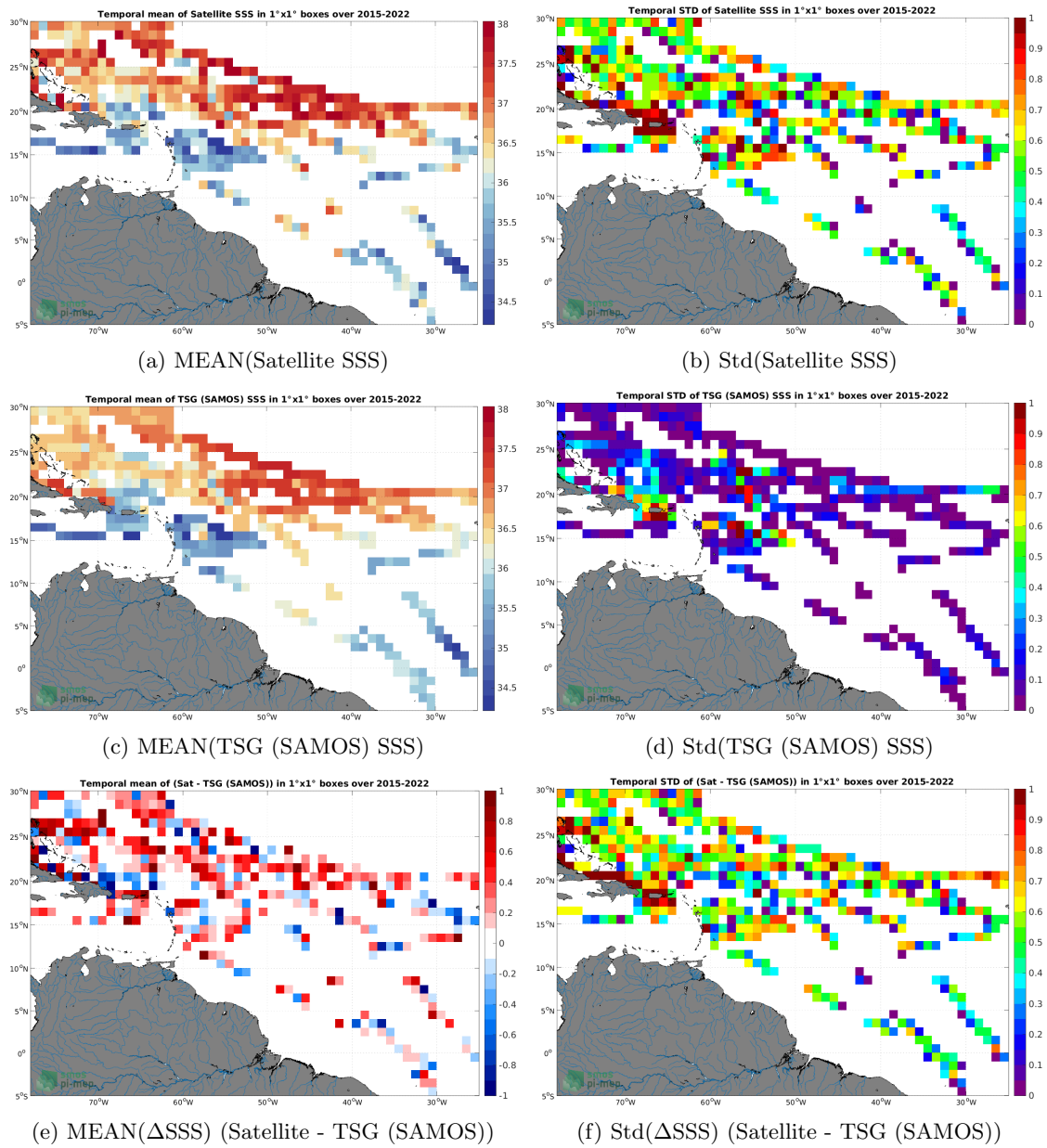
Figure 6: Temporal mean (left) and Std (right) of SSS from SMAP SSS L2 v5 - 40 km (RSS) (top), TSG (SAMOS) (middle), and of \Delta SSS (Satellite - TSG (SAMOS)). Only match-up pairs are used to generate these maps.
