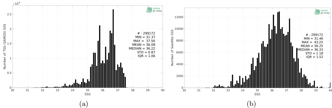
Figure 2: Histograms of SSS from TSG (SAMOS) (a) and SMAP SSS L2 v5 - 40 km (RSS) (b) considering all match-up pairs per bins of 0.1 over the Amazon and Orinoco river plumes Pi-MEP region and for the full satellite product period.
