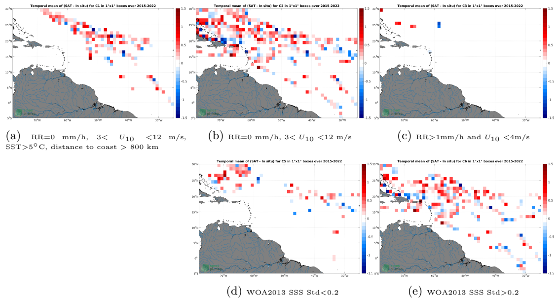
Figure 12: Temporal mean gridded over spatial boxes of size 1^\circ \times 1^\circ of \Delta SSS (SMAP SSS L2 v5 - 40 km (RSS) - TSG (SAMOS)) for 5 different subdatasets corresponding to:RR=0 mm/h, 3 < U_{10} < 12 m/s, SST > 5^\circ C , distance to coast > 800 km (a), RR=0 mm/h, 3 < U_{10} < 12 m/s (b), RR >1 mm/h and U_{10} < 4 m/s (c), WOA2013 SSS Std <0.2 (d), WOA2013 SSS Std >0.2 (e).
