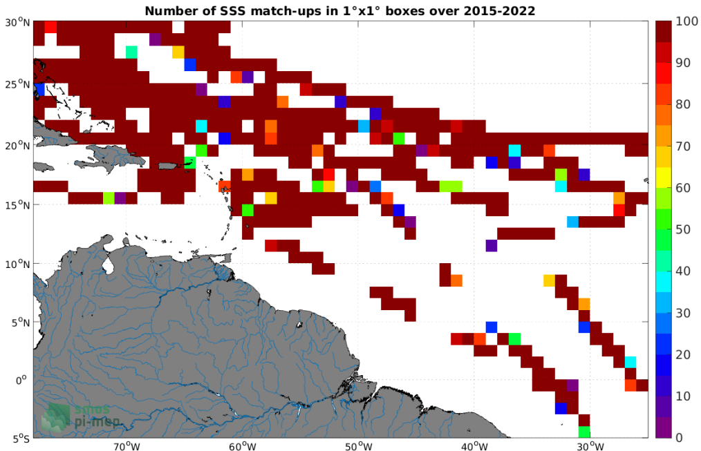
Figure 4: Number of SSS match-ups between TSG (SAMOS) SSS and the SMAP SSS L2 v5 - 40 km (RSS) SSS product for the Amazon and Orinoco river plumes Pi-MEP region over 1^\circ \times 1^\circ boxes and for the full satellite product period.
