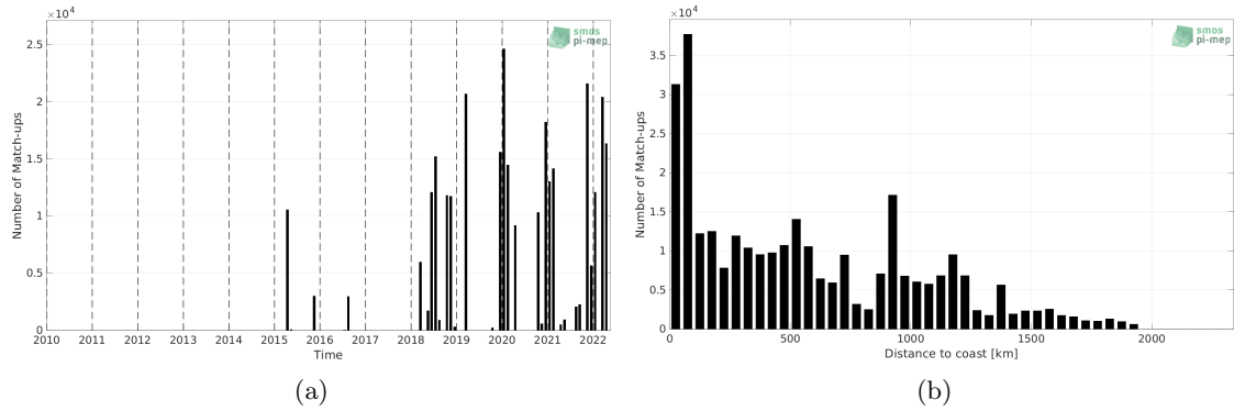
Figure 1: Number of match-ups between TSG (SAMOS) and SMAP SSS L2 v5 - 40 km (RSS) SSS as a function of time (a) and as function of the distance to coast (b) over the Amazon and Orinoco river plumes Pi-MEP region and for the full satellite product period.
