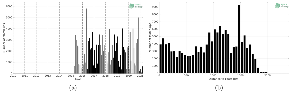
Figure 1: Number of match-ups between TSG (LEGOS-DM) and SMAP SSS L2 v5 - 40 km (RSS) SSS as a function of time (a) and as function of the distance to coast (b) over the Amazon and Orinoco river plumes Pi-MEP region and for the full satellite product period.
