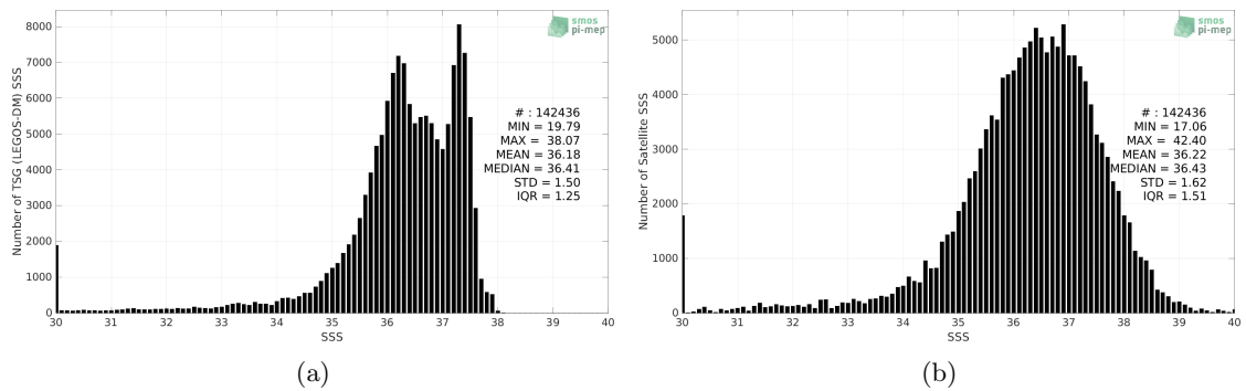
Figure 2: Histograms of SSS from TSG (LEGOS-DM) (a) and SMAP SSS L2 v5 - 40 km (RSS) (b) considering all match-up pairs per bins of 0.1 over the Amazon and Orinoco river plumes Pi-MEP region and for the full satellite product period.
