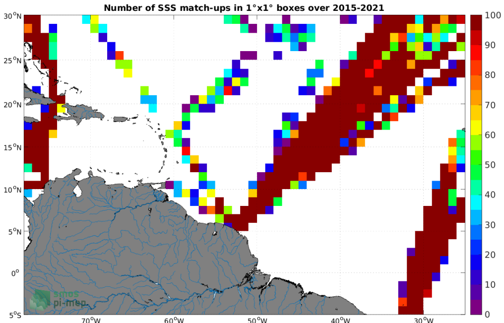
Figure 4: Number of SSS match-ups between TSG (LEGOS-DM) SSS and the SMAP SSS L2 v5 - 40 km (RSS) SSS product for the Amazon and Orinoco river plumes Pi-MEP region over 1^\circ \times 1^\circ boxes and for the full satellite product period.
