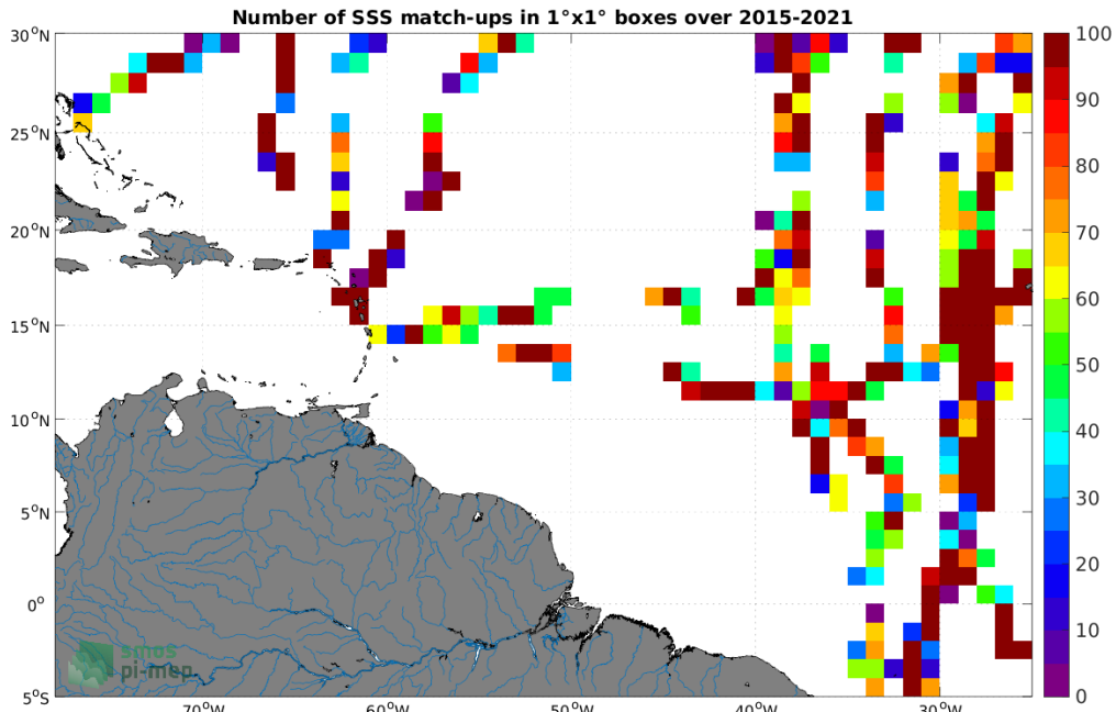
Figure 4: Number of SSS match-ups between TSG (GOSUD-Sailing-ship) SSS and the SMAP SSS L2 v5 - 40 km (RSS) SSS product for the Amazon and Orinoco river plumes Pi-MEP region over 1^\circ \times 1^\circ boxes and for the full satellite product period.
