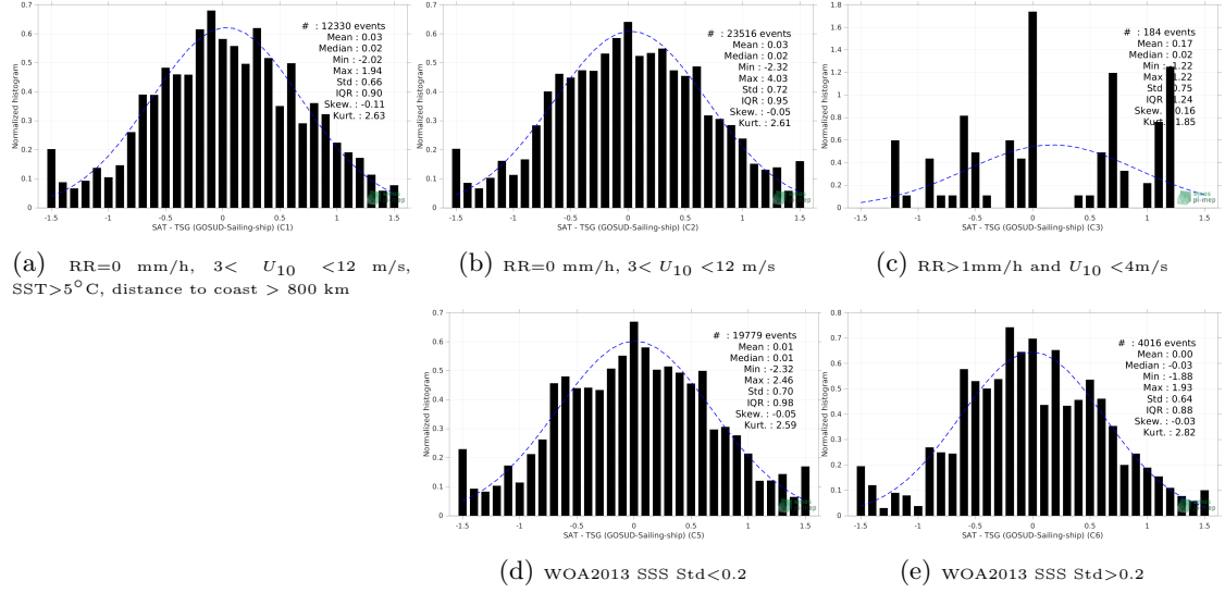
Figure 13: Normalized histogram of \Delta SSS (SMAP SSS L2 v5 - 40 km (RSS) - TSG (GOSUD-Sailing-ship)) for 5 different subdatasets corresponding to: RR=0 mm/h, 3 < U_{10} < 12 m/s, SST>5°C, distance to coast > 800 km (a), RR=0 mm/h, 3 < U_{10} < 12 m/s (b), RR>1mm/h and U_{10} < 4 m/s (c), WOA2013 SSS Std<0.2 (d), WOA2013 SSS Std>0.2 (e).
