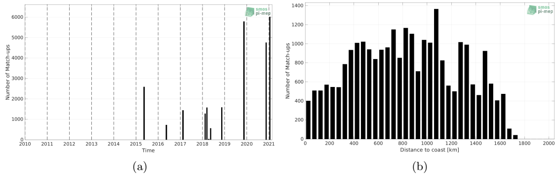
Figure 1: Number of match-ups between TSG (GOSUD-Sailing-ship) and SMAP SSS L2 v5 - 40 km (RSS) SSS as a function of time (a) and as function of the distance to coast (b) over the Amazon and Orinoco river plumes Pi-MEP region and for the full satellite product period.
