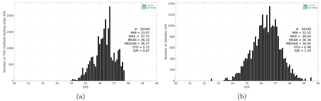
Figure 2: Histograms of SSS from TSG (GOSUD-Sailing-ship) (a) and SMAP SSS L2 v5 - 40 km (RSS) (b) considering all match-up pairs per bins of 0.1 over the Amazon and Orinoco river plumes Pi-MEP region and for the full satellite product period.
