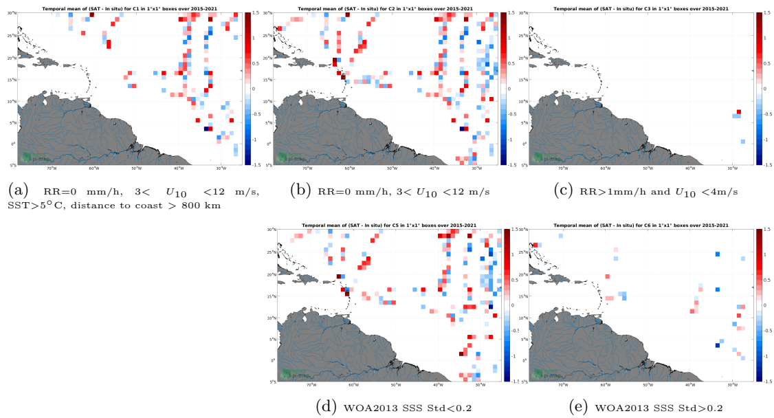
Figure 12: Temporal mean gridded over spatial boxes of size 1^\circ \times 1^\circ of \Delta SSS (SMAP SSS L2 v5 - 40 km (RSS) - TSG (GOSUD-Sailing-ship)) for 5 different subdatasets corresponding to:RR=0 mm/h, 3 < U_{10} < 12 m/s, SST>5°C, distance to coast > 800 km (a), RR=0 mm/h, 3 < U_{10} < 12 m/s (b), RR>1mm/h and U_{10} < 4 m/s (c), WOA2013 SSS Std<0.2 (d), WOA2013 SSS Std>0.2 (e).
