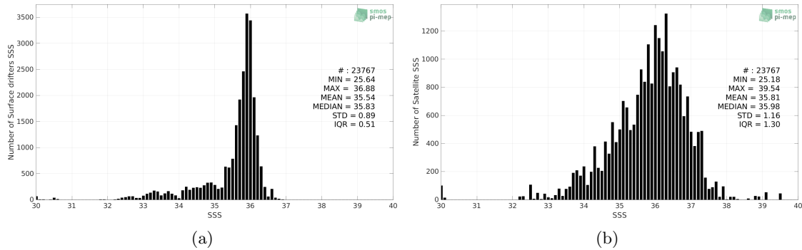
Figure 2: Histograms of SSS from Surface drifters (a) and SMAP SSS L2 v5 - 40 km (RSS) (b) considering all match-up pairs per bins of 0.1 over the Amazon and Orinoco river plumes Pi-MEP region and for the full satellite product period.
