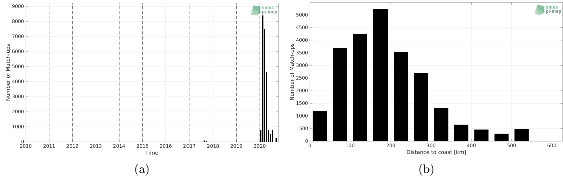
Figure 1: Number of match-ups between Surface drifters and SMAP SSS L2 v5 - 40 km (RSS) SSS as a function of time (a) and as function of the distance to coast (b) over the Amazon and Orinoco river plumes Pi-MEP region and for the full satellite product period.
