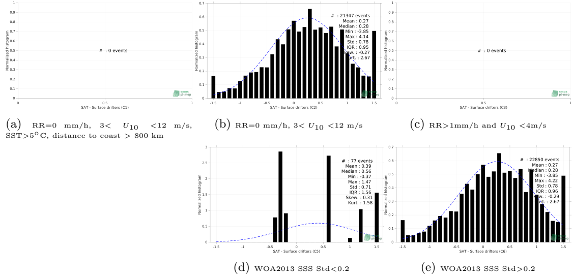
Figure 12: Normalized histogram of \Delta SSS (SMAP SSS L2 v5 - 40 km (RSS) - Surface drifters) for 5 different subdatasets corresponding to: RR=0 mm/h, 3 < U_{10} < 12 m/s, SST > 5°C, distance to coast > 800 km (a), RR=0 mm/h, 3 < U_{10} < 12 m/s (b), RR > 1mm/h and U_{10} < 4 m/s (c), WOA2013 SSS Std < 0.2 (d), WOA2013 SSS Std > 0.2 (e).
