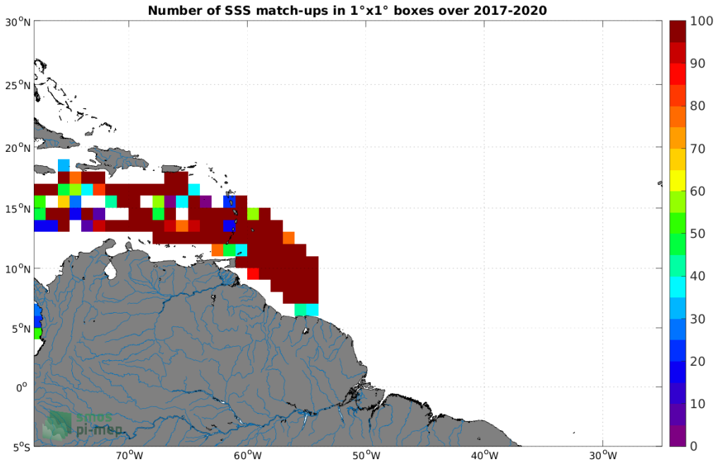
Figure 3: Number of SSS match-ups between Surface drifters SSS and the SMAP SSS L2 v5 - 40 km (RSS) SSS product for the Amazon and Orinoco river plumes Pi-MEP region over 1°x1° boxes and for the full satellite product period.
