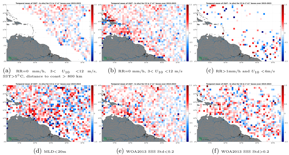
Figure 12: Temporal mean gridded over spatial boxes of size 1^\circ \times 1^\circ of \Delta SSS (SMAP SSS L2 v5 - 40 km (RSS) - Argo) for 6 different subdatasets corresponding to: RR=0 mm/h, 3 < U_{10} < 12 m/s, SST > 5^\circ\text{C} , distance to coast > 800 km (a), RR=0 mm/h, 3 < U_{10} < 12 m/s (b), RR > 1 mm/h and U_{10} < 4 m/s (c),MLD < 20 m (d),WOA2013 SSS Std < 0.2 (e),WOA2013 SSS Std > 0.2 (f).
