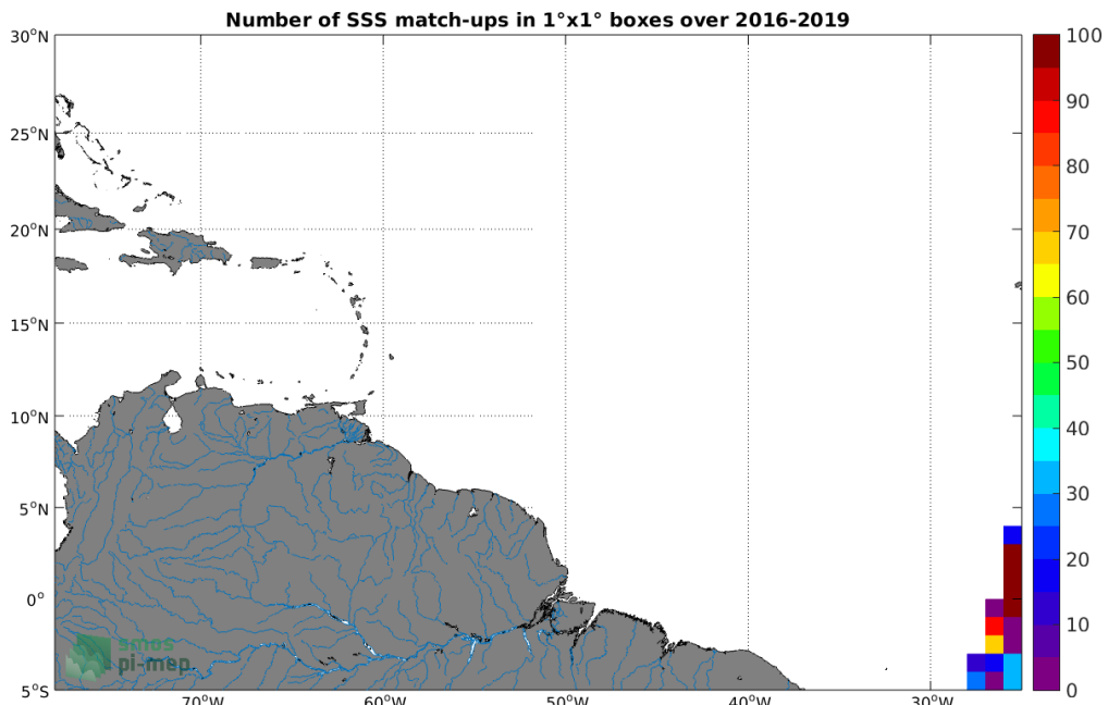
Figure 4: Number of SSS match-ups between TSG (Polarstern) SSS and the SMAP SSS L2 v4 (RSS) SSS product for the Amazon and Orinoco river plumes Pi-MEP region over 1^\circ \times 1^\circ boxes and for the full satellite product period.
