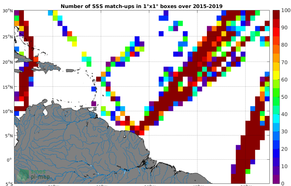
Figure 4: Number of SSS match-ups between TSG-LEGOS-DM SSS and the SMAP-L2-RSS-V4 SSS product for the Amazon and Orinoco river plumes Pi-MEP region over 1°x1° boxes and for the full satellite product period.
