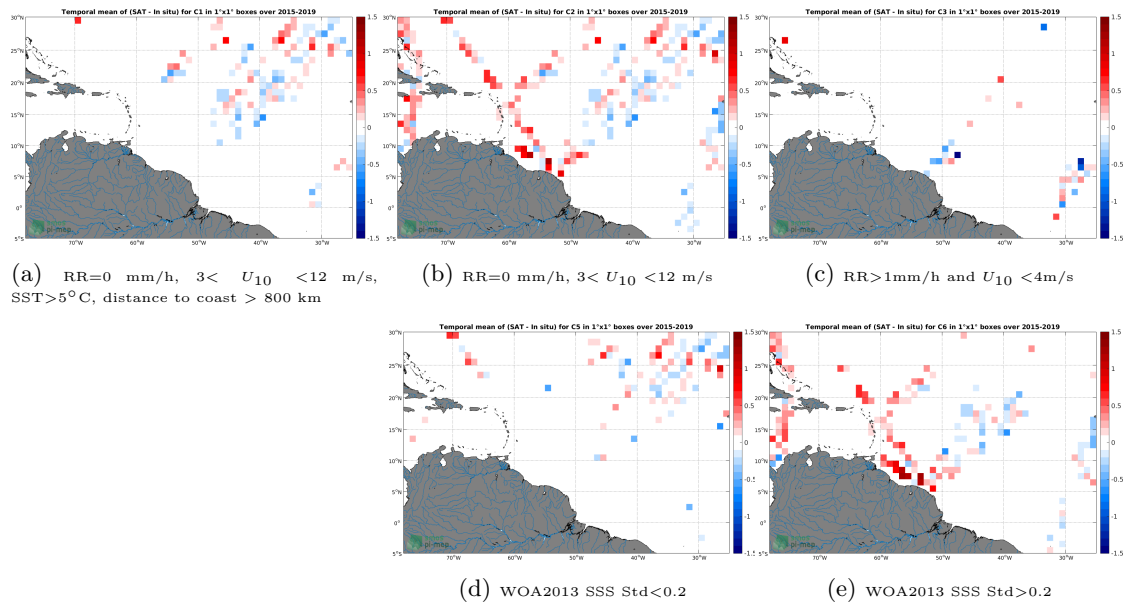
Figure 12: Temporal mean gridded over spatial boxes of size 1^\circ \times 1^\circ of \Delta SSS (SMAP-L2-RSS-V4 - TSG-LEGOS-DM) for 5 different subdatasets corresponding to:RR=0 mm/h, 3 < U_{10} < 12 m/s, SST >5^\circ\text{C} , distance to coast > 800 km (a), RR=0 mm/h, 3 < U_{10} < 12 m/s (b), RR >1 mm/h and U_{10} < 4 m/s (c), WOA2013 SSS Std <0.2 (d), WOA2013 SSS Std >0.2 (e).
