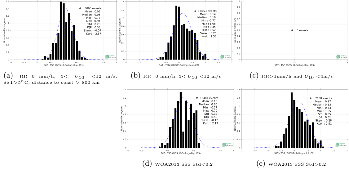
Figure 13: Normalized histogram of \Delta\text{SSS} (SMAP SSS L2 v4 (RSS) - TSG (GOSUD-Sailing-ship)) for 5 different subdatasets corresponding to: RR=0 mm/h, 3 < U_{10} < 12 m/s, SST > 5^\circ\text{C} , distance to coast > 800 km (a), RR=0 mm/h, 3 < U_{10} < 12 m/s (b), RR > 1 mm/h and U_{10} < 4 m/s (c), WOA2013 SSS Std < 0.2 (d), WOA2013 SSS Std > 0.2 (e).
