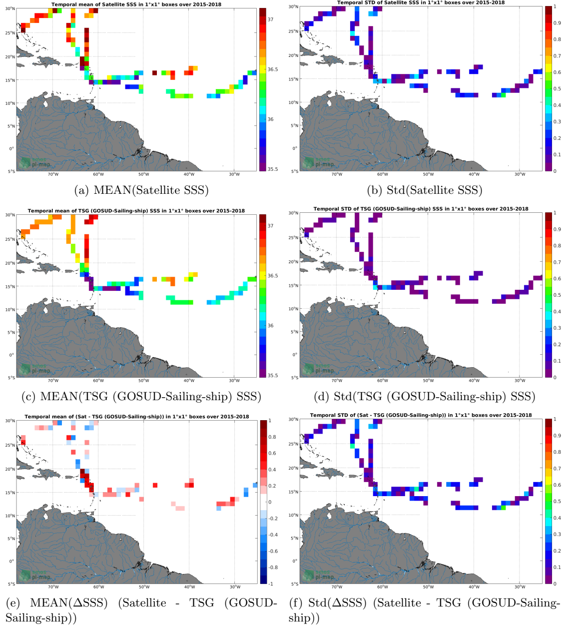
Figure 6: Temporal mean (left) and Std (right) of SSS from SMAP SSS L2 v4 (RSS) (top), TSG (GOSUD-Sailing-ship) (middle), and of \Delta SSS (Satellite - TSG (GOSUD-Sailing-ship)). Only match-up pairs are used to generate these maps.
