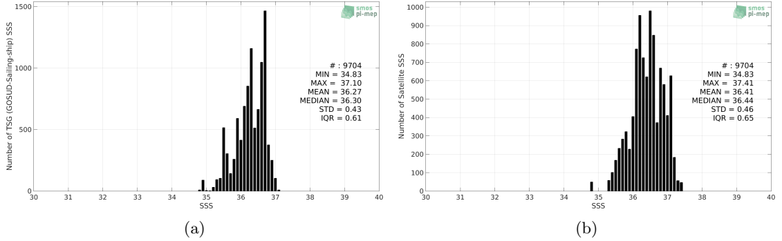
Figure 2: Histograms of SSS from TSG (GOSUD-Sailing-ship) (a) and SMAP SSS L2 v4 (RSS) (b) considering all match-up pairs per bins of 0.1 over the Amazon and Orinoco river plumes Pi-MEP region and for the full satellite product period.
