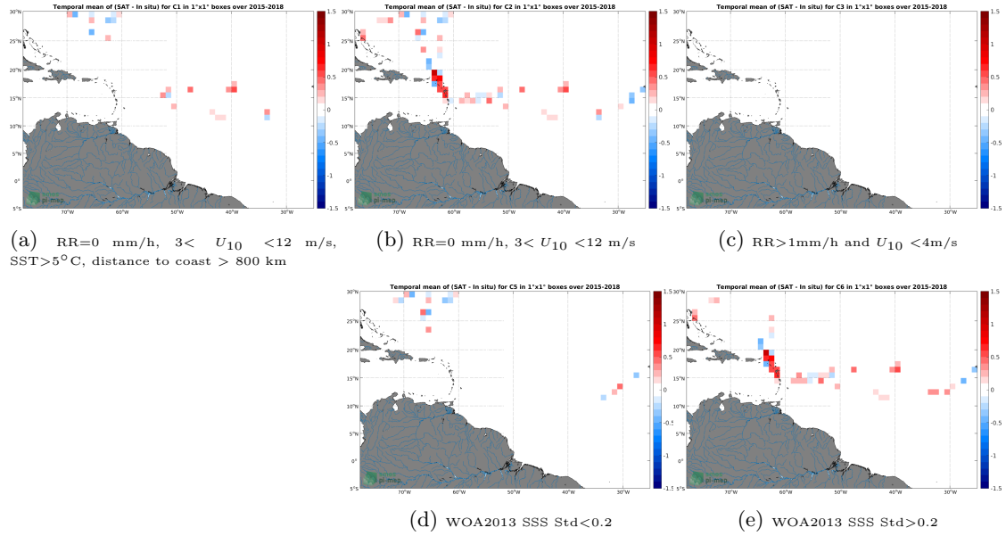
Figure 12: Temporal mean gridded over spatial boxes of size 1^\circ \times 1^\circ of \Delta SSS (SMAP SSS L2 v4 (RSS) - TSG (GOSUD-Sailing-ship)) for 5 different subdatasets corresponding to: RR=0 mm/h, 3 < U_{10} < 12 m/s, SST > 5^\circ\text{C} , distance to coast > 800 km (a), RR=0 mm/h, 3 < U_{10} < 12 m/s (b), RR > 1 mm/h and U_{10} < 4 m/s (c), WOA2013 SSS Std < 0.2 (d), WOA2013 SSS Std > 0.2 (e).
