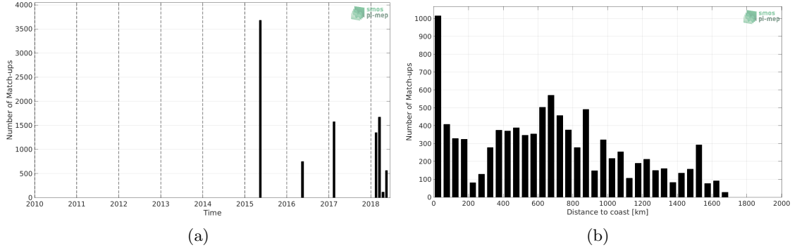
Figure 1: Number of match-ups between TSG (GOSUD-Sailing-ship) and SMAP SSS L2 v4 (RSS) SSS as a function of time (a) and as function of the distance to coast (b) over the Amazon and Orinoco river plumes Pi-MEP region and for the full satellite product period.
