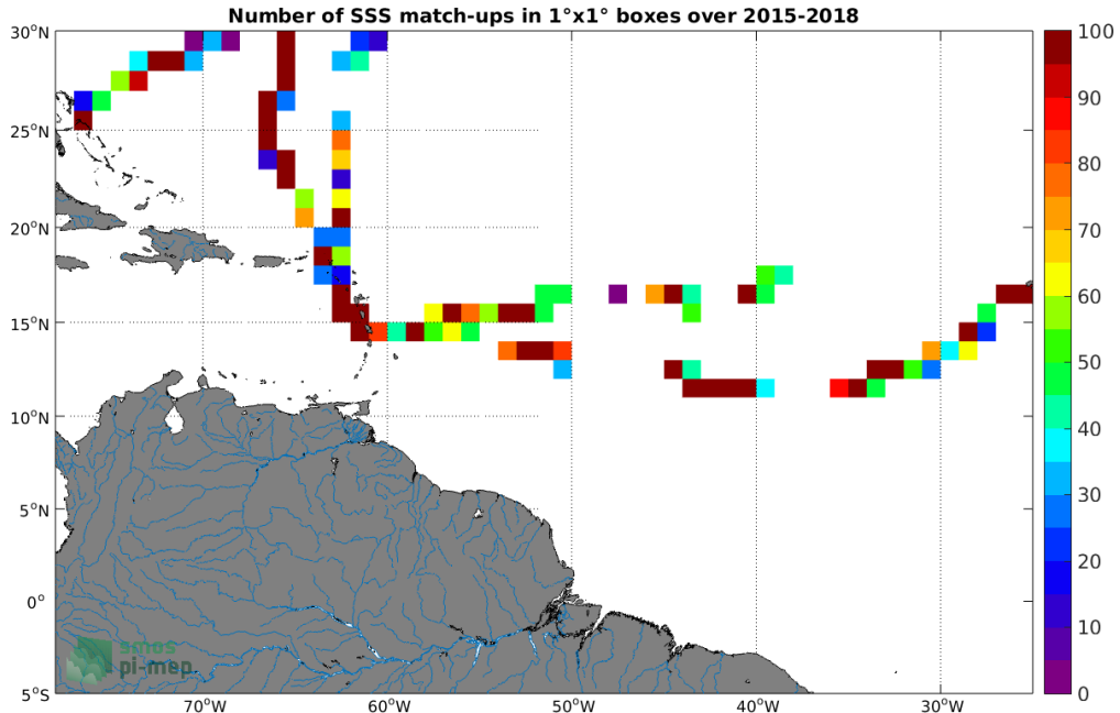
Figure 4: Number of SSS match-ups between TSG (GOSUD-Sailing-ship) SSS and the SMAP SSS L2 v4 (RSS) SSS product for the Amazon and Orinoco river plumes Pi-MEP region over 1^\circ \times 1^\circ boxes and for the full satellite product period.
