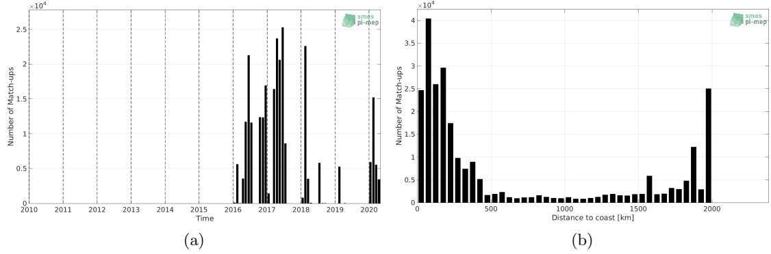
Figure 1: Number of match-ups between TSG (GOSUD-Research-vessel) and SMAP SSS L2 v4 (RSS) SSS as a function of time (a) and as function of the distance to coast (b) over the Amazon and Orinoco river plumes Pi-MEP region and for the full satellite product period.
