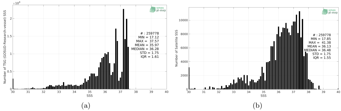
Figure 2: Histograms of SSS from TSG (GOSUD-Research-vessel) (a) and SMAP SSS L2 v4 (RSS) (b) considering all match-up pairs per bins of 0.1 over the Amazon and Orinoco river plumes Pi-MEP region and for the full satellite product period.
