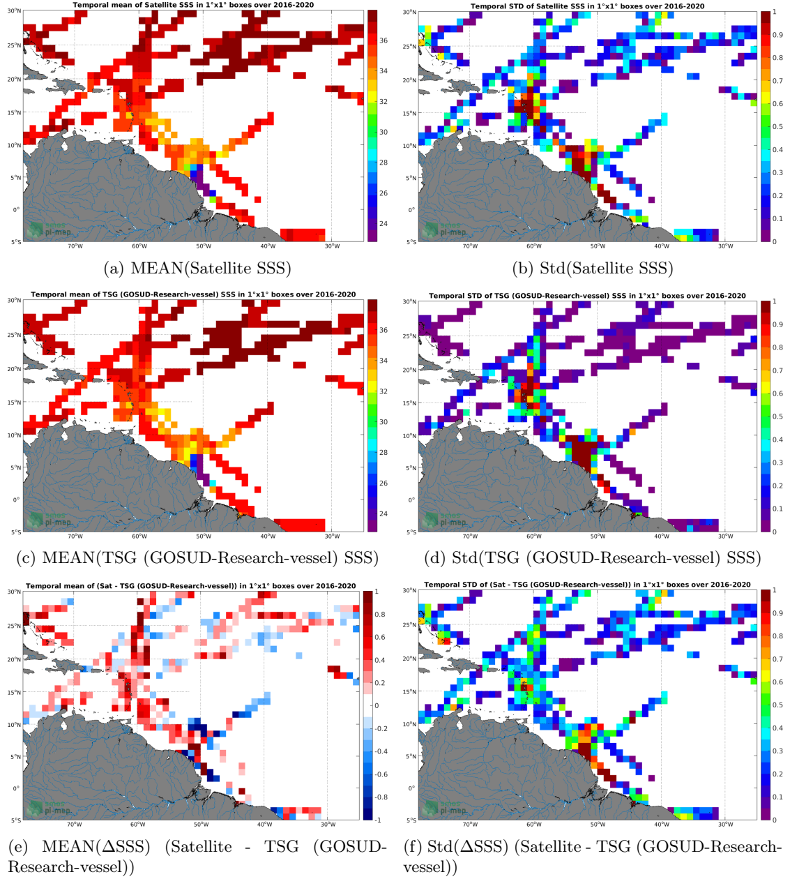
Figure 6: Temporal mean (left) and Std (right) of SSS from SMAP SSS L2 v4 (RSS) (top), TSG (GOSUD-Research-vessel) (middle), and of \Delta SSS (Satellite - TSG (GOSUD-Research-vessel)). Only match-up pairs are used to generate these maps.
