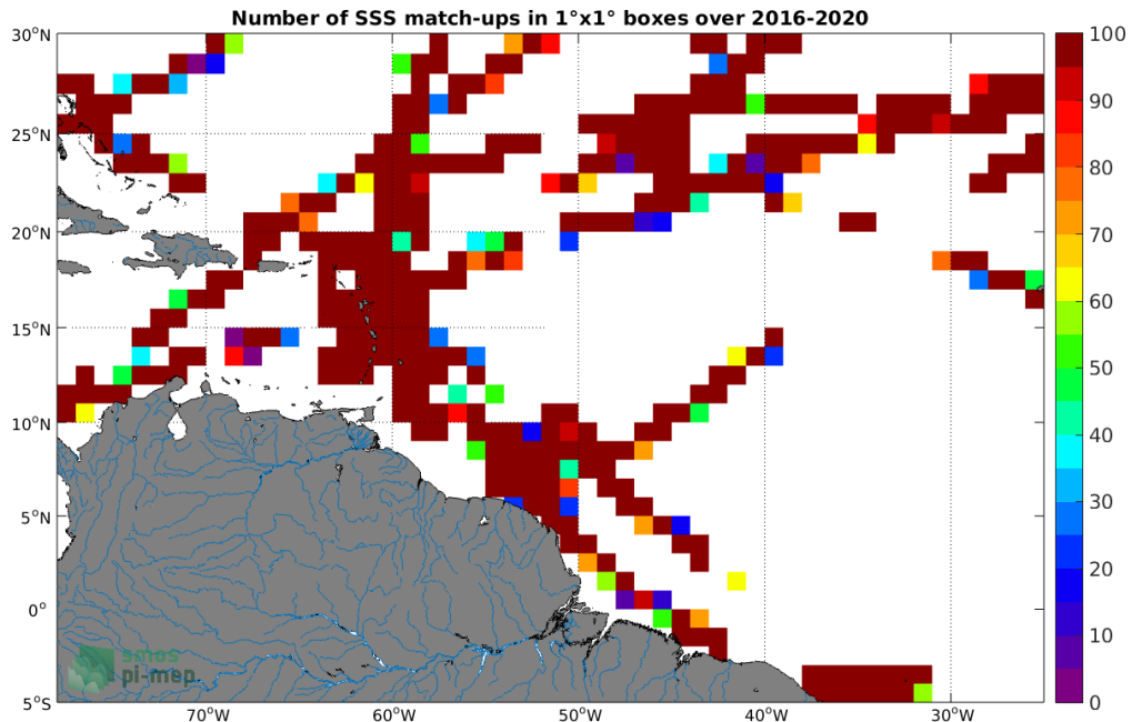
Figure 4: Number of SSS match-ups between TSG (GOSUD-Research-vessel) SSS and the SMAP SSS L2 v4 (RSS) SSS product for the Amazon and Orinoco river plumes Pi-MEP region over 1^\circ \times 1^\circ boxes and for the full satellite product period.
