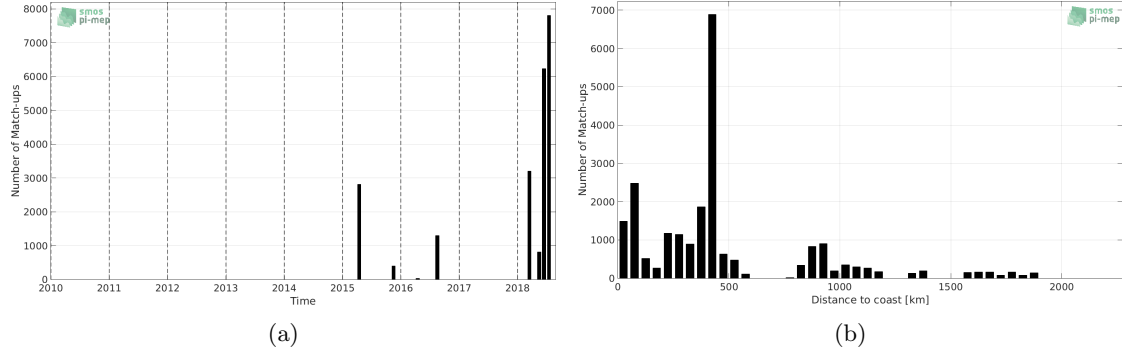
Figure 1: Number of match-ups between TSG-SAMOS and SMAP-L2-RSS-V3-70KM SSS as a function of time (a) and as function of the distance to coast (b) over the Amazon and Orinoco river plumes Pi-MEP region and for the full satellite product period.
