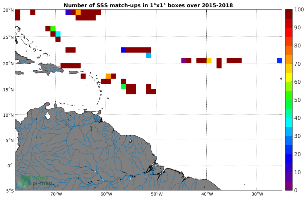
Figure 4: Number of SSS match-ups between TSG-SAMOS SSS and the SMAP-L2-RSS-V3-70KM SSS product for the Amazon and Orinoco river plumes Pi-MEP region over 1^\circ \times 1^\circ boxes and for the full satellite product period.
