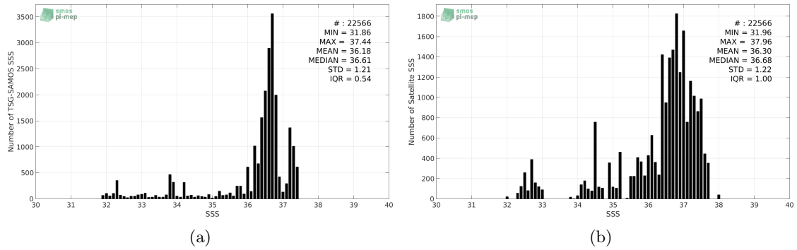
Figure 2: Histograms of SSS from TSG-SAMOS (a) and SMAP-L2-RSS-V3-70KM (b) considering all match-up pairs per bins of 0.1 over the Amazon and Orinoco river plumes Pi-MEP region and for the full satellite product period.
