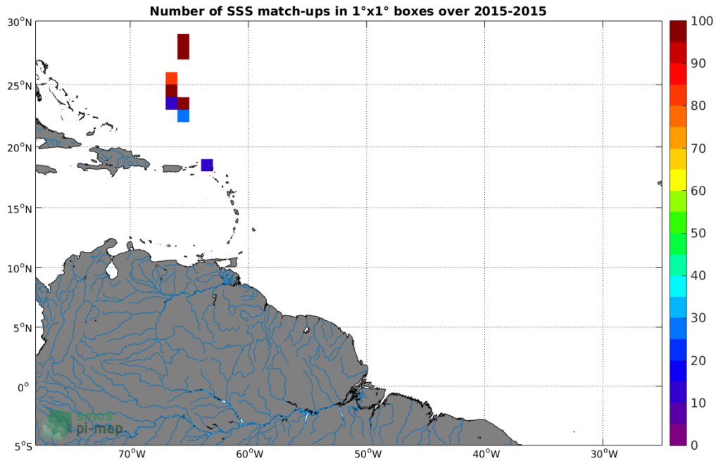
Figure 4: Number of SSS match-ups between TSG-GOSUD-Sailing-ship SSS and the SMAP-L2-RSS-V3-70KM SSS product for the Amazon and Orinoco river plumes Pi-MEP region over 1^\circ \times 1^\circ boxes and for the full satellite product period.
