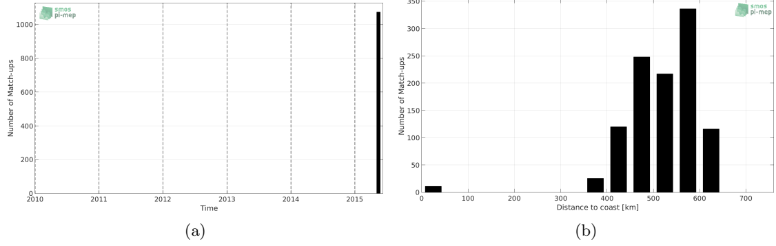
Figure 1: Number of match-ups between TSG-GOSUD-Sailing-ship and SMAP-L2-RSS-V3-70KM SSS as a function of time (a) and as function of the distance to coast (b) over the Amazon and Orinoco river plumes Pi-MEP region and for the full satellite product period.
