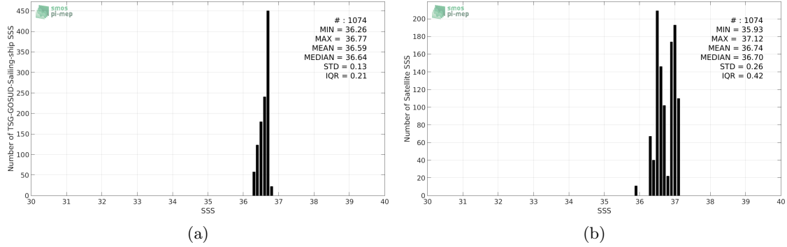
Figure 2: Histograms of SSS from TSG-GOSUD-Sailing-ship (a) and SMAP-L2-RSS-V3-70KM (b) considering all match-up pairs per bins of 0.1 over the Amazon and Orinoco river plumes Pi-MEP region and for the full satellite product period.
