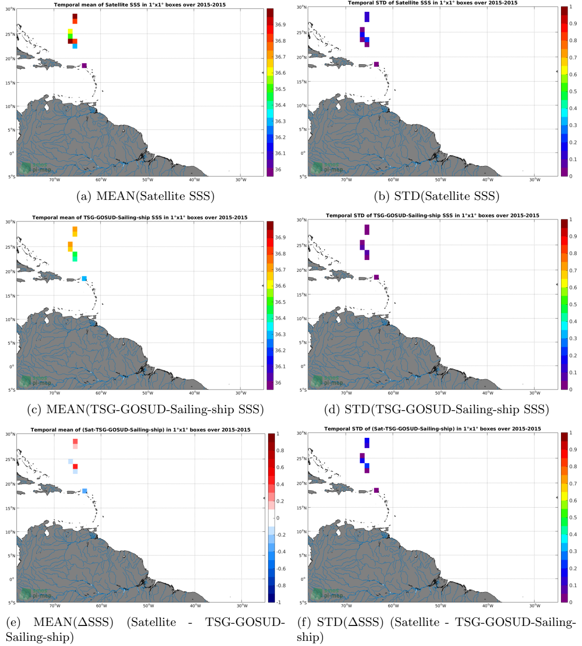
Figure 6: Temporal mean (left) and STD (right) of SSS from SMAP-L2-RSS-V3-70KM (top), TSG-GOSUD-Sailing-ship (middle), and of \Delta SSS (Satellite - TSG-GOSUD-Sailing-ship). Only match-up pairs are used to generate these maps.
