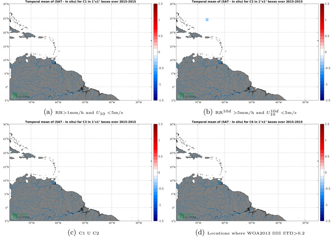
Figure 12: Temporal mean gridded over spatial boxes of size 1^\circ \times 1^\circ of \Delta SSS (SMAP-L2-RSS-V3-70KM - TSG-GOSUD-Sailing-ship) for 4 different subdatasets corresponding to: RR > 1\text{mm/h} and U_{10} < 5\text{m/s} (a), RR^{10d} > 5\text{mm/h} and U_{10}^{10d} < 5\text{m/s} (b), C1 U C2 (c), Locations where WOA2013 SSS STD > 0.2 (d).
