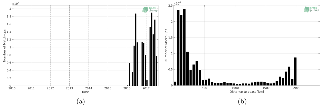
Figure 1: Number of match-ups between TSG-GOSUD-Research-vessel and SMAP-L2-RSS-V3-70KM SSS as a function of time (a) and as function of the distance to coast (b) over the Amazon and Orinoco river plumes Pi-MEP region and for the full satellite product period.
