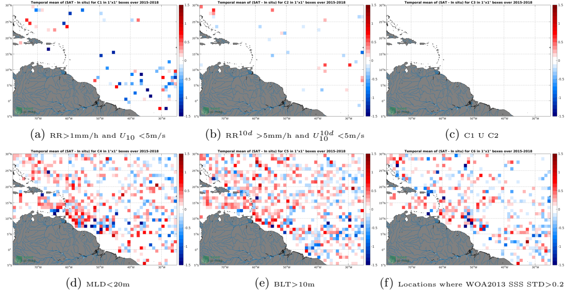
Figure 12: Temporal mean gridded over spatial boxes of size 1^\circ \times 1^\circ of \Delta\text{SSS} (SMAP-L2-RSS-V3-70KM - Argo) for 6 different subdatasets corresponding to: RR > 1\text{mm/h} and U_{10} < 5\text{m/s} (a), RR^{10d} > 5\text{mm/h} and U_{10}^{10d} < 5\text{m/s} (b), C1 U C2 (c), MLD < 20\text{m} (d), BLT > 10\text{m} (e), Locations where WOA2013 SSS STD > 0.2 (f).
