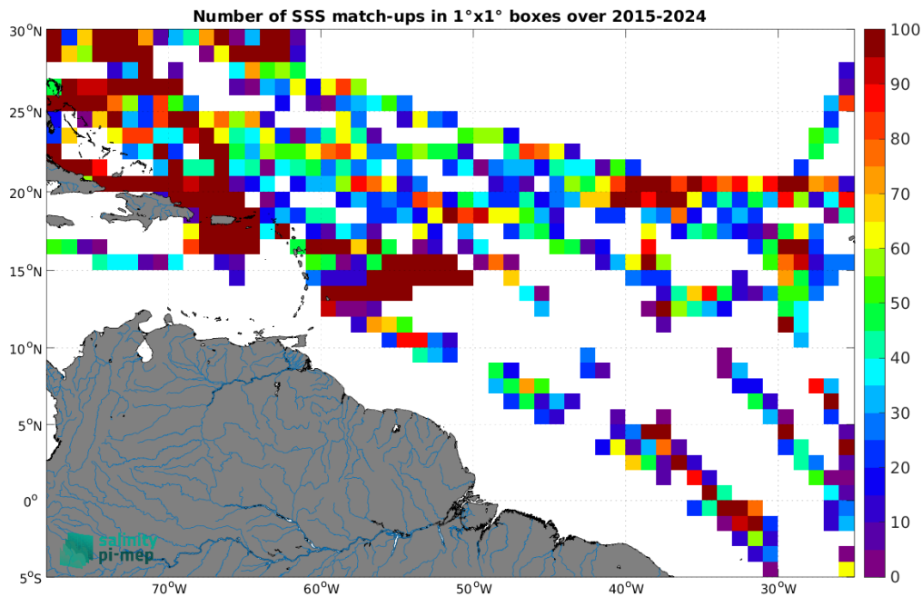
Figure 5: Number of SSS match-ups between TSG (SAMOS) SSS and the SMAP SSS L2 v5.0 (JPL) SSS product for the Amazon and Orinoco river plumes Pi-MEP region over 1^{\circ} \times 1^{\circ} boxes and for the full satellite product period.
