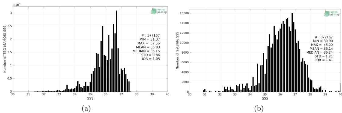
Figure 2: Histograms of SSS from TSG (SAMOS) (a) and SMAP SSS L2 v5.0 (JPL) (b) considering all match-up pairs per bins of 0.1 over the Amazon and Orinoco river plumes Pi-MEP region and for the full satellite product period.
