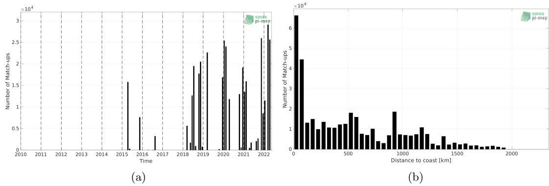
Figure 1: Number of match-ups between TSG (SAMOS) and SMAP SSS L2 v5.0 (JPL) SSS as a function of time (a) and as function of the distance to coast (b) over the Amazon and Orinoco river plumes Pi-MEP region and for the full satellite product period.
