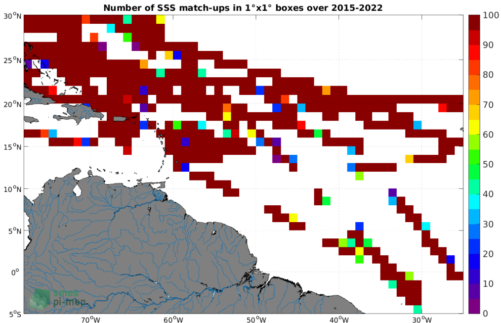
Figure 4: Number of SSS match-ups between TSG (SAMOS) SSS and the SMAP SSS L2 v5.0 (JPL) SSS product for the Amazon and Orinoco river plumes Pi-MEP region over 1^\circ \times 1^\circ boxes and for the full satellite product period.
