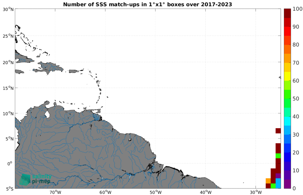
Figure 5: Number of SSS match-ups between TSG (Polarstern) SSS and the SMAP SSS L2 v5.0 (JPL) SSS product for the Amazon and Orinoco river plumes Pi-MEP region over 1^\circ \times 1^\circ boxes and for the full satellite product period.
