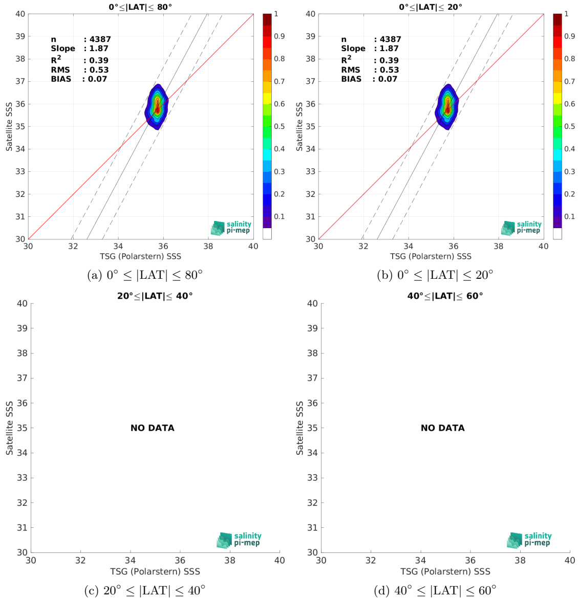
Figure 10: Contour maps of the concentration of SMAP SSS L2 v5.0 (JPL) SSS (y-axis) versus TSG (Polarstern) SSS (x-axis) at match-up pairs for different latitude bands. For each plot, the red line shows x=y . The black thin and dashed lines indicate a linear fit through the data cloud and the \pm 95\% confidence levels, respectively. The number match-up pairs n , the slope and R^2 coefficient of the linear fit, the root mean square (RMS) and the mean bias between satellite and in situ data are indicated for each latitude band in each plots.
