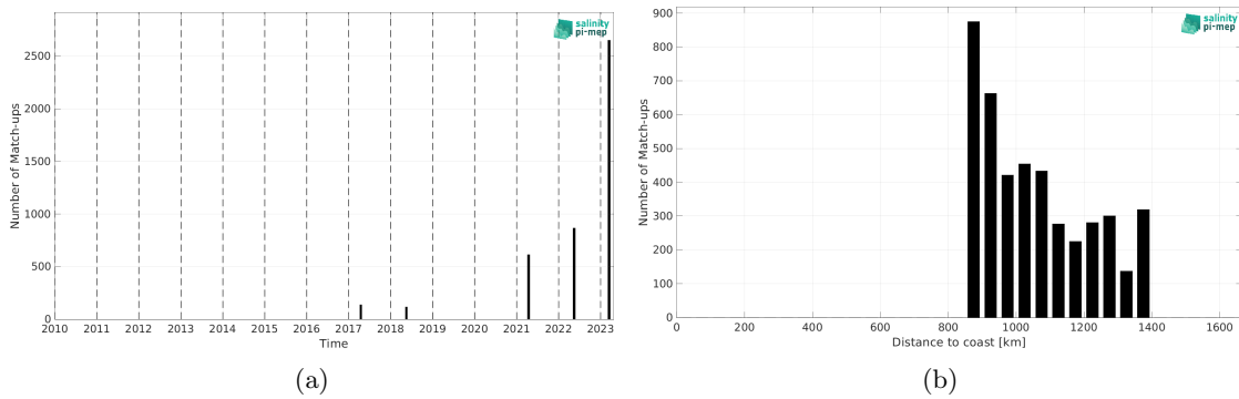
Figure 2: Number of match-ups between TSG (Polarstern) and SMAP SSS L2 v5.0 (JPL) SSS as a function of time (a) and as function of the distance to coast (b) over the Amazon and Orinoco river plumes Pi-MEP region and for the full satellite product period.
