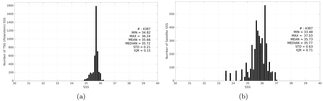
Figure 3: Histograms of SSS from TSG (Polarstern) (a) and SMAP SSS L2 v5.0 (JPL) (b) considering all match-up pairs per bins of 0.1 over the Amazon and Orinoco river plumes Pi-MEP region and for the full satellite product period.
