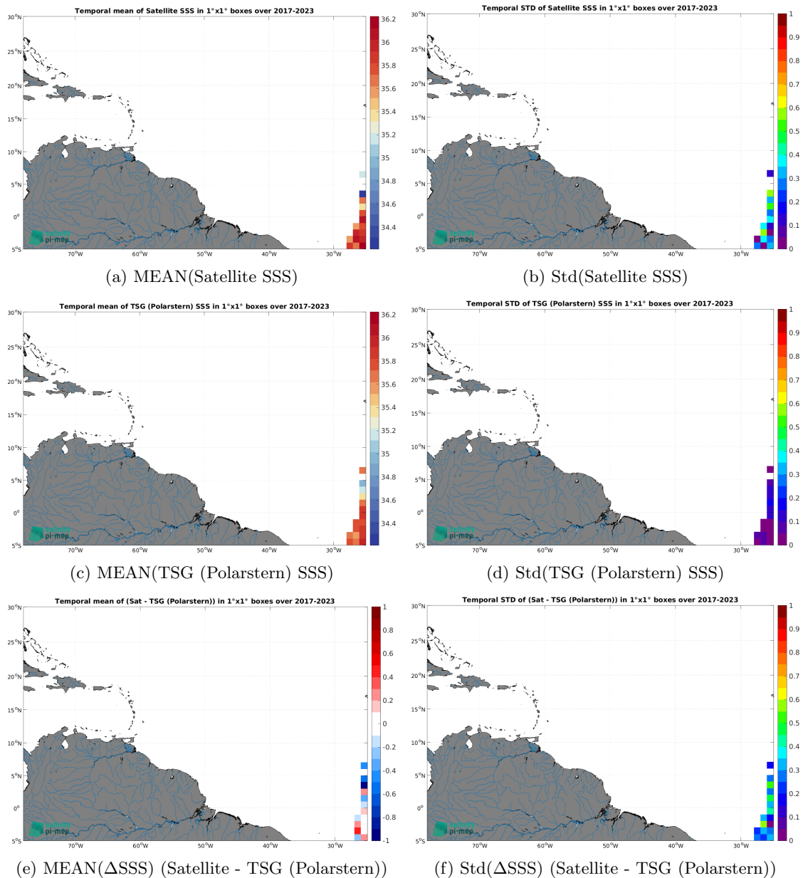
Figure 7: Temporal mean (left) and Std (right) of SSS from SMAP SSS L2 v5.0 (JPL) (top), TSG (Polarstern) (middle), and of \Delta SSS (Satellite - TSG (Polarstern)). Only match-up pairs are used to generate these maps.
