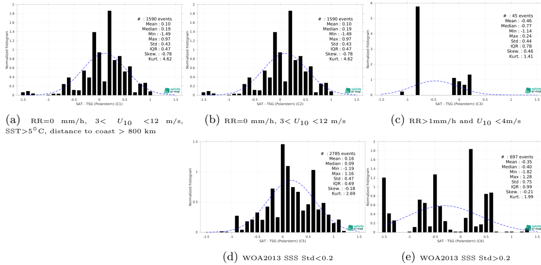
Figure 15: Normalized histogram of \Delta SSS (SMAP SSS L2 v5.0 (JPL) - TSG (Polarstern)) for 5 different subdatasets corresponding to: RR=0 mm/h, 3 < U_{10} < 12 m/s, SST>5°C, distance to coast > 800 km (a), RR=0 mm/h, 3 < U_{10} < 12 m/s (b), RR>1mm/h and U_{10} < 4 m/s (c), WOA2013 SSS Std<0.2 (d), WOA2013 SSS Std>0.2 (e).
