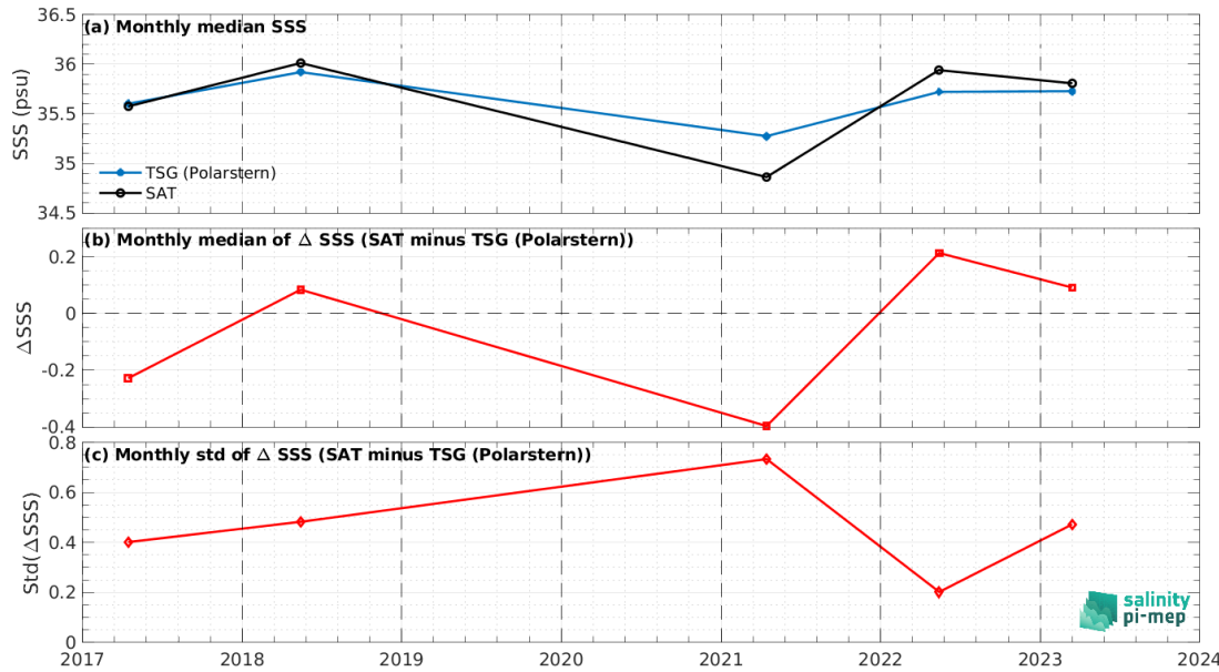
Figure 8: Time series of the monthly median SSS (top), median of \Delta\text{SSS} (Satellite - TSG (Polarstern)) and Std of \Delta\text{SSS} (Satellite - TSG (Polarstern)) over the Amazon and Orinoco river plumes Pi-MEP region considering all match-ups collected by the Pi-MEP.
