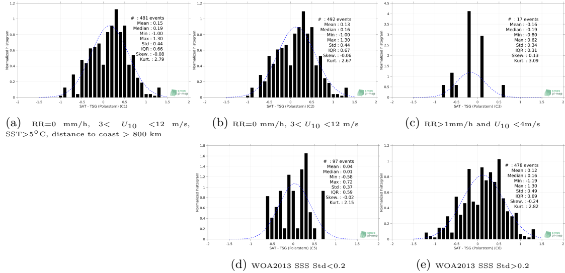
Figure 13: Normalized histogram of \Delta SSS (SMAP SSS L2 v5.0 (JPL) - TSG (Polarstern)) for 5 different subdatasets corresponding to: RR=0 mm/h, 3 < U_{10} < 12 m/s, SST > 5°C, distance to coast > 800 km (a), RR=0 mm/h, 3 < U_{10} < 12 m/s (b), RR > 1mm/h and U_{10} < 4 m/s (c), WOA2013 SSS Std < 0.2 (d), WOA2013 SSS Std > 0.2 (e).
