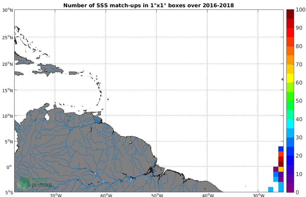
Figure 4: Number of SSS match-ups between TSG (Polarstern) SSS and the SMAP SSS L2 v5.0 (JPL) SSS product for the Amazon and Orinoco river plumes Pi-MEP region over 1°x1° boxes and for the full satellite product period.
