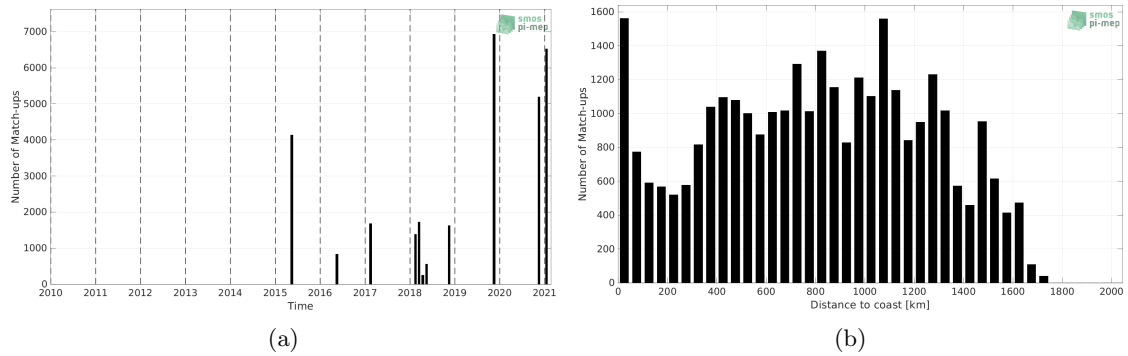
Figure 1: Number of match-ups between TSG (GOSUD-Sailing-ship) and SMAP SSS L2 v5.0 (JPL) SSS as a function of time (a) and as function of the distance to coast (b) over the Amazon and Orinoco river plumes Pi-MEP region and for the full satellite product period.
