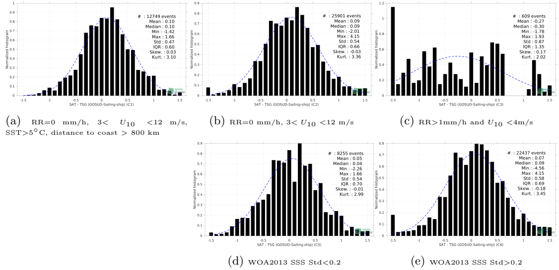
Figure 13: Normalized histogram of \Delta SSS (SMAP SSS L2 v5.0 (JPL) - TSG (GOSUD-Sailing-ship)) for 5 different subdatasets corresponding to: RR=0 mm/h, 3 < U_{10} < 12 m/s, SST>5°C, distance to coast > 800 km (a), RR=0 mm/h, 3 < U_{10} < 12 m/s (b), RR>1mm/h and U_{10} < 4 m/s (c), WOA2013 SSS Std<0.2 (d), WOA2013 SSS Std>0.2 (e).
