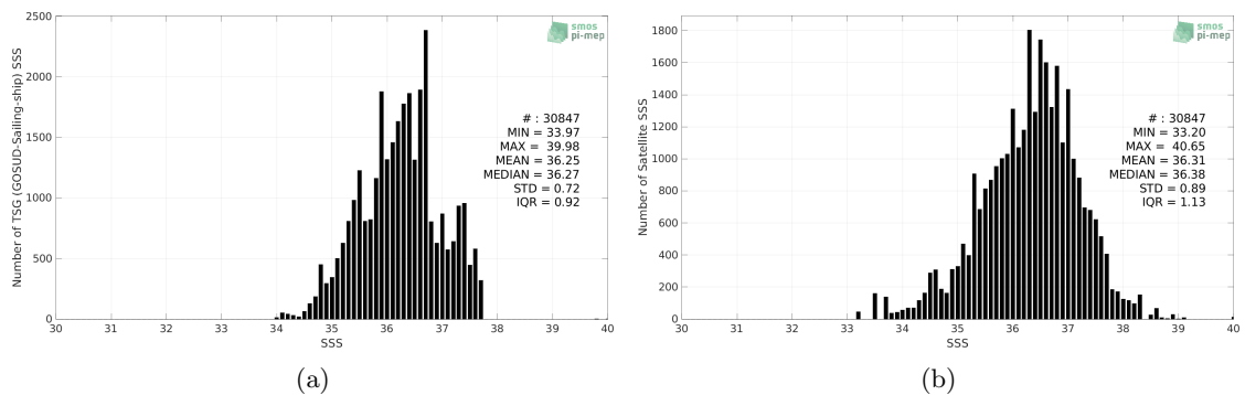
Figure 2: Histograms of SSS from TSG (GOSUD-Sailing-ship) (a) and SMAP SSS L2 v5.0 (JPL) (b) considering all match-up pairs per bins of 0.1 over the Amazon and Orinoco river plumes Pi-MEP region and for the full satellite product period.
