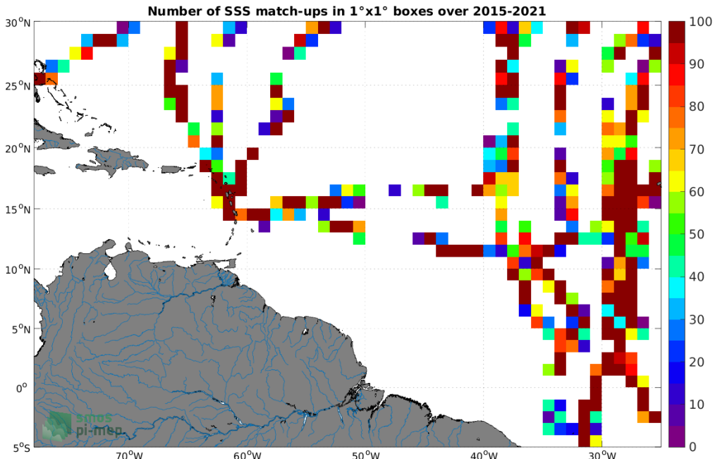
Figure 4: Number of SSS match-ups between TSG (GOSUD-Sailing-ship) SSS and the SMAP SSS L2 v5.0 (JPL) SSS product for the Amazon and Orinoco river plumes Pi-MEP region over 1^\circ \times 1^\circ boxes and for the full satellite product period.
