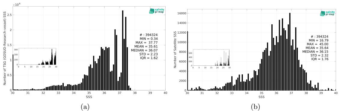
Figure 3: Histograms of SSS from TSG (GOSUD-Research-vessel) (a) and SMAP SSS L2 v5.0 (JPL) (b) considering all match-up pairs per bins of 0.1 over the Amazon and Orinoco river plumes Pi-MEP region and for the full satellite product period.
