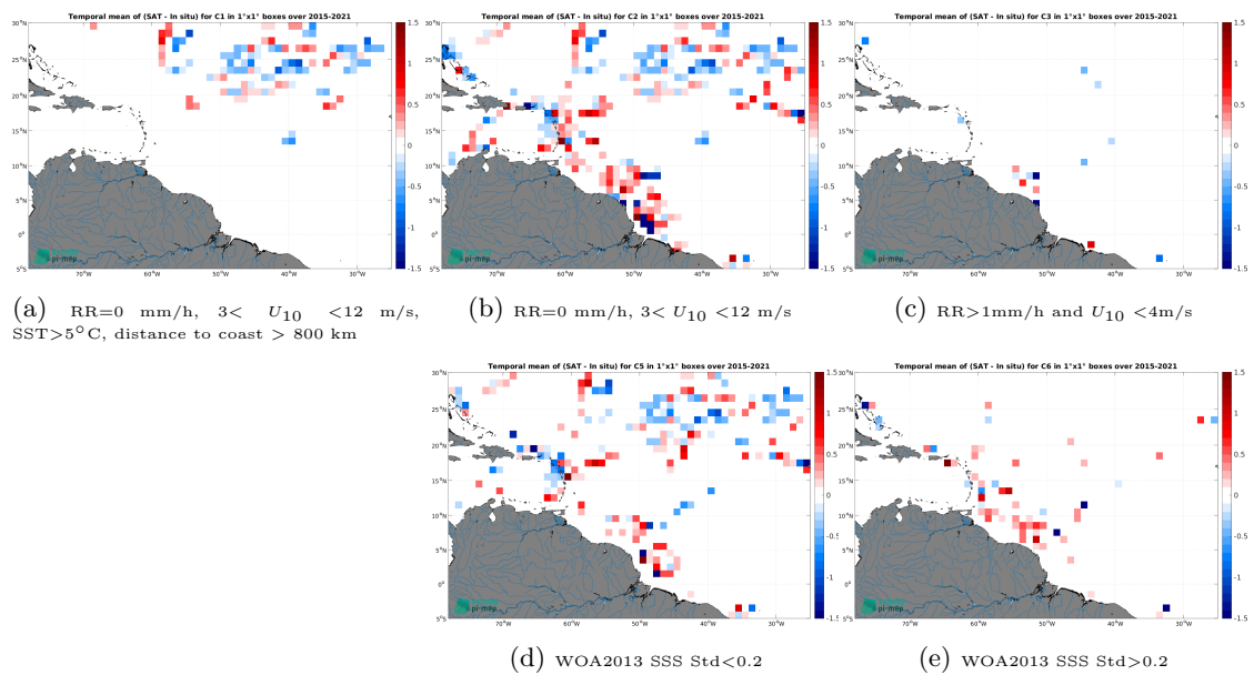
Figure 14: Temporal mean gridded over spatial boxes of size 1^\circ \times 1^\circ of \Delta SSS (SMAP SSS L2 v5.0 (JPL) - TSG (GOSUD-Research-vessel)) for 5 different subdatasets corresponding to:RR=0 mm/h, 3 < U_{10} < 12 m/s, SST > 5°C, distance to coast > 800 km (a), RR=0 mm/h, 3 < U_{10} < 12 m/s (b), RR > 1mm/h and U_{10} < 4 m/s (c), WOA2013 SSS Std < 0.2 (d), WOA2013 SSS Std > 0.2 (e).
