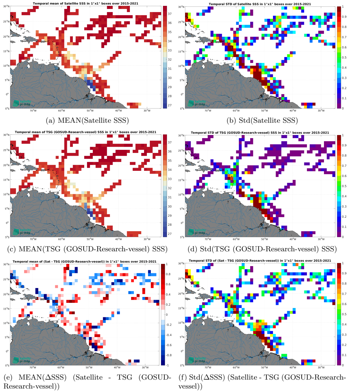
Figure 7: Temporal mean (left) and Std (right) of SSS from SMAP SSS L2 v5.0 (JPL) (top), TSG (GOSUD-Research-vessel) (middle), and of \Delta SSS (Satellite - TSG (GOSUD-Research-vessel)). Only match-up pairs are used to generate these maps.
