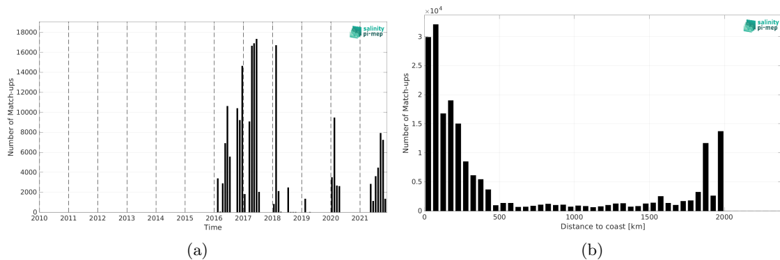
Figure 2: Number of match-ups between TSG (GOSUD-Research-vessel) and SMAP SSS L2 v5.0 (JPL) SSS as a function of time (a) and as function of the distance to coast (b) over the Amazon and Orinoco river plumes Pi-MEP region and for the full satellite product period.
