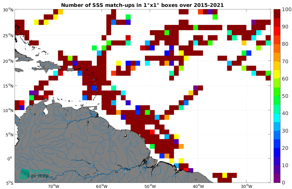
Figure 5: Number of SSS match-ups between TSG (GOSUD-Research-vessel) SSS and the SMAP SSS L2 v5.0 (JPL) SSS product for the Amazon and Orinoco river plumes Pi-MEP region over 1^\circ \times 1^\circ boxes and for the full satellite product period.
