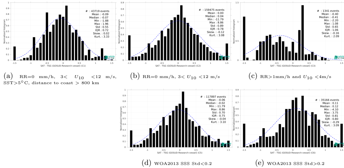
Figure 15: Normalized histogram of \Delta SSS (SMAP SSS L2 v5.0 (JPL) - TSG (GOSUD-Research-vessel)) for 5 different subdatasets corresponding to: RR=0 mm/h, 3 < U_{10} < 12 m/s, SST>5°C, distance to coast > 800 km (a), RR=0 mm/h, 3 < U_{10} < 12 m/s (b), RR>1mm/h and U_{10} < 4 m/s (c), WOA2013 SSS Std<0.2 (d), WOA2013 SSS Std>0.2 (e).
