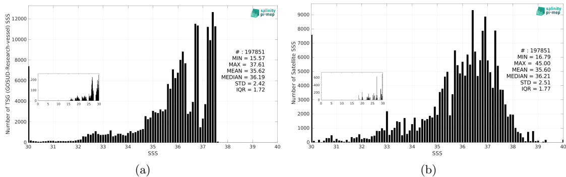
Figure 3: Histograms of SSS from TSG (GOSUD-Research-vessel) (a) and SMAP SSS L2 v5.0 (JPL) (b) considering all match-up pairs per bins of 0.1 over the Amazon and Orinoco river plumes Pi-MEP region and for the full satellite product period.
