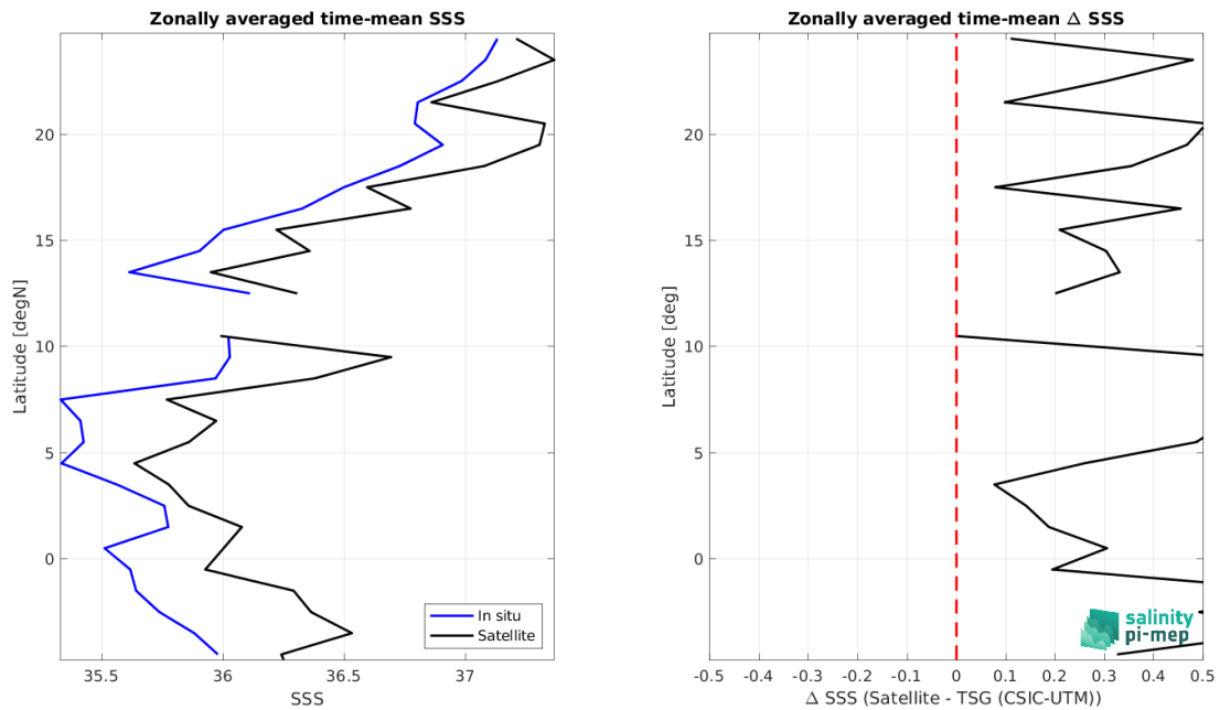
Figure 9: Left panel: Zonal mean SSS from SMAP SSS L2 v5.0 (JPL) satellite product (black) and from TSG (CSIC-UTM) (blue). Right panel: Zonal mean of \Delta SSS (Satellite - TSG (CSIC-UTM)) for all the collected Pi-MEP match-up pairs estimated over the full satellite product period.
