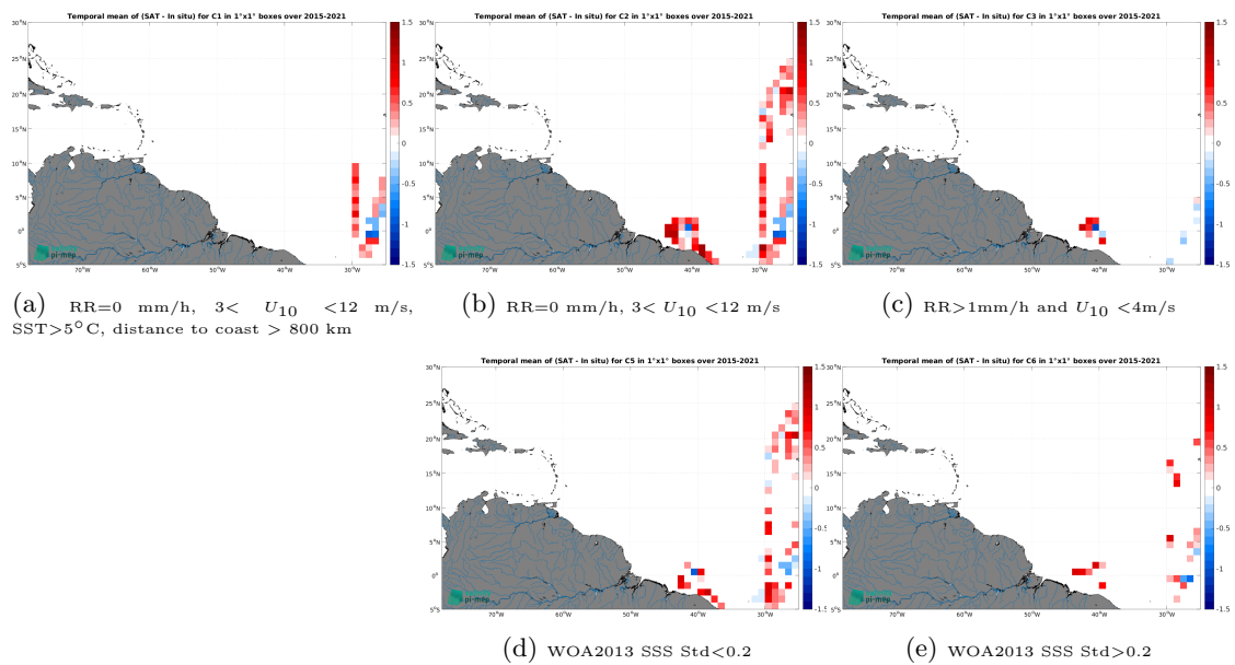
Figure 14: Temporal mean gridded over spatial boxes of size 1^\circ \times 1^\circ of \Delta SSS (SMAP SSS L2 v5.0 (JPL) - TSG (CSIC-UTM)) for 5 different subdatasets corresponding to:RR=0 mm/h, 3 < U_{10} < 12 m/s, SST >5^\circ\text{C} , distance to coast > 800 km (a), RR=0 mm/h, 3 < U_{10} < 12 m/s (b), RR >1 mm/h and U_{10} < 4 m/s (c), WOA2013 SSS Std <0.2 (d), WOA2013 SSS Std >0.2 (e).
