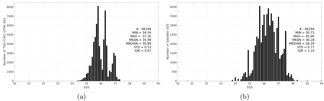
Figure 3: Histograms of SSS from TSG (CSIC-UTM) (a) and SMAP SSS L2 v5.0 (JPL) (b) considering all match-up pairs per bins of 0.1 over the Amazon and Orinoco river plumes Pi-MEP region and for the full satellite product period.
