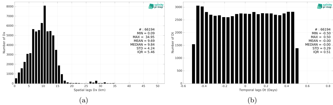
Figure 6: Histograms of the spatial (a) and temporal (b) lags between the location/time of the TSG (CSIC-UTM) measurement and the date of the corresponding SMAP SSS L2 v5.0 (JPL) SSS pixel.
