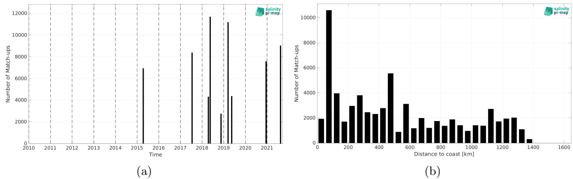
Figure 2: Number of match-ups between TSG (CSIC-UTM) and SMAP SSS L2 v5.0 (JPL) SSS as a function of time (a) and as function of the distance to coast (b) over the Amazon and Orinoco river plumes Pi-MEP region and for the full satellite product period.
