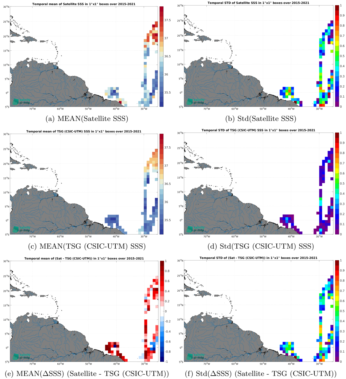
Figure 7: Temporal mean (left) and Std (right) of SSS from SMAP SSS L2 v5.0 (JPL) (top), TSG (CSIC-UTM) (middle), and of \Delta SSS (Satellite - TSG (CSIC-UTM)). Only match-up pairs are used to generate these maps.
