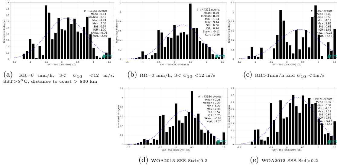
Figure 15: Normalized histogram of \Delta SSS (SMAP SSS L2 v5.0 (JPL) - TSG (CSIC-UTM)) for 5 different subdatasets corresponding to: RR=0 mm/h, 3 < U_{10} < 12 m/s, SST>5°C, distance to coast > 800 km (a), RR=0 mm/h, 3 < U_{10} < 12 m/s (b), RR>1mm/h and U_{10} < 4 m/s (c), WOA2013 SSS Std<0.2 (d), WOA2013 SSS Std>0.2 (e).
