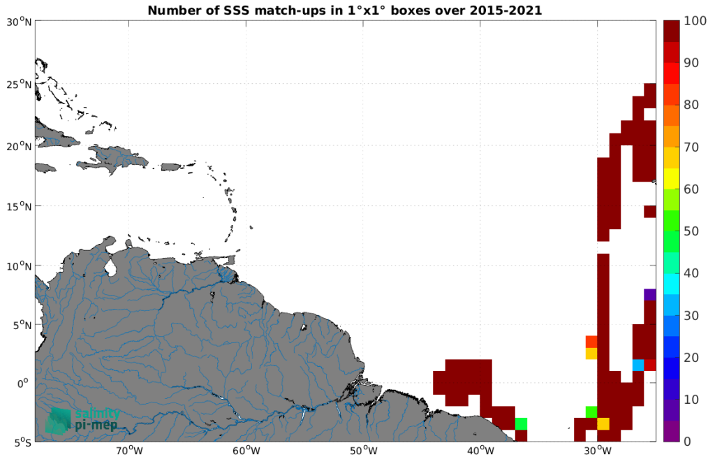
Figure 5: Number of SSS match-ups between TSG (CSIC-UTM) SSS and the SMAP SSS L2 v5.0 (JPL) SSS product for the Amazon and Orinoco river plumes Pi-MEP region over 1°x1° boxes and for the full satellite product period.
