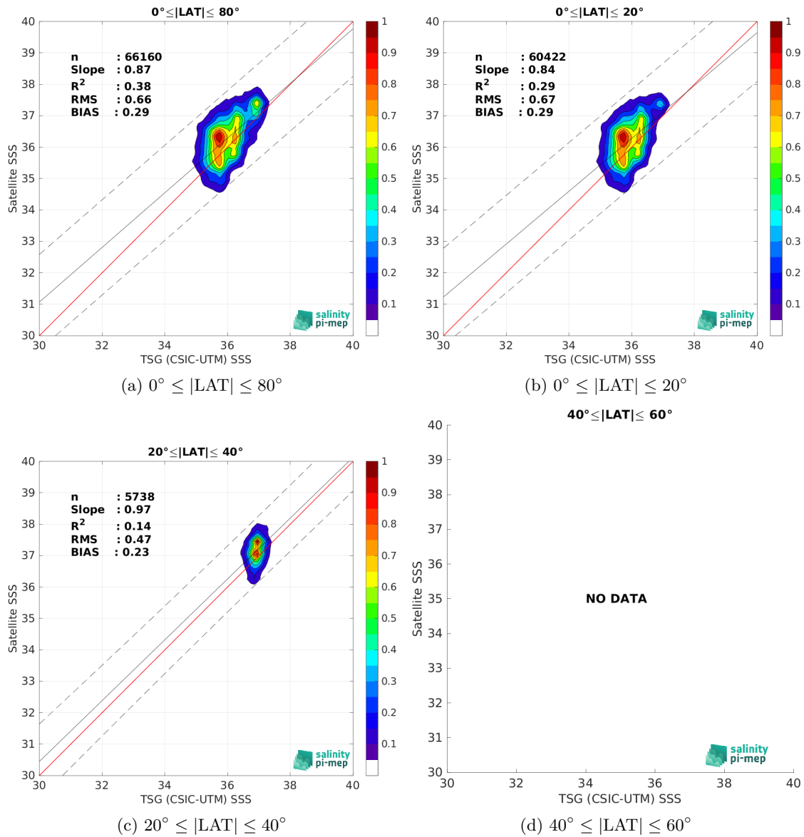
Figure 10: Contour maps of the concentration of SMAP SSS L2 v5.0 (JPL) SSS (y-axis) versus TSG (CSIC-UTM) SSS (x-axis) at match-up pairs for different latitude bands. For each plot, the red line shows x=y . The black thin and dashed lines indicate a linear fit through the data cloud and the \pm 95\% confidence levels, respectively. The number match-up pairs n , the slope and R^2 coefficient of the linear fit, the root mean square (RMS) and the mean bias between satellite and in situ data are indicated for each latitude band in each plots.
