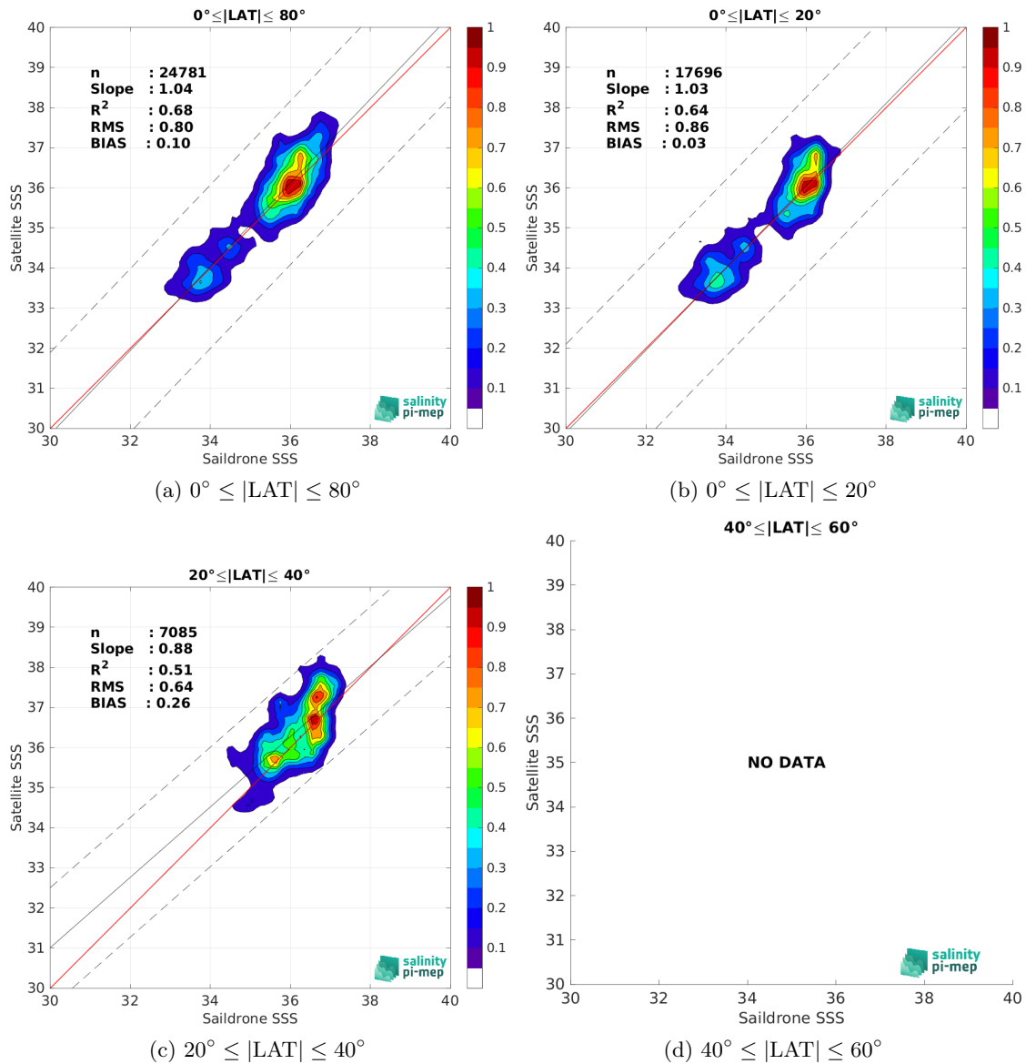
Figure 10: Contour maps of the concentration of SMAP SSS L2 v5.0 (JPL) SSS (y-axis) versus Sailldrone SSS (x-axis) at match-up pairs for different latitude bands. For each plot, the red line shows x=y . The black thin and dashed lines indicate a linear fit through the data cloud and the \pm 95\% confidence levels, respectively. The number match-up pairs n , the slope and R^2 coefficient of the linear fit, the root mean square (RMS) and the mean bias between satellite and in situ data are indicated for each latitude band in each plots.
