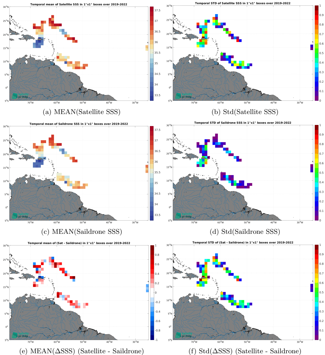
Figure 7: Temporal mean (left) and Std (right) of SSS from SMAP SSS L2 v5.0 (JPL) (top), Saildrone (middle), and of \Delta SSS (Satellite - Saildrone). Only match-up pairs are used to generate these maps.
