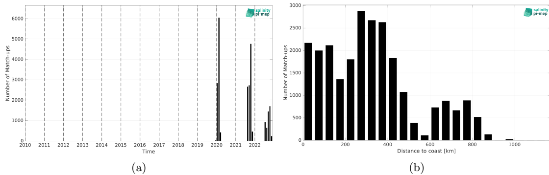
Figure 2: Number of match-ups between Saildrone and SMAP SSS L2 v5.0 (JPL) SSS as a function of time (a) and as function of the distance to coast (b) over the Amazon and Orinoco river plumes Pi-MEP region and for the full satellite product period.
