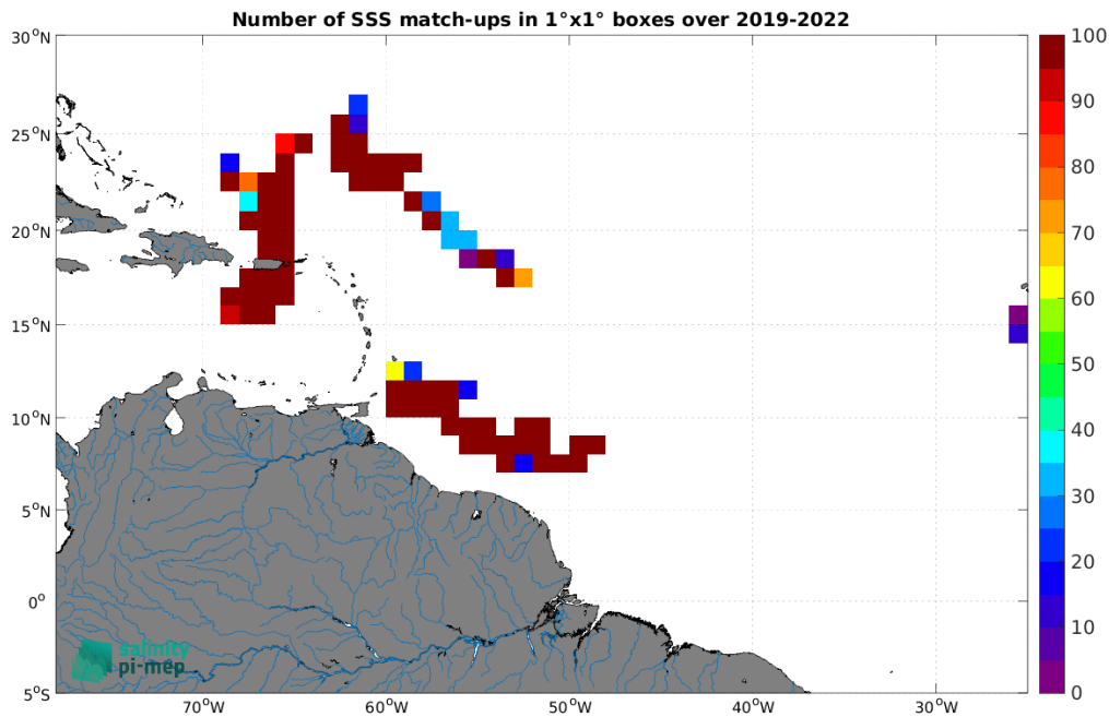
Figure 5: Number of SSS match-ups between Saildrone SSS and the SMAP SSS L2 v5.0 (JPL) SSS product for the Amazon and Orinoco river plumes Pi-MEP region over 1^\circ \times 1^\circ boxes and for the full satellite product period.
