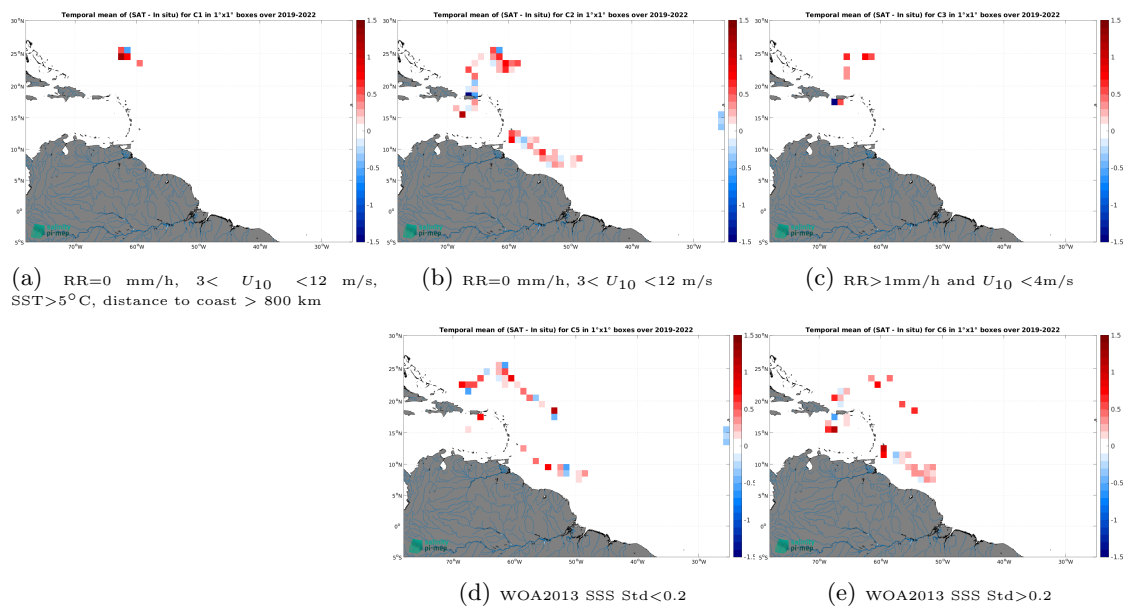
Figure 14: Temporal mean gridded over spatial boxes of size 1^\circ \times 1^\circ of \Delta SSS (SMAP SSS L2 v5.0 (JPL) - Saldrone) for 5 different subdatasets corresponding to:RR=0 mm/h, 3 < U_{10} < 12 m/s, SST >5^\circ\text{C} , distance to coast > 800 km (a), RR=0 mm/h, 3 < U_{10} < 12 m/s (b), RR >1 mm/h and U_{10} < 4 m/s (c), WOA2013 SSS Std <0.2 (d), WOA2013 SSS Std >0.2 (e).
