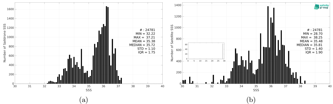
Figure 3: Histograms of SSS from Saildrone (a) and SMAP SSS L2 v5.0 (JPL) (b) considering all match-up pairs per bins of 0.1 over the Amazon and Orinoco river plumes Pi-MEP region and for the full satellite product period.
