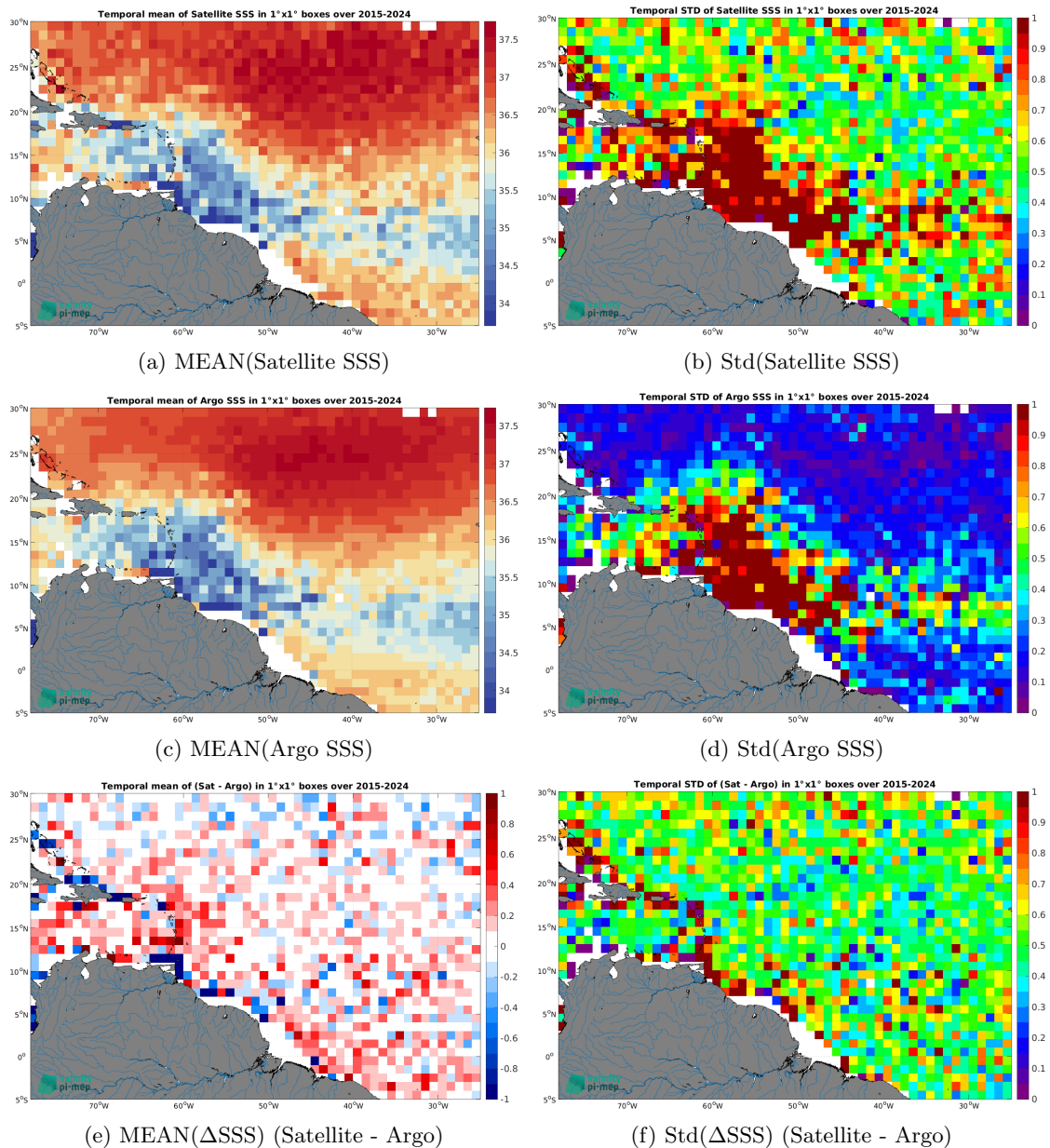
Figure 7: Temporal mean (left) and Std (right) of SSS from SMAP SSS L2 v5.0 (JPL) (top), Argo (middle), and of \Delta SSS (Satellite - Argo). Only match-up pairs are used to generate these maps.
