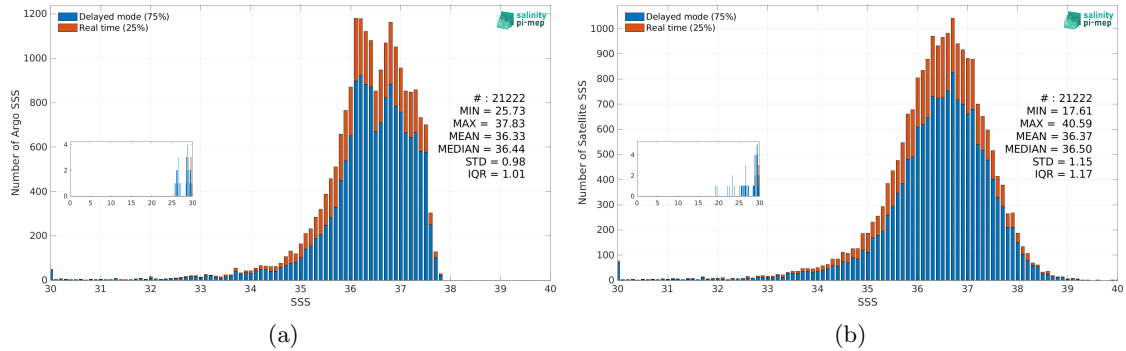
Figure 3: Histograms of SSS from Argo (a) and SMAP SSS L2 v5.0 (JPL) (b) considering all match-up pairs per bins of 0.1 over the Amazon and Orinoco river plumes Pi-MEP region and for the full satellite product period.
