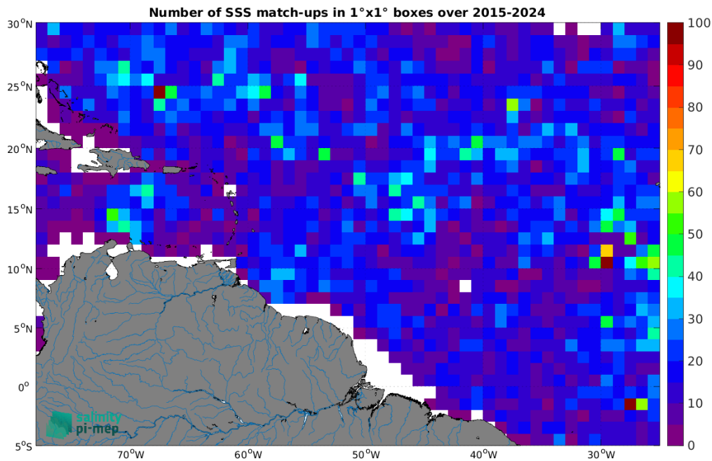
Figure 5: Number of SSS match-ups between Argo SSS and the SMAP SSS L2 v5.0 (JPL) SSS product for the Amazon and Orinoco river plumes Pi-MEP region over 1^\circ \times 1^\circ boxes and for the full satellite product period.
