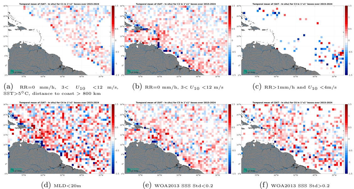
Figure 14: Temporal mean gridded over spatial boxes of size 1^\circ \times 1^\circ of \Delta SSS (SMAP SSS L2 v5.0 (JPL) - Argo) for 6 different subdatasets corresponding to: RR=0 mm/h, 3 < U_{10} < 12 m/s, SST > 5°C, distance to coast > 800 km (a), RR=0 mm/h, 3 < U_{10} < 12 m/s (b), RR > 1mm/h and U_{10} < 4 m/s (c), MLD < 20m (d), WOA2013 SSS Std < 0.2 (e), WOA2013 SSS Std > 0.2 (f).
