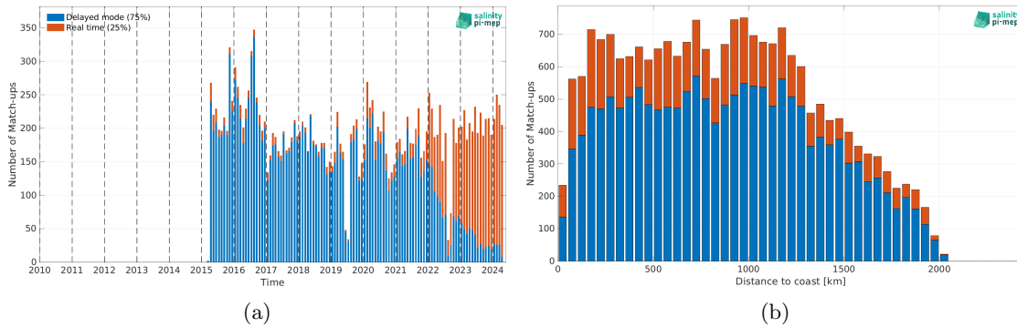
Figure 2: Number of match-ups between Argo and SMAP SSS L2 v5.0 (JPL) SSS as a function of time (a) and as function of the distance to coast (b) over the Amazon and Orinoco river plumes Pi-MEP region and for the full satellite product period.
