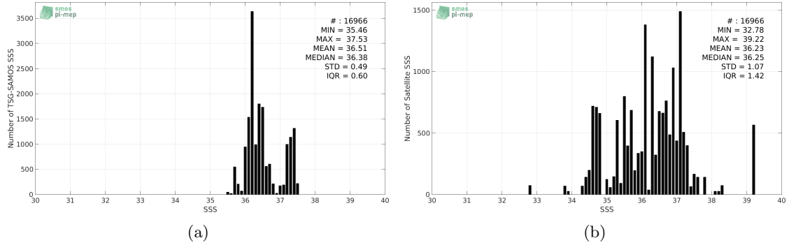
Figure 2: Histograms of SSS from TSG-SAMOS (a) and SMAP-L2-JPL-V4 (b) considering all match-up pairs per bins of 0.1 over the Amazon and Orinoco river plumes Pi-MEP region and for the full satellite product period.
