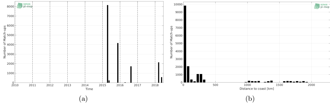
Figure 1: Number of match-ups between TSG-SAMOS and SMAP-L2-JPL-V4 SSS as a function of time (a) and as function of the distance to coast (b) over the Amazon and Orinoco river plumes Pi-MEP region and for the full satellite product period.
