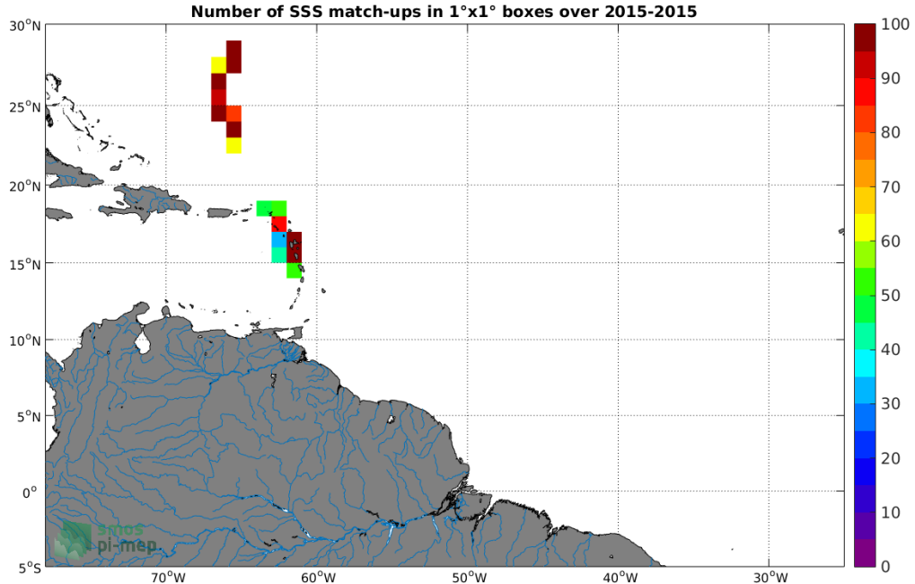
Figure 4: Number of SSS match-ups between TSG-GOSUD-Sailing-ship SSS and the SMAP-L2-JPL-V4 SSS product for the Amazon and Orinoco river plumes Pi-MEP region over 1^\circ \times 1^\circ boxes and for the full satellite product period.
