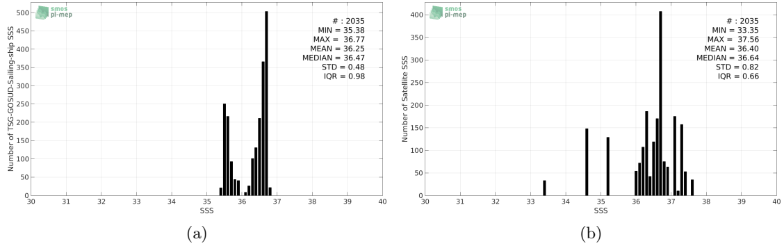
Figure 2: Histograms of SSS from TSG-GOSUD-Sailing-ship (a) and SMAP-L2-JPL-V4 (b) considering all match-up pairs per bins of 0.1 over the Amazon and Orinoco river plumes Pi-MEP region and for the full satellite product period.
