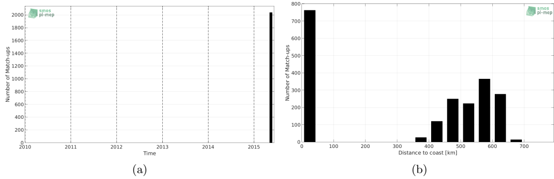
Figure 1: Number of match-ups between TSG-GOSUD-Sailing-ship and SMAP-L2-JPL-V4 SSS as a function of time (a) and as function of the distance to coast (b) over the Amazon and Orinoco river plumes Pi-MEP region and for the full satellite product period.
