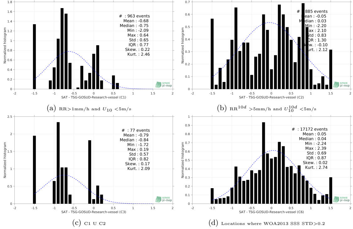
Figure 13: Normalized histogram of \Delta SSS (SMAP-L2-JPL-V4 - TSG-GOSUD-Research-vessel) for 6 different subdatasets corresponding to: RR > 1mm/h and U_{10} < 5\text{m/s} (a), RR^{10d} > 5\text{mm/h} and U_{10}^{10d} < 5\text{m/s} (b), C1 U C2 (c), Locations where WOA2013 SSS STD > 0.2 (d).
