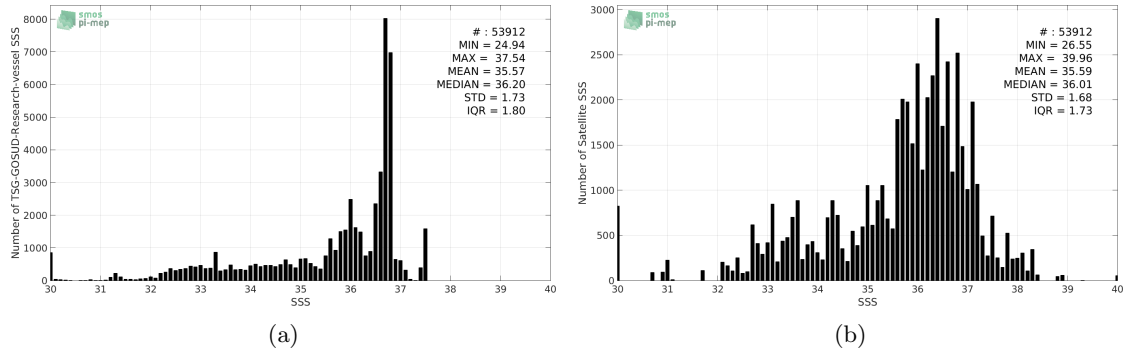
Figure 2: Histograms of SSS from TSG-GOSUD-Research-vessel (a) and SMAP-L2-JPL-V4 (b) considering all match-up pairs per bins of 0.1 over the Amazon and Orinoco river plumes Pi-MEP region and for the full satellite product period.
