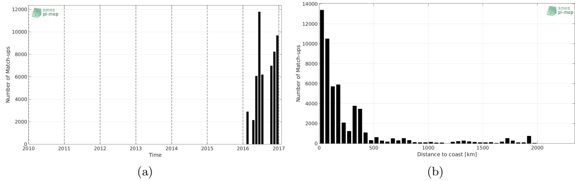
Figure 1: Number of match-ups between TSG-GOSUD-Research-vessel and SMAP-L2-JPL-V4 SSS as a function of time (a) and as function of the distance to coast (b) over the Amazon and Orinoco river plumes Pi-MEP region and for the full satellite product period.
