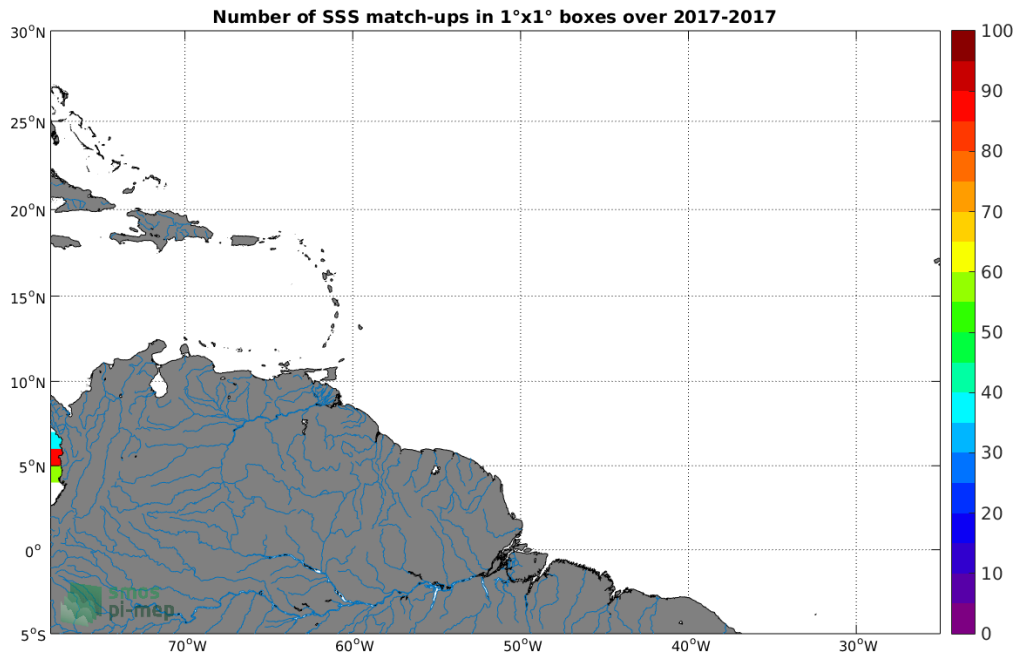
Figure 3: Number of SSS match-ups between Surface drifters SSS and the SMAP-L2-JPL-V4 SSS product for the Amazon and Orinoco river plumes Pi-MEP region over 1°x1° boxes and for the full satellite product period.
