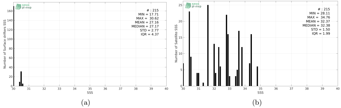
Figure 2: Histograms of SSS from Surface drifters (a) and SMAP-L2-JPL-V4 (b) considering all match-up pairs per bins of 0.1 over the Amazon and Orinoco river plumes Pi-MEP region and for the full satellite product period.
