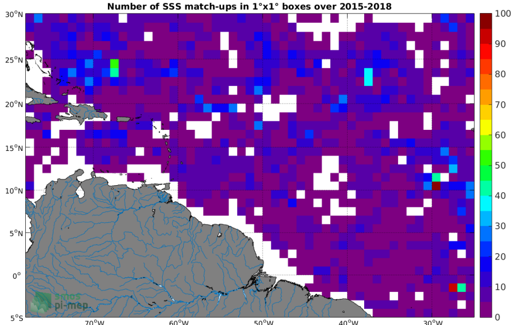
Figure 4: Number of SSS match-ups between Argo SSS and the SMAP-L2-JPL-V4 SSS product for the Amazon and Orinoco river plumes Pi-MEP region over 1^\circ \times 1^\circ boxes and for the full satellite product period.
