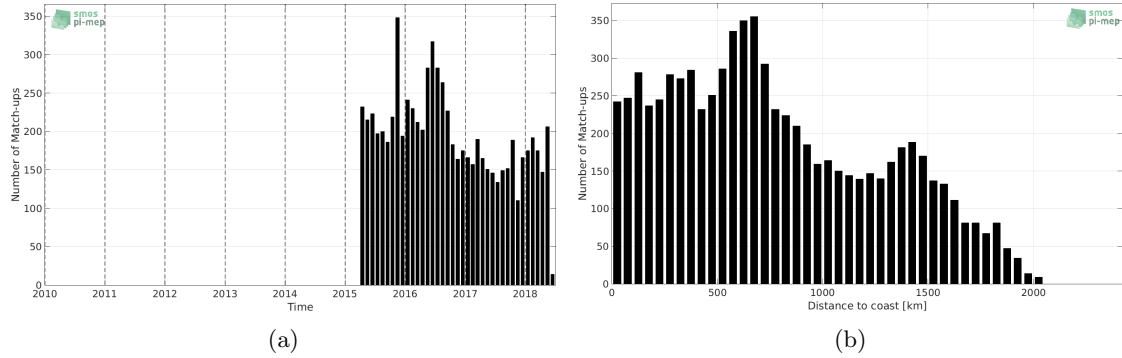
Figure 1: Number of match-ups between Argo and SMAP-L2-JPL-V4 SSS as a function of time (a) and as function of the distance to coast (b) over the Amazon and Orinoco river plumes Pi-MEP region and for the full satellite product period.
