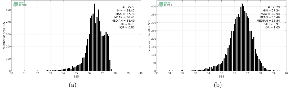
Figure 2: Histograms of SSS from Argo (a) and SMAP-L2-JPL-V4 (b) considering all match-up pairs per bins of 0.1 over the Amazon and Orinoco river plumes Pi-MEP region and for the full satellite product period.
