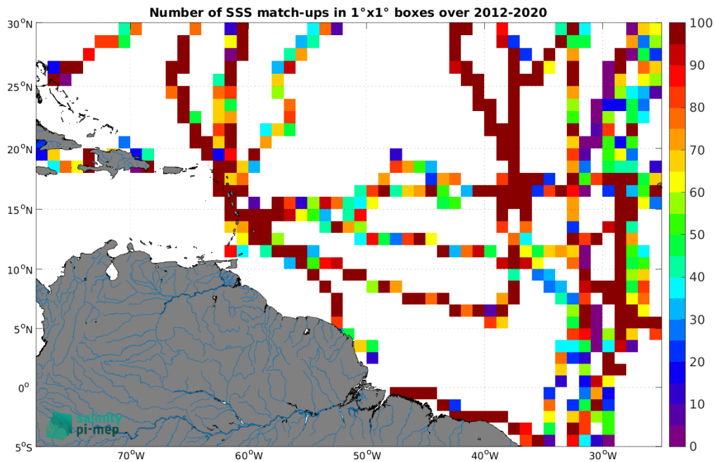
Figure 5: Number of SSS match-ups between TSG (GOSUD-Sailing-ship) SSS and the ISAS SSS product for the Amazon and Orinoco river plumes Pi-MEP region over 1^{\circ} \times 1^{\circ} boxes and for the full satellite product period.
