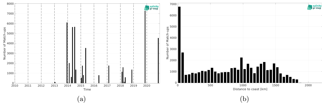
Figure 2: Number of match-ups between TSG (GOSUD-Sailing-ship) and ISAS SSS as a function of time (a) and as function of the distance to coast (b) over the Amazon and Orinoco river plumes Pi-MEP region and for the full satellite product period.
