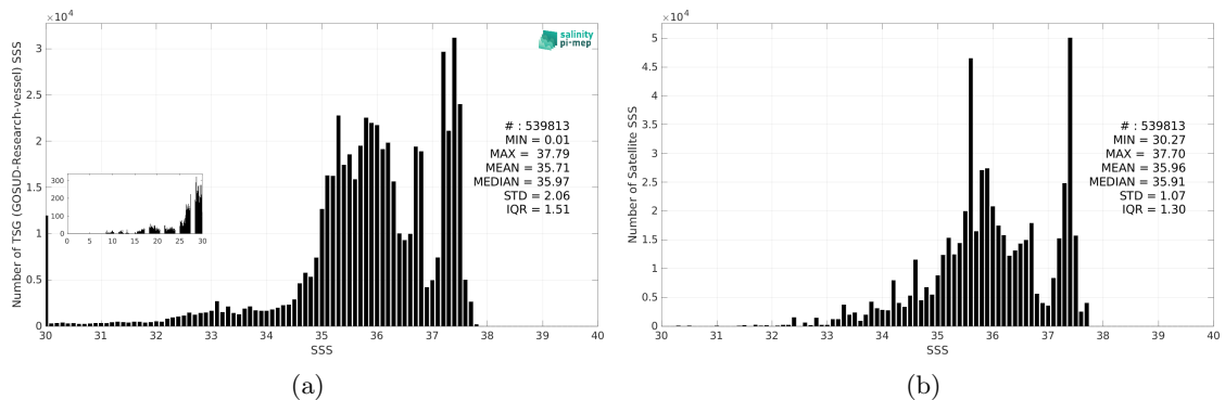
Figure 3: Histograms of SSS from TSG (GOSUD-Research-vessel) (a) and ISAS v7 - Monthly (Ifremer-LOPS-CMEMS) (b) considering all match-up pairs per bins of 0.1 over the Amazon and Orinoco river plumes Pi-MEP region and for the full satellite product period.
