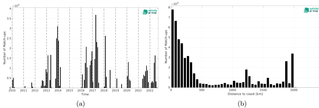
Figure 2: Number of match-ups between TSG (GOSUD-Research-vessel) and ISAS v7 - Monthly (Ifremer-LOPS-CMEMS) SSS as a function of time (a) and as function of the distance to coast (b) over the Amazon and Orinoco river plumes Pi-MEP region and for the full satellite product period.
