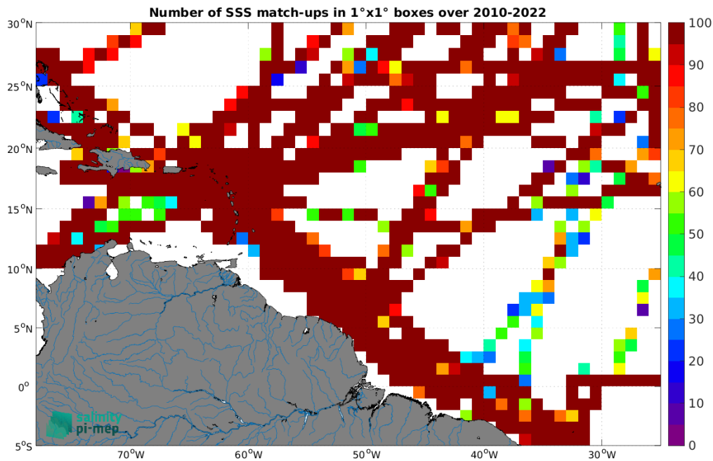
Figure 5: Number of SSS match-ups between TSG (GOSUD-Research-vessel) SSS and the ISAS v7 - Monthly (Ifremer-LOPS-CMEMS) SSS product for the Amazon and Orinoco river plumes Pi-MEP region over 1^\circ \times 1^\circ boxes and for the full satellite product period.
