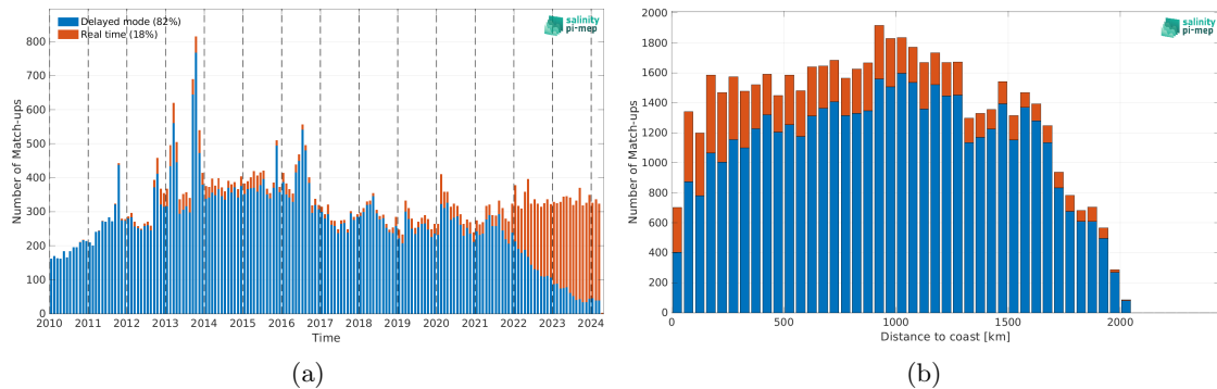
Figure 2: Number of match-ups between Argo and ISAS SSS as a function of time (a) and as function of the distance to coast (b) over the Amazon and Orinoco river plumes Pi-MEP region and for the full satellite product period.
