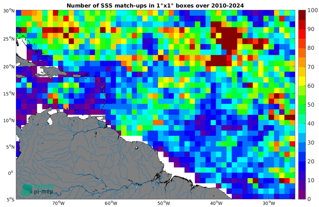
Figure 5: Number of SSS match-ups between Argo SSS and the ISAS SSS product for the Amazon and Orinoco river plumes Pi-MEP region over 1^\circ \times 1^\circ boxes and for the full satellite product period.
