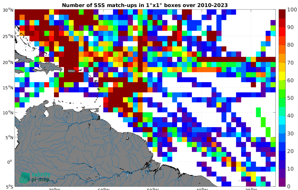
Figure 5: Number of SSS match-ups between TSG (SAMOS) SSS and the CCI SSS L4 Merged-OI v5.5 - 7-day running (ESA) SSS product for the Amazon and Orinoco river plumes Pi-MEP region over 1^\circ \times 1^\circ boxes and for the full satellite product period.
