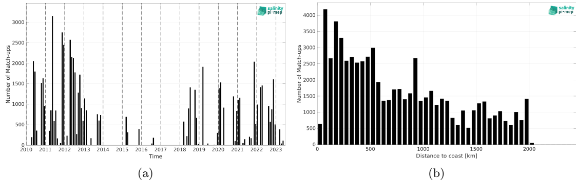
Figure 2: Number of match-ups between TSG (SAMOS) and CCI SSS L4 Merged-OI v5.5 - 7-day running (ESA) SSS as a function of time (a) and as function of the distance to coast (b) over the Amazon and Orinoco river plumes Pi-MEP region and for the full satellite product period.
