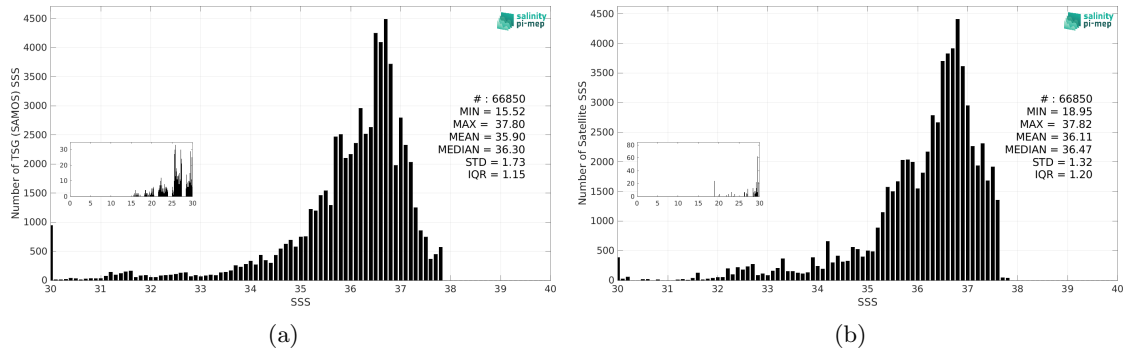
Figure 3: Histograms of SSS from TSG (SAMOS) (a) and CCI SSS L4 Merged-OI v5.5 - 7-day running (ESA) (b) considering all match-up pairs per bins of 0.1 over the Amazon and Orinoco river plumes Pi-MEP region and for the full satellite product period.
