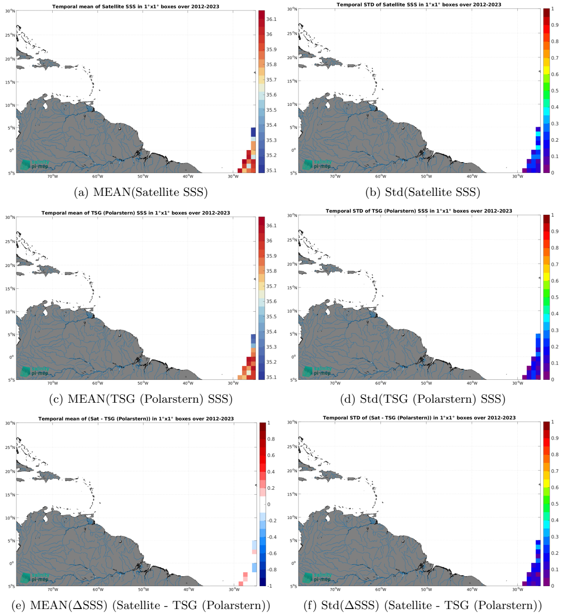
Figure 7: Temporal mean (left) and Std (right) of SSS from CCI SSS L4 Merged-OI v5.5 - 7-day running (ESA) (top), TSG (Polarstern) (middle), and of \Delta SSS (Satellite - TSG (Polarstern)). Only match-up pairs are used to generate these maps.
