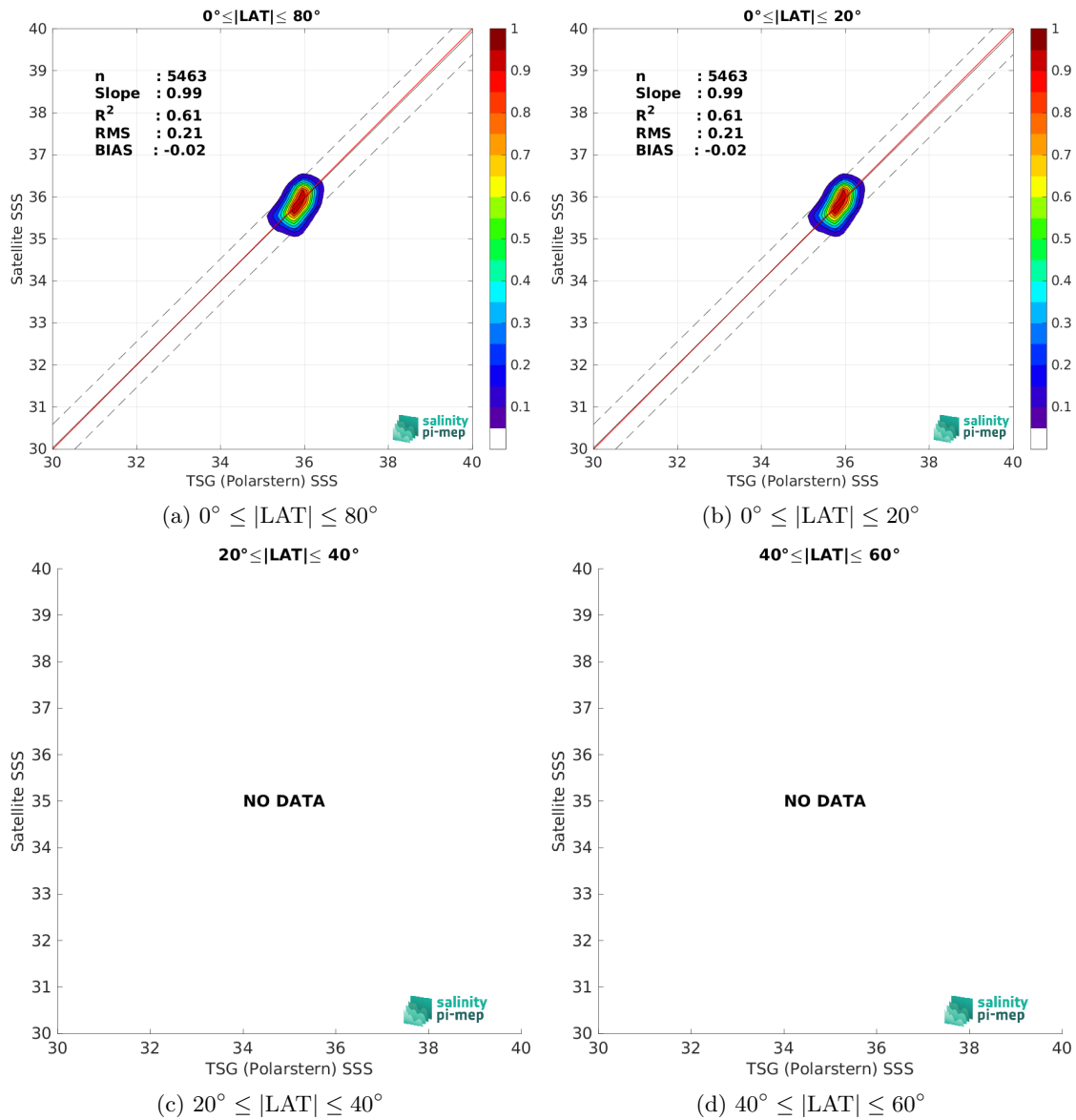
Figure 10: Contour maps of the concentration of CCI SSS L4 Merged-OI v5.5 - 7-day running (ESA) SSS (y-axis) versus TSG (Polarstern) SSS (x-axis) at match-up pairs for different latitude bands. For each plot, the red line shows x=y . The black thin and dashed lines indicate a linear fit through the data cloud and the \pm 95\% confidence levels, respectively. The number match-up pairs n , the slope and R^2 coefficient of the linear fit, the root mean square (RMS) and the mean bias between satellite and in situ data are indicated for each latitude band in each plots.
