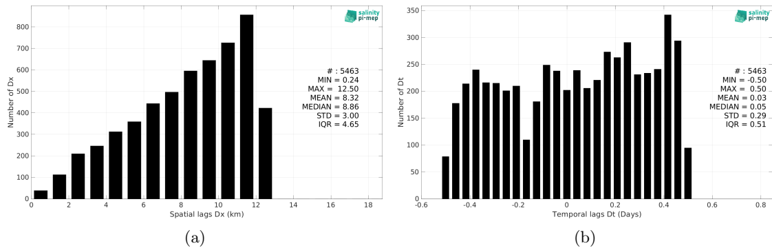
Figure 6: Histograms of the spatial (a) and temporal (b) lags between the location/time of the TSG (Polarstern) measurement and the date of the corresponding CCI SSS L4 Merged-OI v5.5 - 7-day running (ESA) SSS pixel.
