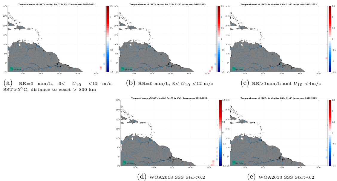
Figure 14: Temporal mean gridded over spatial boxes of size 1^\circ \times 1^\circ of \Delta SSS (CCI SSS L4 Merged-OI v5.5 - 7-day running (ESA) - TSG (Polarstern)) for 5 different subdatasets corresponding to:RR=0 mm/h, 3 < U_{10} < 12 m/s, SST >5^\circ C, distance to coast > 800 km (a), RR=0 mm/h, 3 < U_{10} < 12 m/s (b), RR >1 mm/h and U_{10} < 4 m/s (c), WOA2013 SSS Std <0.2 (d), WOA2013 SSS Std >0.2 (e).
