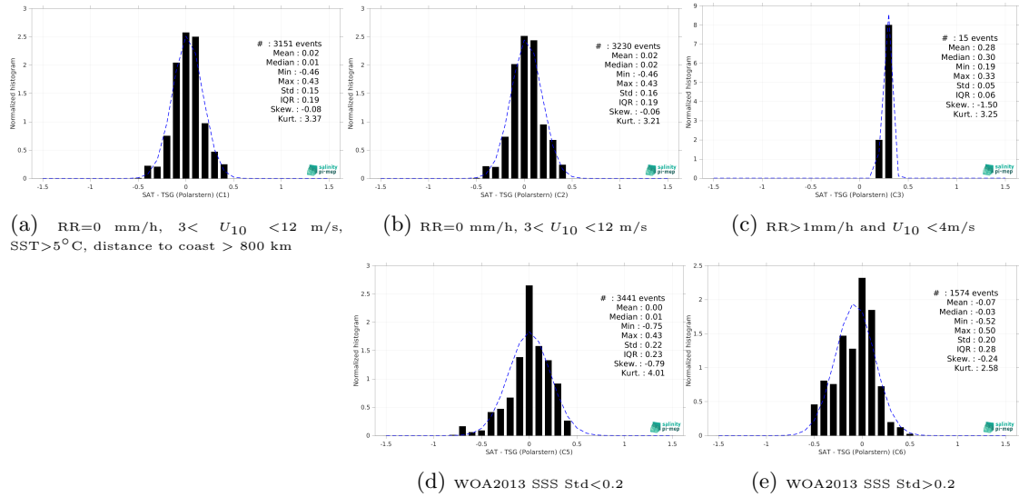
Figure 15: Normalized histogram of \Delta SSS (CCI SSS L4 Merged-OI v5.5 - 7-day running (ESA) - TSG (Polarstern)) for 5 different subdatasets corresponding to: RR=0 mm/h, 3 < U_{10} < 12 m/s, SST > 5°C, distance to coast > 800 km (a), RR=0 mm/h, 3 < U_{10} < 12 m/s (b), RR > 1mm/h and U_{10} < 4 m/s (c), WOA2013 SSS Std < 0.2 (d), WOA2013 SSS Std > 0.2 (e).
