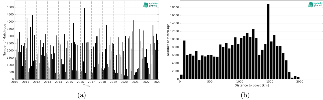
Figure 2: Number of match-ups between TSG (LEGOS-DM) and CCI SSS L4 Merged-OI v5.5 - 7-day running (ESA) SSS as a function of time (a) and as function of the distance to coast (b) over the Amazon and Orinoco river plumes Pi-MEP region and for the full satellite product period.
