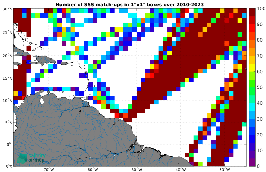
Figure 5: Number of SSS match-ups between TSG (LEGOS-DM) SSS and the CCI SSS L4 Merged-OI v5.5 - 7-day running (ESA) SSS product for the Amazon and Orinoco river plumes Pi-MEP region over 1^\circ \times 1^\circ boxes and for the full satellite product period.
