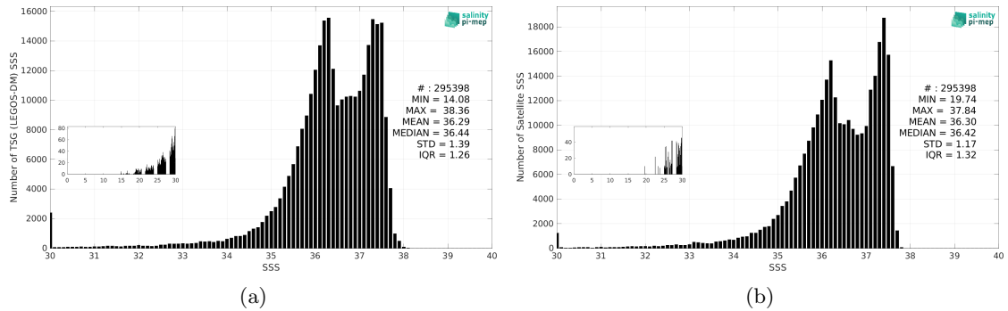
Figure 3: Histograms of SSS from TSG (LEGOS-DM) (a) and CCI SSS L4 Merged-OI v5.5 - 7-day running (ESA) (b) considering all match-up pairs per bins of 0.1 over the Amazon and Orinoco river plumes Pi-MEP region and for the full satellite product period.
