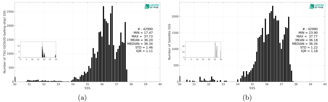
Figure 3: Histograms of SSS from TSG (GOSUD-Sailing-ship) (a) and CCI SSS L4 Merged-OI v5.5 - 7-day running (ESA) (b) considering all match-up pairs per bins of 0.1 over the Amazon and Orinoco river plumes Pi-MEP region and for the full satellite product period.
