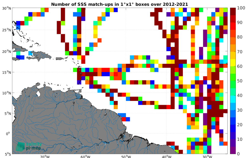
Figure 5: Number of SSS match-ups between TSG (GOSUD-Sailing-ship) SSS and the CCI SSS L4 Merged-OI v5.5 - 7-day running (ESA) SSS product for the Amazon and Orinoco river plumes Pi-MEP region over 1^\circ \times 1^\circ boxes and for the full satellite product period.
