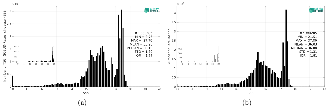
Figure 3: Histograms of SSS from TSG (GOSUD-Research-vessel) (a) and CCI SSS L4 Merged-OI v5.5 - 7-day running (ESA) (b) considering all match-up pairs per bins of 0.1 over the Amazon and Orinoco river plumes Pi-MEP region and for the full satellite product period.
