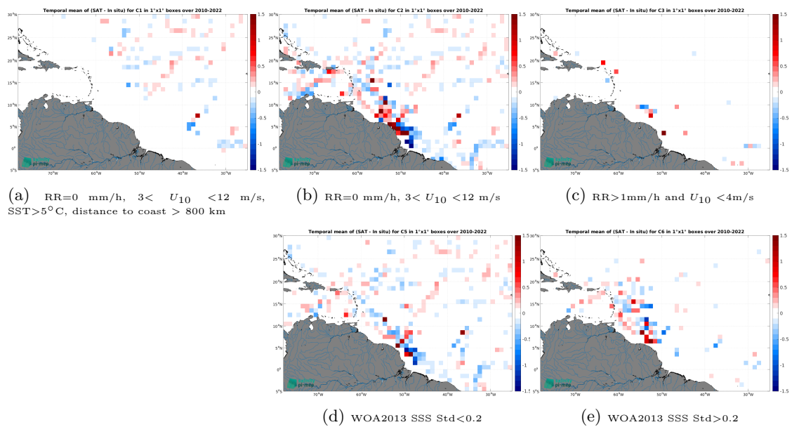
Figure 14: Temporal mean gridded over spatial boxes of size 1^\circ \times 1^\circ of \Delta\text{SSS} (CCI SSS L4 Merged-OI v5.5 - 7-day running (ESA) - TSG (GOSUD-Research-vessel)) for 5 different subdatasets corresponding to:RR=0 mm/h, 3 < U_{10} < 12 m/s, SST >5^\circ\text{C} , distance to coast > 800 km (a), RR=0 mm/h, 3 < U_{10} < 12 m/s (b), RR >1 mm/h and U_{10} < 4 m/s (c), WOA2013 SSS Std <0.2 (d), WOA2013 SSS Std >0.2 (e).
