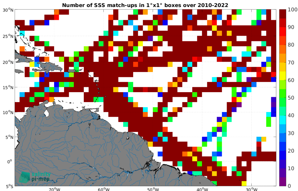
Figure 5: Number of SSS match-ups between TSG (GOSUD-Research-vessel) SSS and the CCI SSS L4 Merged-OI v5.5 - 7-day running (ESA) SSS product for the Amazon and Orinoco river plumes Pi-MEP region over 1^\circ \times 1^\circ boxes and for the full satellite product period.
