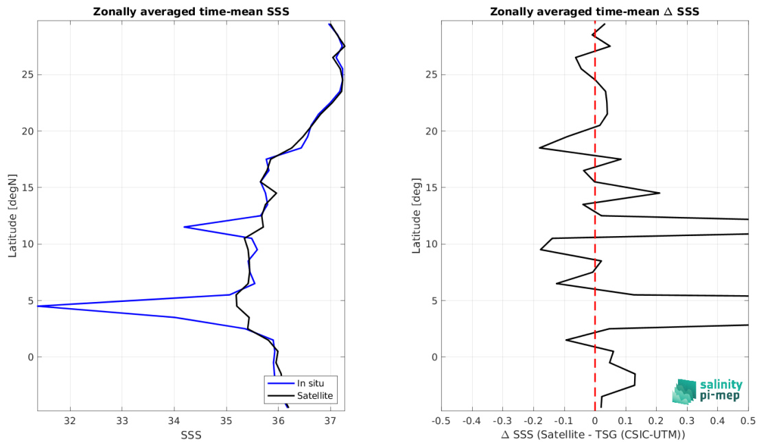
Figure 9: Left panel: Zonal mean SSS from CCI SSS L4 Merged-OI v5.5 - 7-day running (ESA) satellite product (black) and from TSG (CSIC-UTM) (blue). Right panel: Zonal mean of \Delta SSS (Satellite - TSG (CSIC-UTM)) for all the collected Pi-MEP match-up pairs estimated over the full satellite product period.
