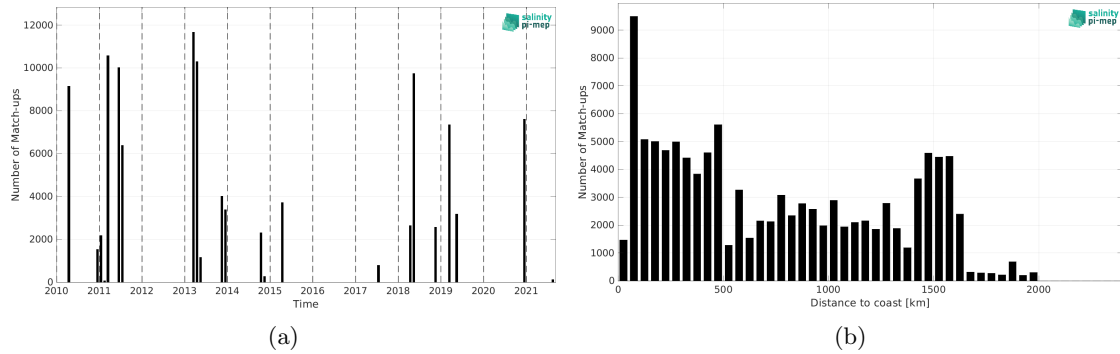
Figure 2: Number of match-ups between TSG (CSIC-UTM) and CCI SSS L4 Merged-OI v5.5 - 7-day running (ESA) SSS as a function of time (a) and as function of the distance to coast (b) over the Amazon and Orinoco river plumes Pi-MEP region and for the full satellite product period.
