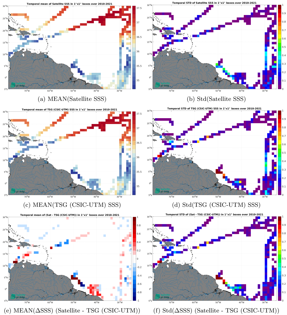
Figure 7: Temporal mean (left) and Std (right) of SSS from CCI SSS L4 Merged-OI v5.5 - 7-day running (ESA) (top), TSG (CSIC-UTM) (middle), and of \Delta SSS (Satellite - TSG (CSIC-UTM)). Only match-up pairs are used to generate these maps.
