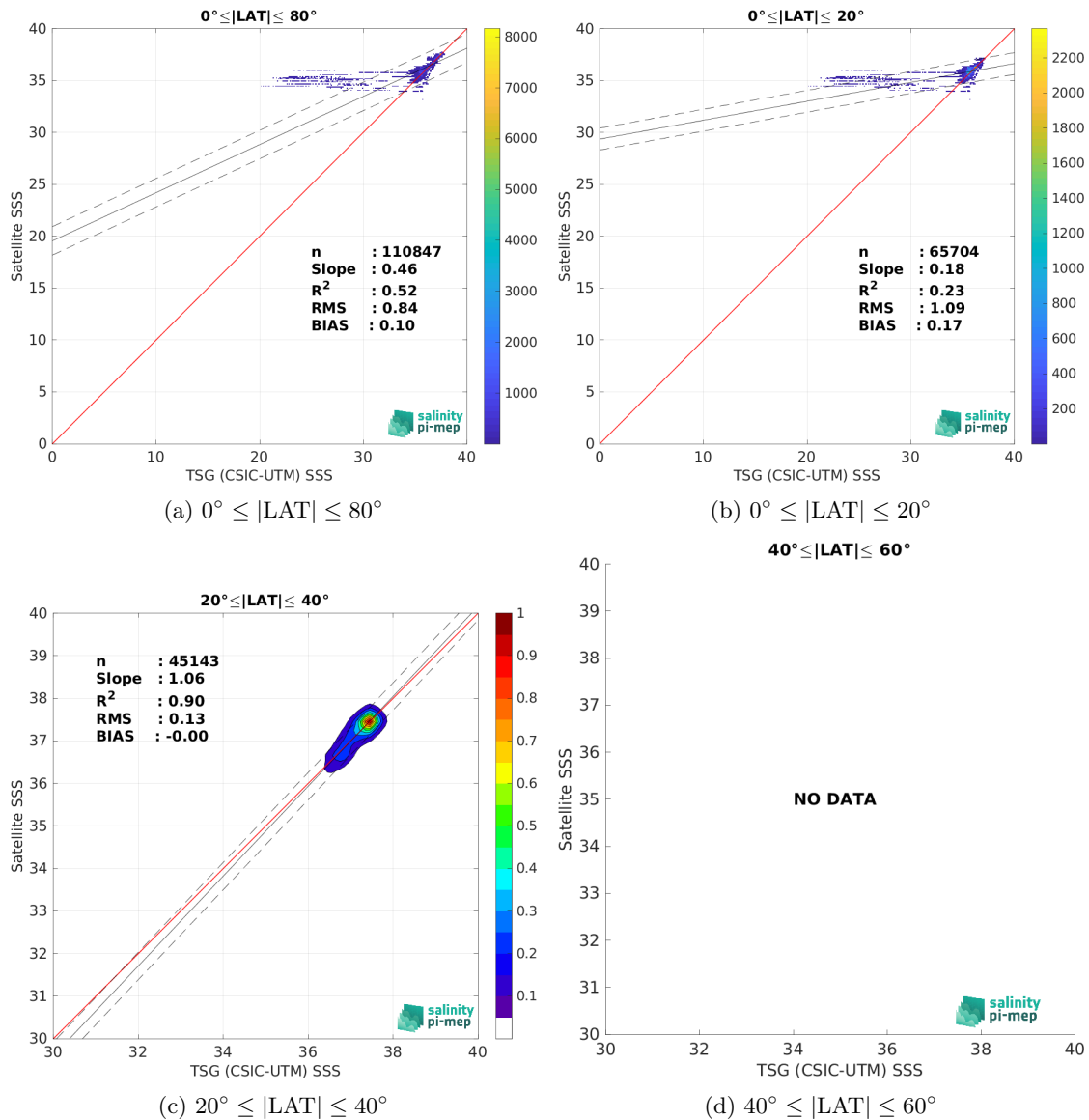
Figure 10: Contour maps of the concentration of CCI SSS L4 Merged-OI v5.5 - 7-day running (ESA) SSS (y-axis) versus TSG (CSIC-UTM) SSS (x-axis) at match-up pairs for different latitude bands. For each plot, the red line shows x=y . The black thin and dashed lines indicate a linear fit through the data cloud and the \pm 95\% confidence levels, respectively. The number match-up pairs n , the slope and R^2 coefficient of the linear fit, the root mean square (RMS) and the mean bias between satellite and in situ data are indicated for each latitude band in each plots.
