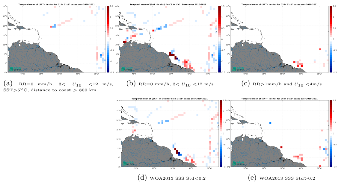
Figure 14: Temporal mean gridded over spatial boxes of size 1^\circ \times 1^\circ of \Delta\text{SSS} (CCI SSS L4 Merged-OI v5.5 - 7-day running (ESA) - TSG (CSIC-UTM)) for 5 different subdatasets corresponding to:RR=0 mm/h, 3 < U_{10} < 12 m/s, SST >5^\circ\text{C} , distance to coast > 800 km (a), RR=0 mm/h, 3 < U_{10} < 12 m/s (b), RR >1 mm/h and U_{10} < 4 m/s (c), WOA2013 SSS Std <0.2 (d), WOA2013 SSS Std >0.2 (e).
