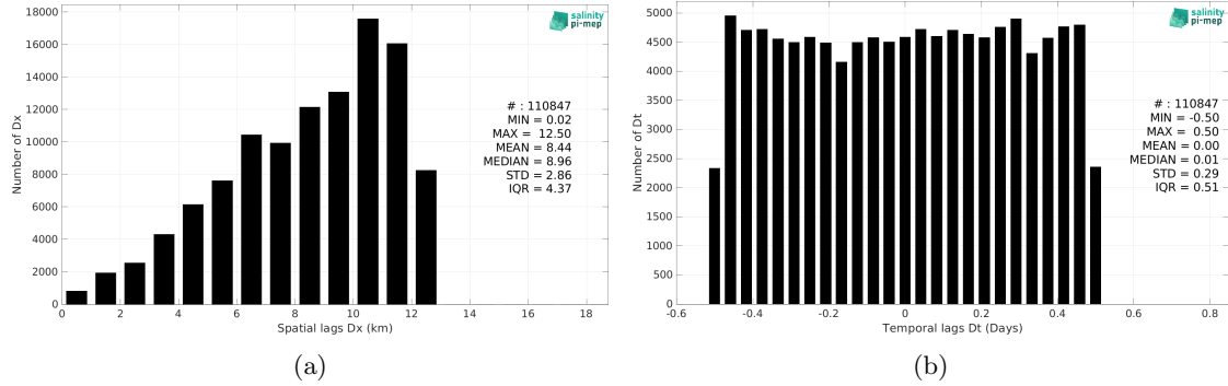
Figure 6: Histograms of the spatial (a) and temporal (b) lags between the location/time of the TSG (CSIC-UTM) measurement and the date of the corresponding CCI SSS L4 Merged-OI v5.5 - 7-day running (ESA) SSS pixel.
