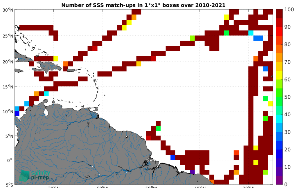
Figure 5: Number of SSS match-ups between TSG (CSIC-UTM) SSS and the CCI SSS L4 Merged-OI v5.5 - 7-day running (ESA) SSS product for the Amazon and Orinoco river plumes Pi-MEP region over 1^\circ \times 1^\circ boxes and for the full satellite product period.
