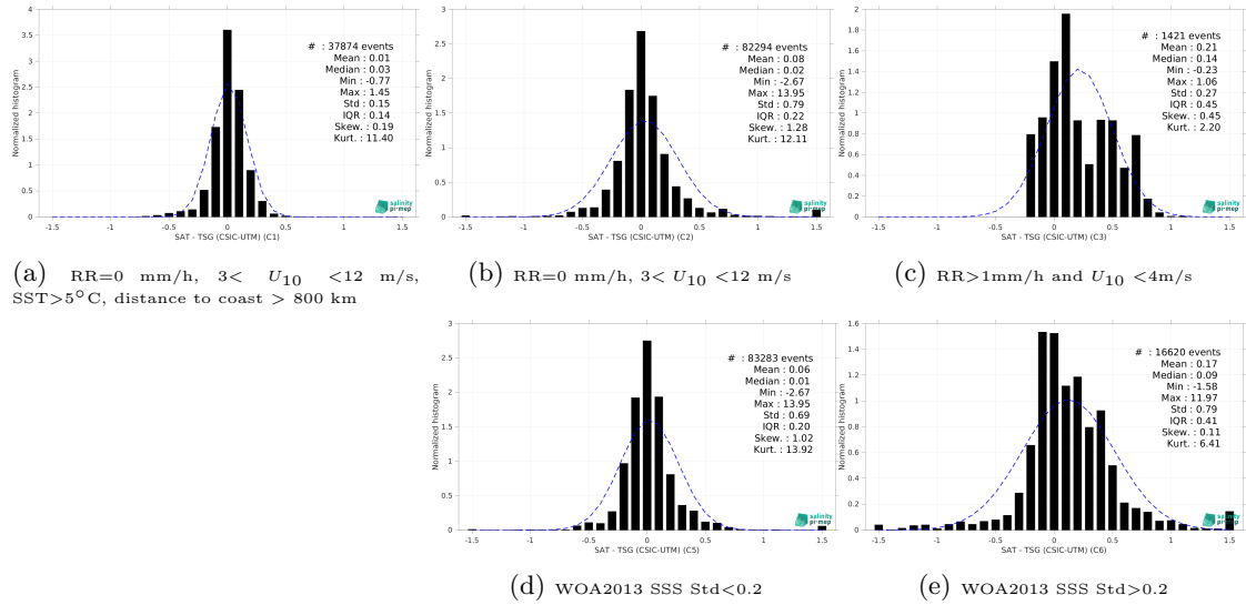
Figure 15: Normalized histogram of \Delta SSS (CCI SSS L4 Merged-OI v5.5 - 7-day running (ESA) - TSG (CSIC-UTM)) for 5 different subdatasets corresponding to: RR=0 mm/h, 3 < U_{10} < 12 m/s, SST>5°C, distance to coast > 800 km (a), RR=0 mm/h, 3 < U_{10} < 12 m/s (b), RR>1mm/h and U_{10} < 4 m/s (c), WOA2013 SSS Std<0.2 (d), WOA2013 SSS Std>0.2 (e).
