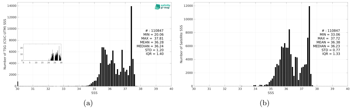
Figure 3: Histograms of SSS from TSG (CSIC-UTM) (a) and CCI SSS L4 Merged-OI v5.5 - 7-day running (ESA) (b) considering all match-up pairs per bins of 0.1 over the Amazon and Orinoco river plumes Pi-MEP region and for the full satellite product period.
